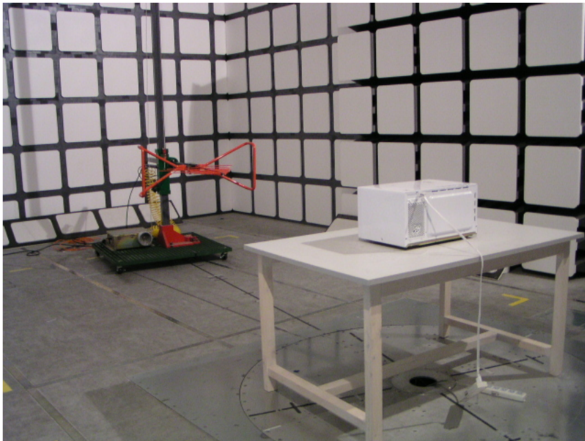
Radiated Emission (30MHz to 1000MHz) - Rear View
