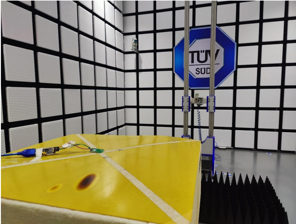
Spurious radiated emissions_Above 18000MHz
