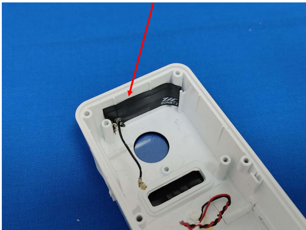
< 433.9MHz Antenna >
