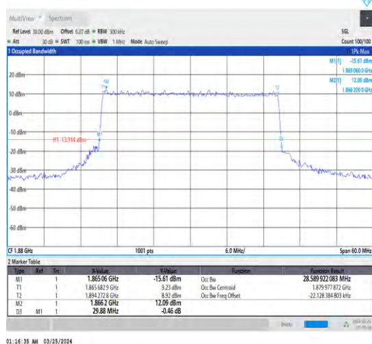
1-N2-15-30-M-7-CP-16QAM-Outer_Full-160@0-Ant1 -28.59-29.880-≤30-PASS
