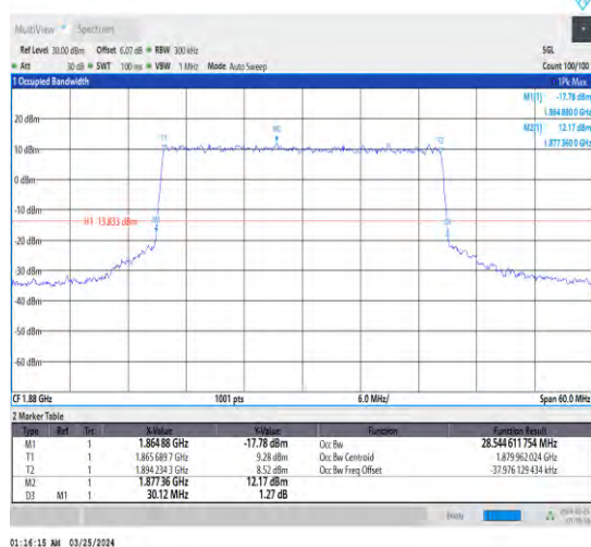
1-N2-15-30-M-6-CP-QPSK-Outer_Full-160@0-Ant1 28.545-30.120-≤30-PASS
