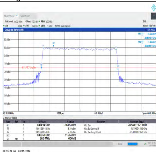
1-N2-15-30-M-5-DFT-256QAM-Outer_Full-160@0-A nt1-28.54-30.000-≤30-PASS
