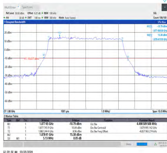
1-N2-15-5-M-4-DFT-64QAM-Outer_Full-25@0-Ant1-4. 4.499-5.130-≤5-PASS
