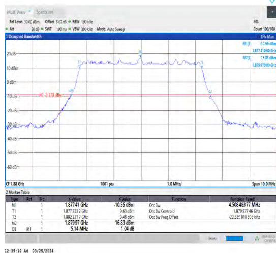
1-N2-15-5-M-3-DFT-16QAM-Outer_Full-25@0-Ant1-4. 4.508-5.140-≤5-PASS
