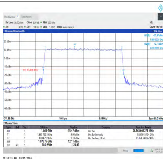
1-N2-15-30-M-4-DFT-64QAM-Outer_Full-160@0-Ant 1-28.564-30.000-≤30-PASS
