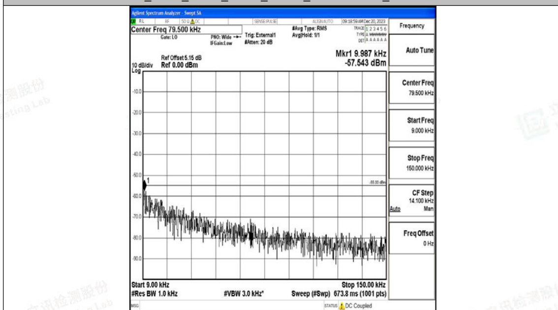
Band41_5MHz_16QAM_40620_1RB#0_0.009~0.15_0.009~0.15
