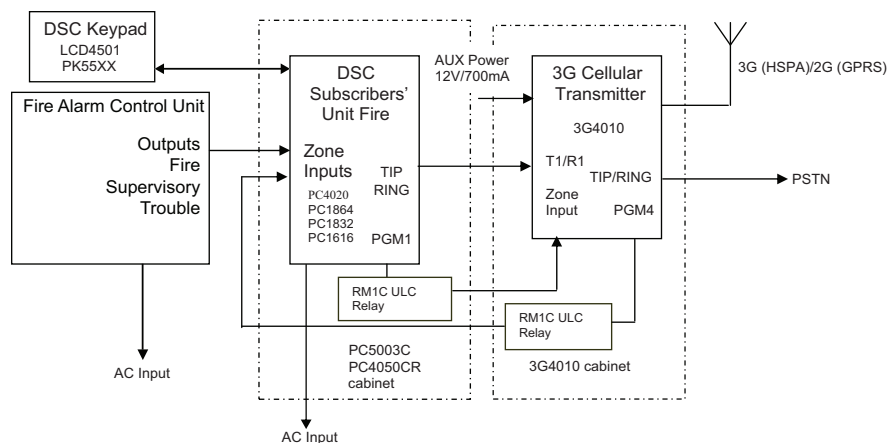
Figure 10-5 DSC Subscribers' Unit Fire and Cellular Transmitter Mounted in the Same Room
