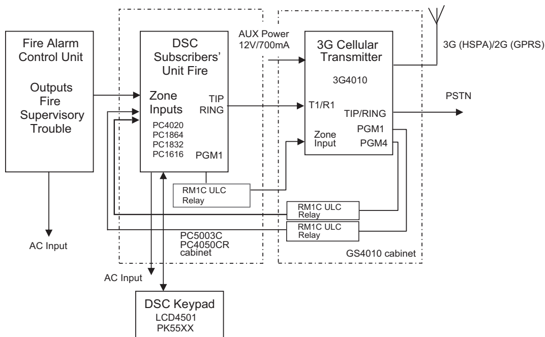
Figure 10-6 DSC Subscribers' Unit Fire and 3G Cellular Transmitter Mounted Remotely Alternate Wiring Diagram for DSC Subscribers' Unit Fire and Cellular Transmitter Passive Communication System - Using Phone Line Supervision Relay
