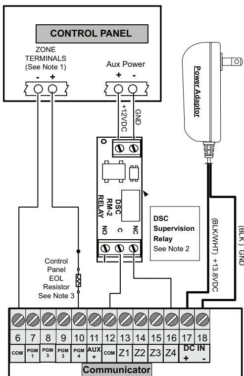
Figure 10-3 Power Supply and Supervision Wiring Diagram
