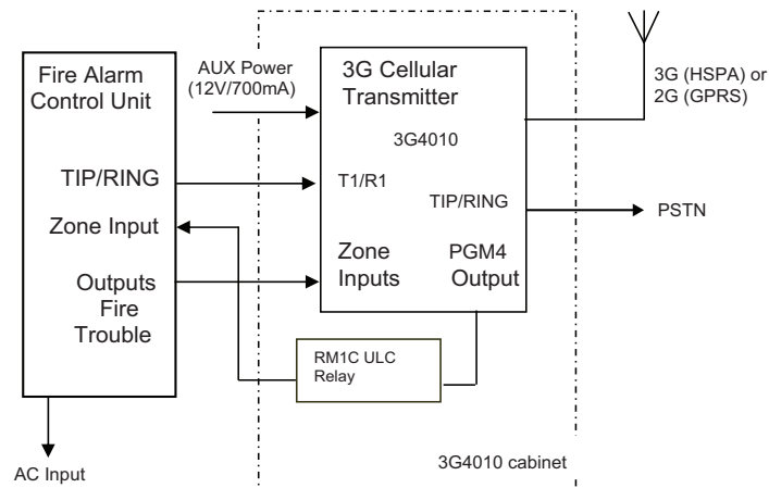
Figure 10-4 Wiring Diagram for Fire Alarm Control Unit (with dialler) and Cellular Transmitter (Passive Communication System)
