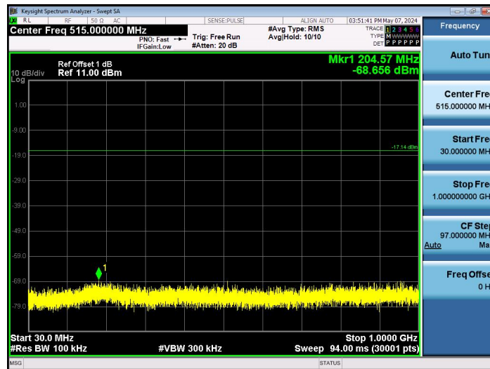
Zigbee-Ant1-2440-30~1000-PASS
