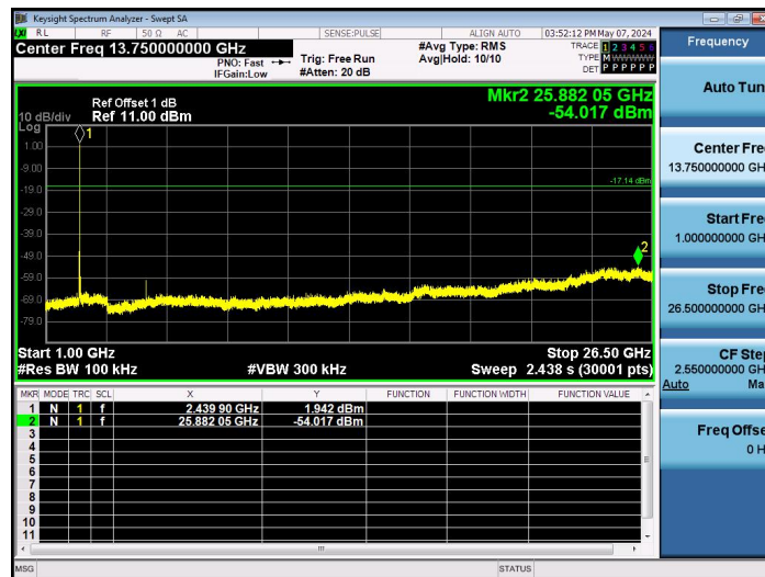
Zigbee-Ant1-2440-1000~26500-PASS
