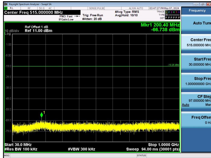
Zigbee-Ant1-2405-30~1000-PASS
