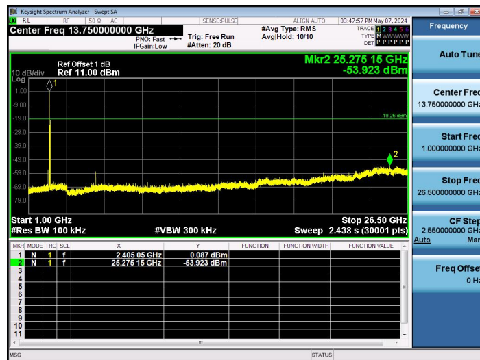
Zigbee-Ant1-2405-1000~26500-PASS
