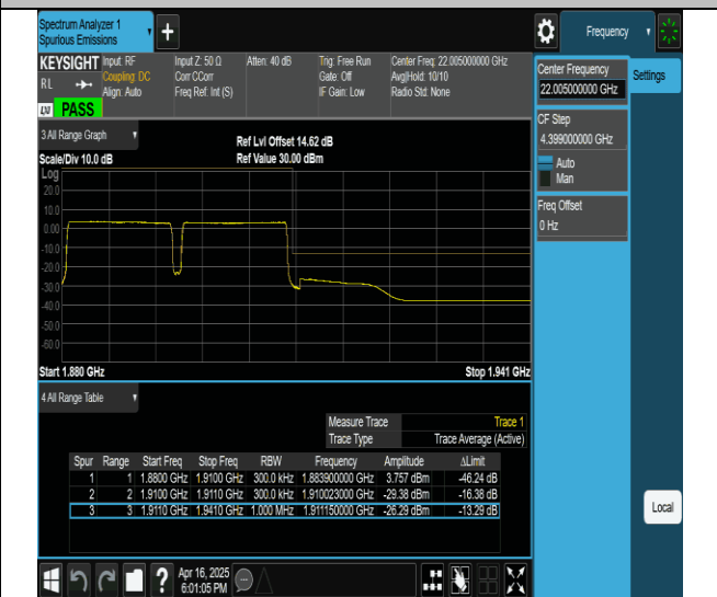
2-2-15MHz-15MHz-QPSK@QPSK-QPSK@QPSK-18975-19125- 75RB#0@0RB#0-0RB#0@0RB#0-PASS
