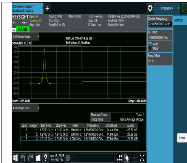
2-2-15MHz-20MHz-QPSK@QPSK-QPSK-18929-19100- 1RB#74@0RB#0-0RB#0@0RB#0-PASS
