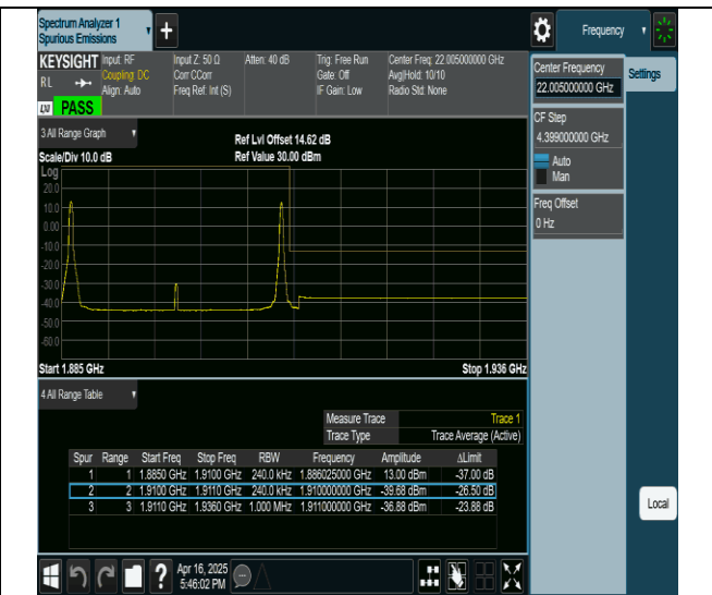
2-2-15MHz-10MHz-QPSK@QPSK-QPSK@QPSK-19027-19147- 1RB#0@0RB#0-1RB#49@0RB#0-PASS
