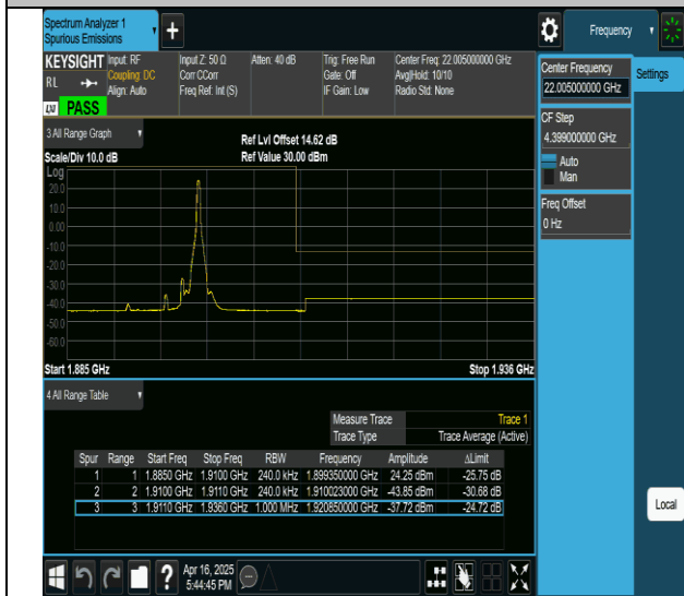
2-2-15MHz-10MHz-QPSK@QPSK-QPSK@QPSK-19027-19147- 1RB#74@0RB#0-0RB#0@0RB#0-PASS
