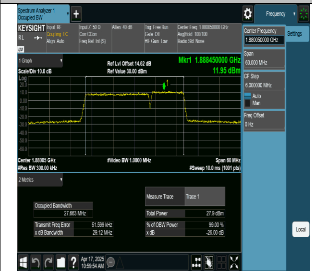
2-2-20MHz-10MHz-256QAM-256QAM-18851-18995-100RB#0-50RB#0-PASS
