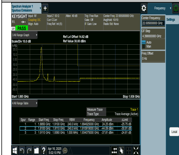
2-2-10MHz-15MHz-QPSK@QPSK-QPSK@QPSK-19005-19125- 1RB#49@0RB#0-0RB#0@0RB#0-PASS
