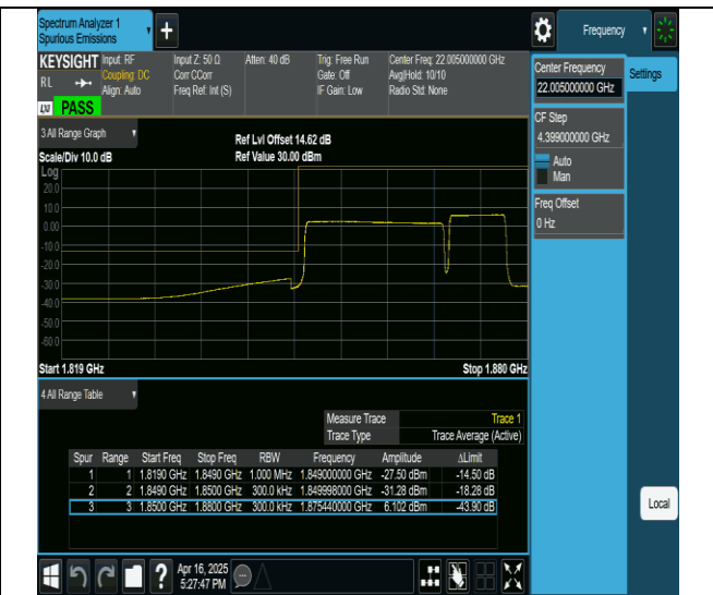
2-2-20MHz-10MHz-QPSK@QPSK-QPSK-18700-18844- 100RB#0@0RB#0-40RB#0@0RB#0-PASS
