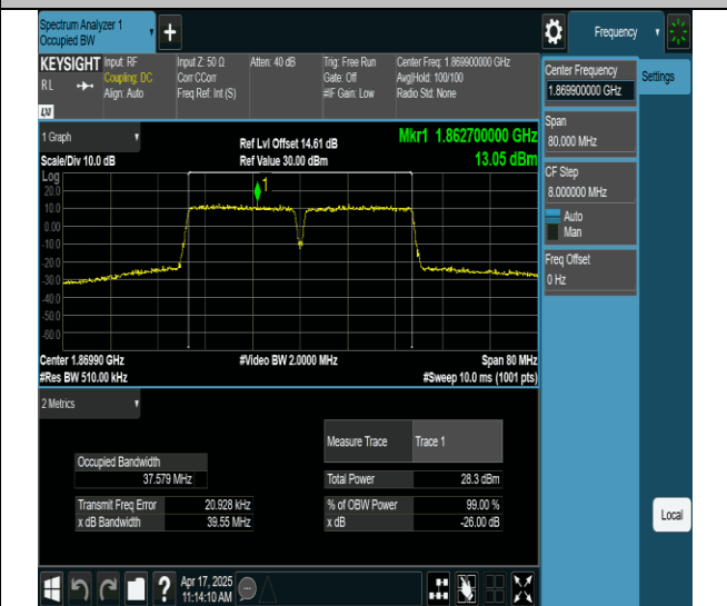
2-2-20MHz-20MHz-256QAM-256QAM-18700-18898-100RB#0-100RB#0-PASS
