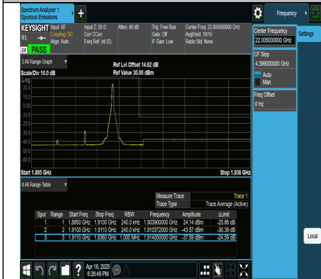
2-2-20MHz-5MHz-QPSK@QPSK-QPSK@QPSK-19050-19167-1RB#99@ORB#0-ORB#0@ORB#0-PASS
