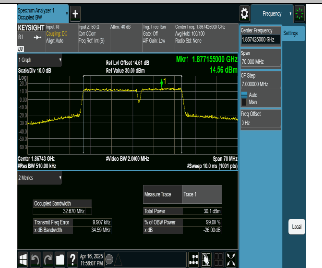
2-2-20MHz-15MHz-16QAM-16QAM-18700-18871-100RB#0- 75RB#0-PASS
