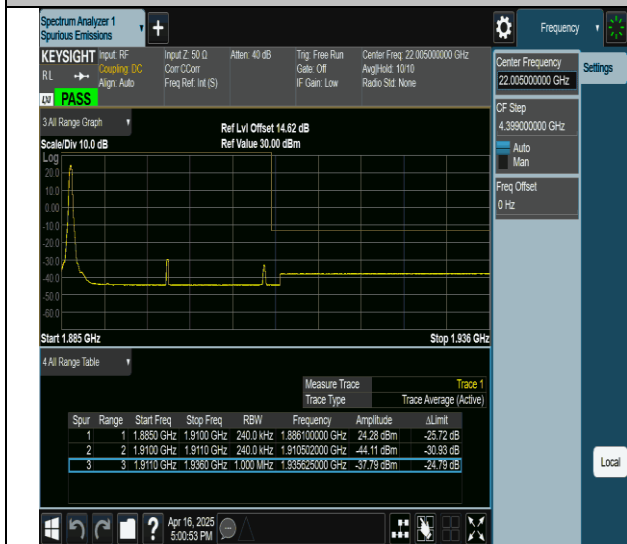
2-2-10MHz-15MHz-QPSK@QPSK-QPSK@QPSK-19005-19125- 1RB#0@0RB#0-0RB#0@0RB#0-PASS
