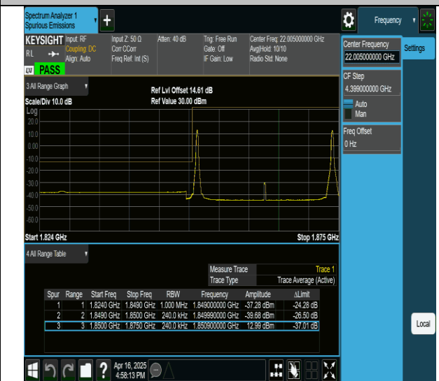
2-2-10MHz-15MHz-QPSK@QPSK-QPSK@QPSK-18653-18773-1RB#0@ORB#0-1RB#74@ORB#0-PASS
