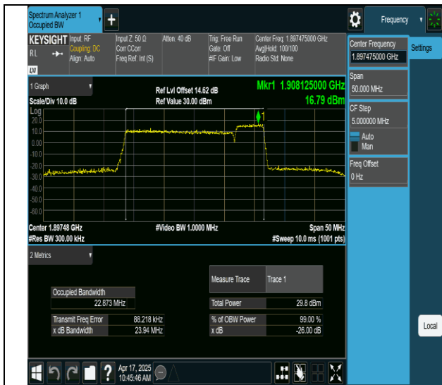
2-2-20MHz-5MHz-64QAM-64QAM-19050-19167-100RB#0-25RB#0-PASS
