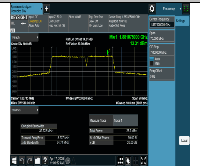
2-2-20MHz-15MHz-256QAM-256QAM-18700-18871-100RB#0- 75RB#0-PASS
