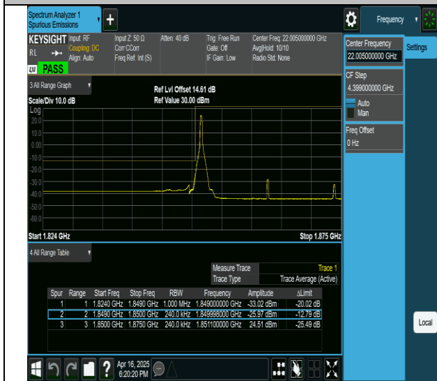
2-2-20MHz-5MHz-QPSK@QPSK-QPSK-18700-18817- 1RB#0@0RB#0-0RB#0@0RB#0-PASS
