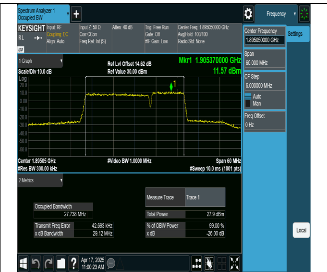
2-2-20MHz-10MHz-256QAM-256QAM-19001-19145-100RB#0- 50RB#0-PASS
