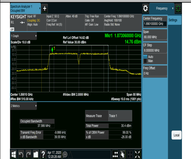
2-2-20MHz-20MHz-16QAM-16QAM-18902-19100-100RB#0-100RB#0-PASS
