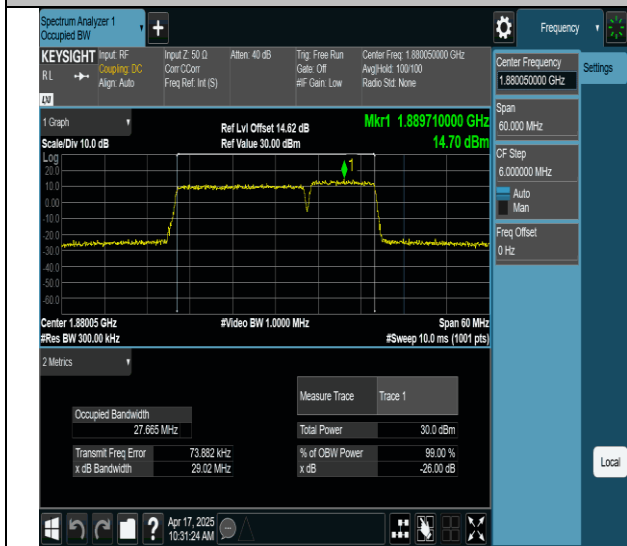
2-2-20MHz-10MHz-64QAM-64QAM-18851-18995-100RB#0-50RB#0-PASS
