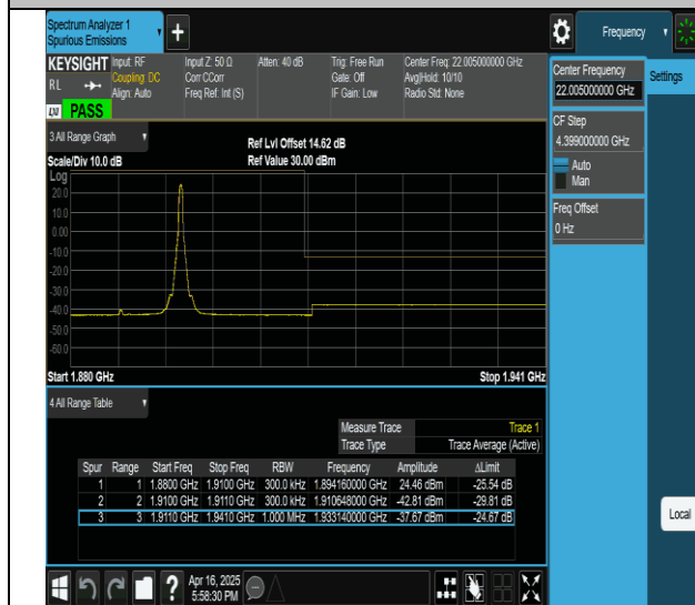
2-2-15MHz-15MHz-QPSK@QPSK-QPSK@QPSK-18975-19125- 1RB#74@0RB#0-0RB#0@0RB#0-PASS
