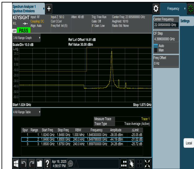
2-2-10MHz-15MHz-QPSK@QPSK-QPSK@QPSK-18653-18773- 1RB#49@0RB#0-0RB#0@0RB#0-PASS
