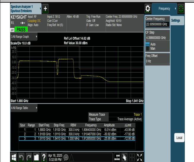
2-2-20MHz-10MHz-QPSK@QPSK-QPSK-19001-19145- 100RB#0@0RB#0-40RB#0@0RB#0-PASS
