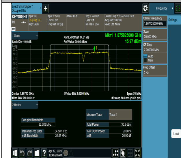
2-2-20MHz-15MHz-64QAM-64QAM-18700-18871-100RB#0- 75RB#0-PASS
