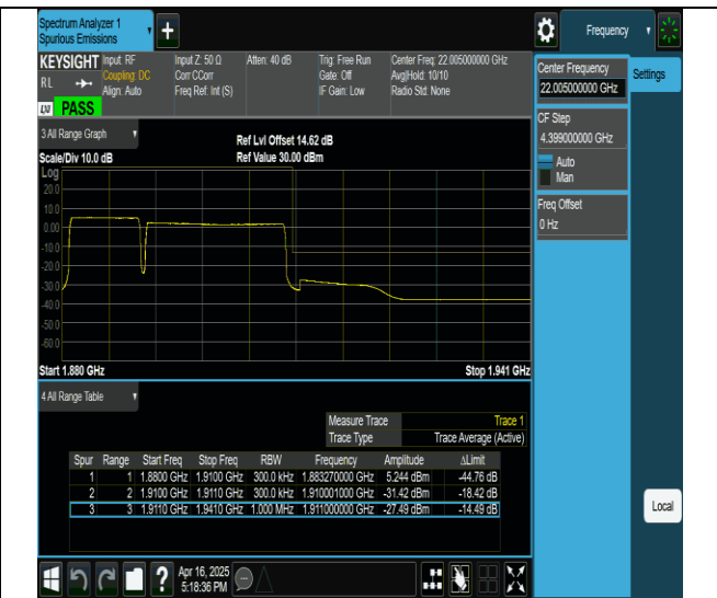
2-2-10MHz-20MHz-QPSK@QPSK-QPSK@QPSK-18956-19100- 50RB#0@0RB#0-100RB#0@0RB#0-PASS
