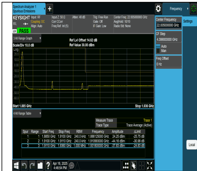
2-2-5MHz-20MHz-QPSK@QPSK-QPSK@QPSK-18983-19100-1RB#0@ORB#0-ORB#0@ORB#0-PASS
