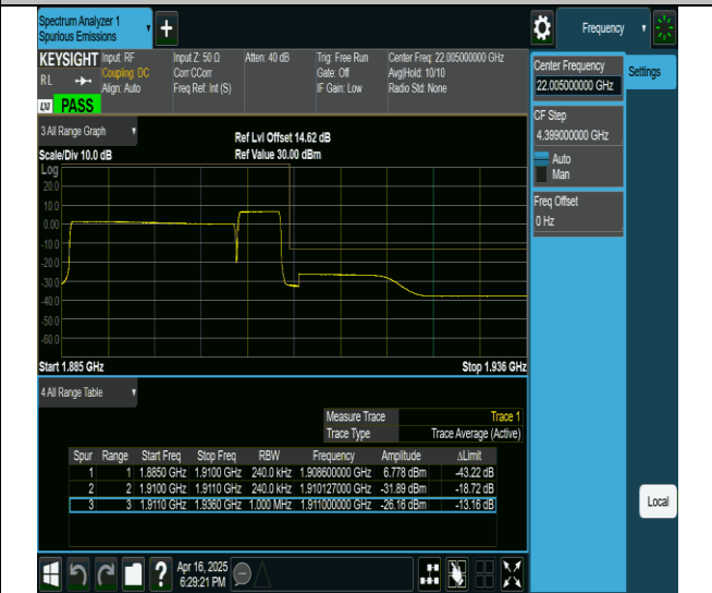
2-2-20MHz-5MHz-QPSK@QPSK-QPSK@QPSK-19050-19167-100RB#0@ORB#0-25RB#0@ORB#0-PASS
