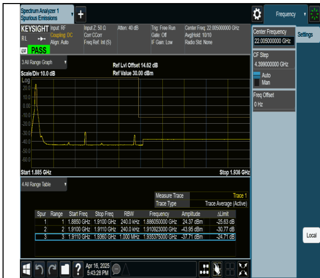
2-2-15MHz-10MHz-QPSK@QPSK-QPSK@QPSK-19027-19147- 1RB#0@0RB#0-0RB#0@0RB#0-PASS
