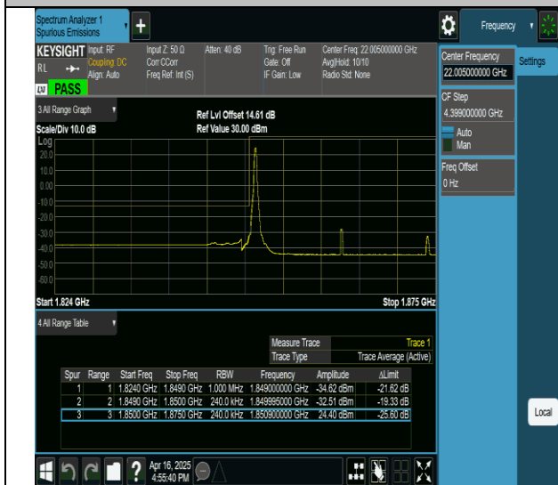
2-2-10MHz-15MHz-QPSK@QPSK-QPSK@QPSK-18653-18773-1RB#0@ORB#0-ORB#0@ORB#0-PASS
