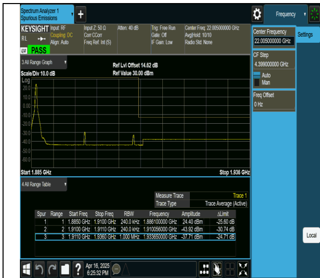
2-2-20MHz-5MHz-QPSK@QPSK-QPSK@QPSK-19050-19167-1RB#0@ORB#0-ORB#0@ORB#0-PASS
