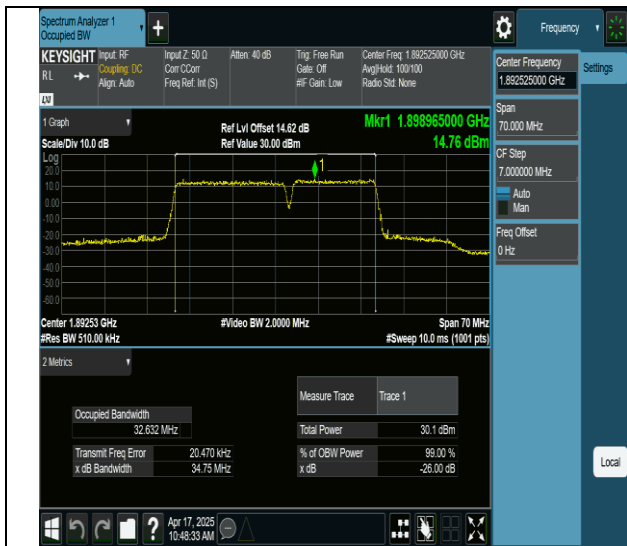
2-2-20MHz-15MHz-64QAM-64QAM-18951-19122-100RB#0-75RB#0-PASS
