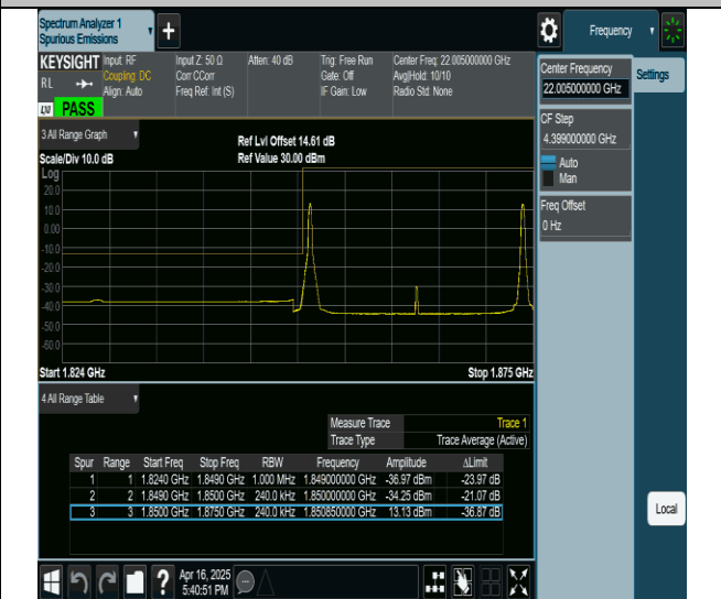
2-2-15MHz-10MHz-QPSK@QPSK-QPSK@QPSK-18675-18795- 1RB#0@0RB#0-1RB#49@0RB#0-PASS
