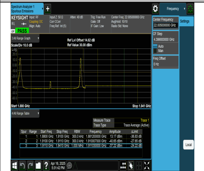
2-2-20MHz-10MHz-QPSK@QPSK-QPSK-19001-19145- 1RB#0@0RB#0-1RB#49@0RB#0-PASS
