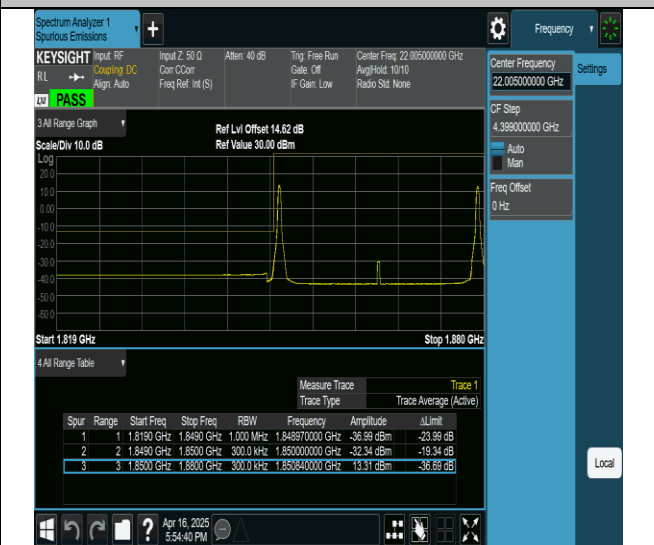
2-2-15MHz-15MHz-QPSK@QPSK-QPSK@QPSK-18675-18825- 1RB#0@0RB#0-1RB#74@0RB#0-PASS
