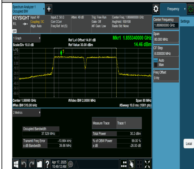
2-2-20MHz-20MHz-64QAM-64QAM-18700-18898-100RB#0-100RB#0-PASS
