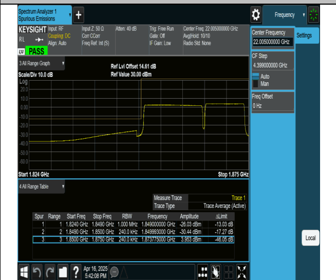
2-2-15MHz-10MHz-QPSK@QPSK-QPSK@QPSK-18675-18795- 75RB#0@0RB#0-50RB#0@0RB#0-PASS
