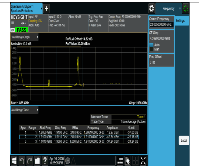
2-2-20MHz-5MHz-QPSK@QPSK-QPSK@QPSK-19050-19167-1RB#0@ORB#0-1RB#24@ORB#0-PASS
