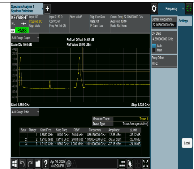
2-2-5MHz-20MHz-QPSK@QPSK-QPSK@QPSK-18983-19100-1RB#0@ORB#0-1RB#99@ORB#0-PASS
