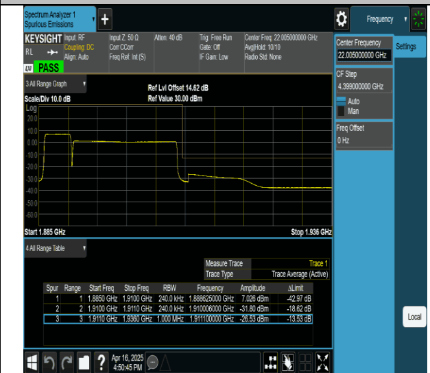
2-2-5MHz-20MHz-QPSK@QPSK-QPSK@QPSK-18983-19100-25RB#0@ORB#0-100RB#0@ORB#0-PASS
