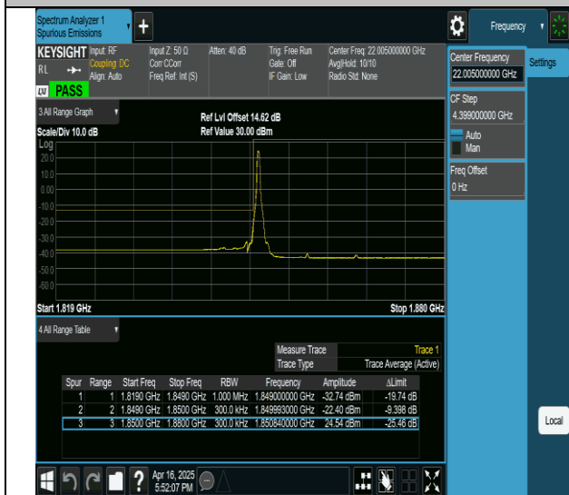
2-2-15MHz-15MHz-QPSK@QPSK-QPSK@QPSK-18675-18825- 1RB#0@0RB#0-0RB#0@0RB#0-PASS
