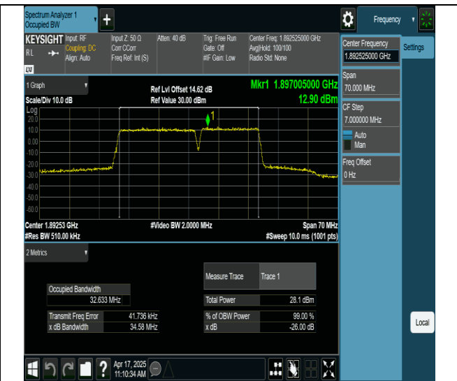
2-2-20MHz-15MHz-256QAM-256QAM-18951-19122-100RB#0-75RB#0-PASS
