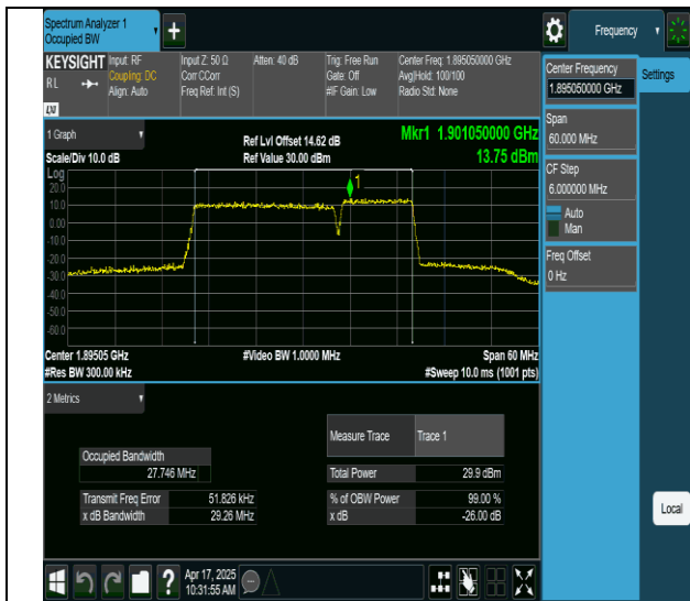
2-2-20MHz-10MHz-64QAM-64QAM-19001-19145-100RB#0- 50RB#0-PASS
