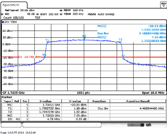
Band4-5MHz-16QAM-20175-25RB#0-4.456
