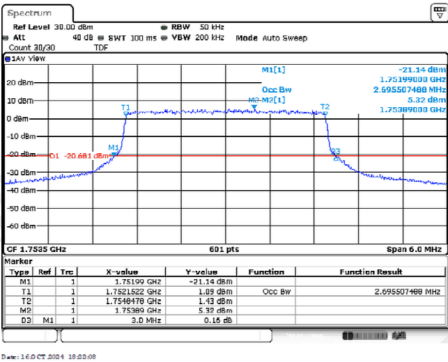
Band4-3MHz-QPSK-20385-15RB#0-2.696
