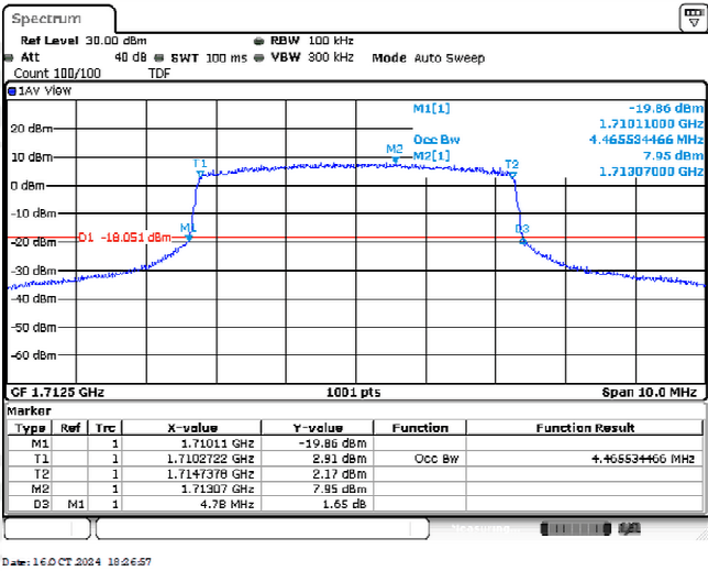
Band4-5MHz-QPSK-19975-25RB#0-4.466
