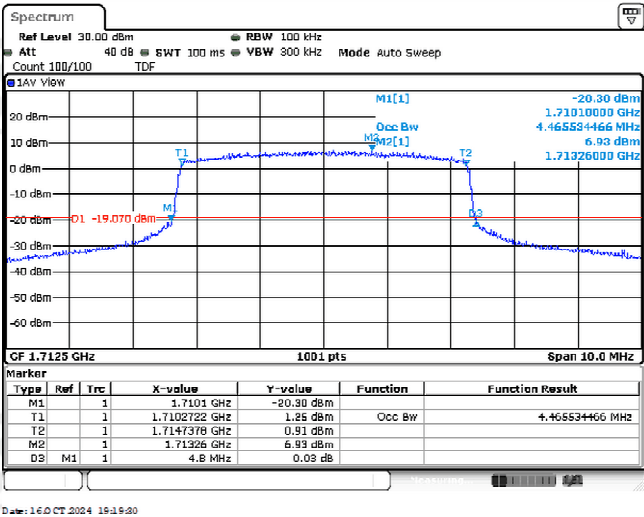
Band4-5MHz-16QAM-19975-25RB#0-4.466
