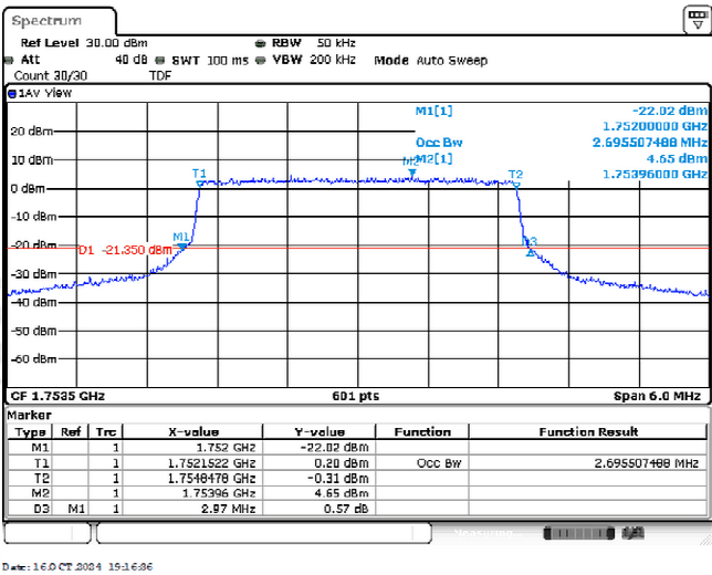
Band4-3MHz-16QAM-20385-15RB#0-2.696
