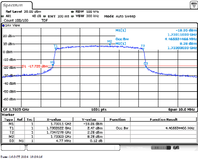
Band4-5MHz-QPSK-20175-25RB#0-4.466
