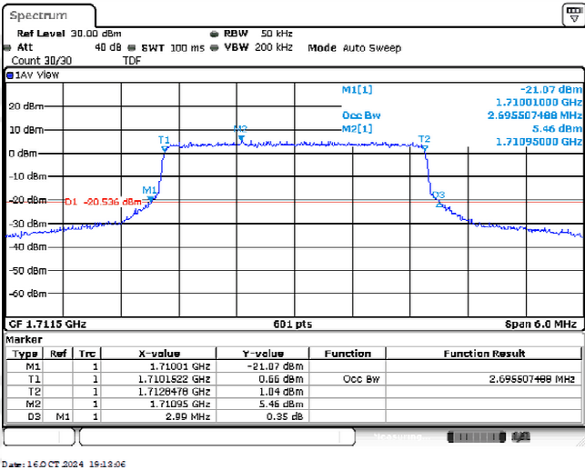
Band4-3MHz-16QAM-19965-15RB#0-2.696
