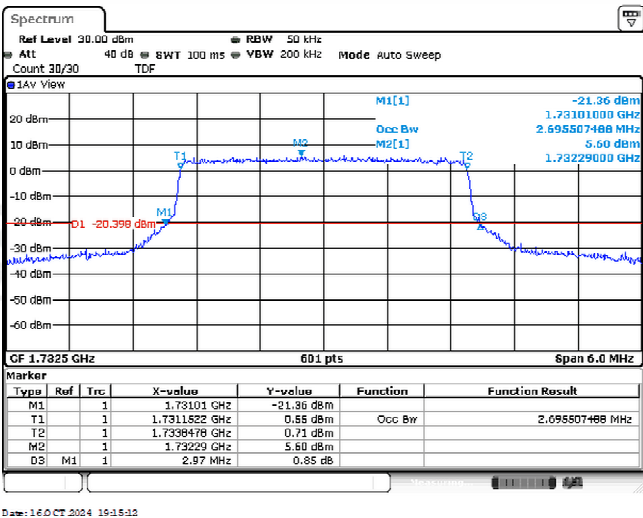
Band4-3MHz-16QAM-20175-15RB#0-2.696
