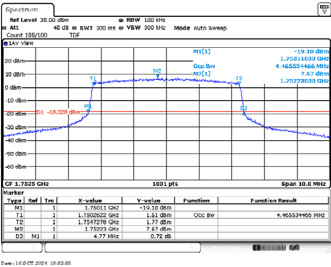
Band4-5MHz-QPSK-20375-25RB#0-4.466
