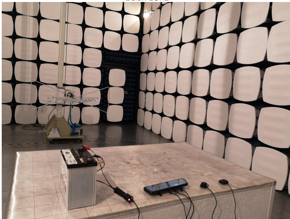
DC 12V Radiated Emission Below 1GHz
