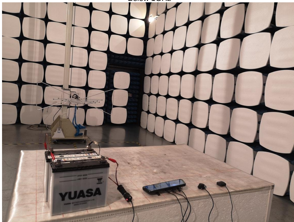
DC 24V Radiated Emission Below 1GHz
