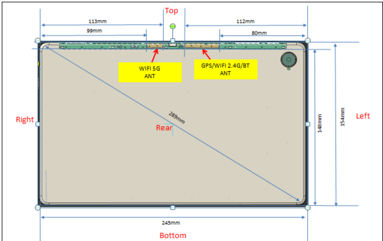
Fig.13.1 EUT Antenna Locations
