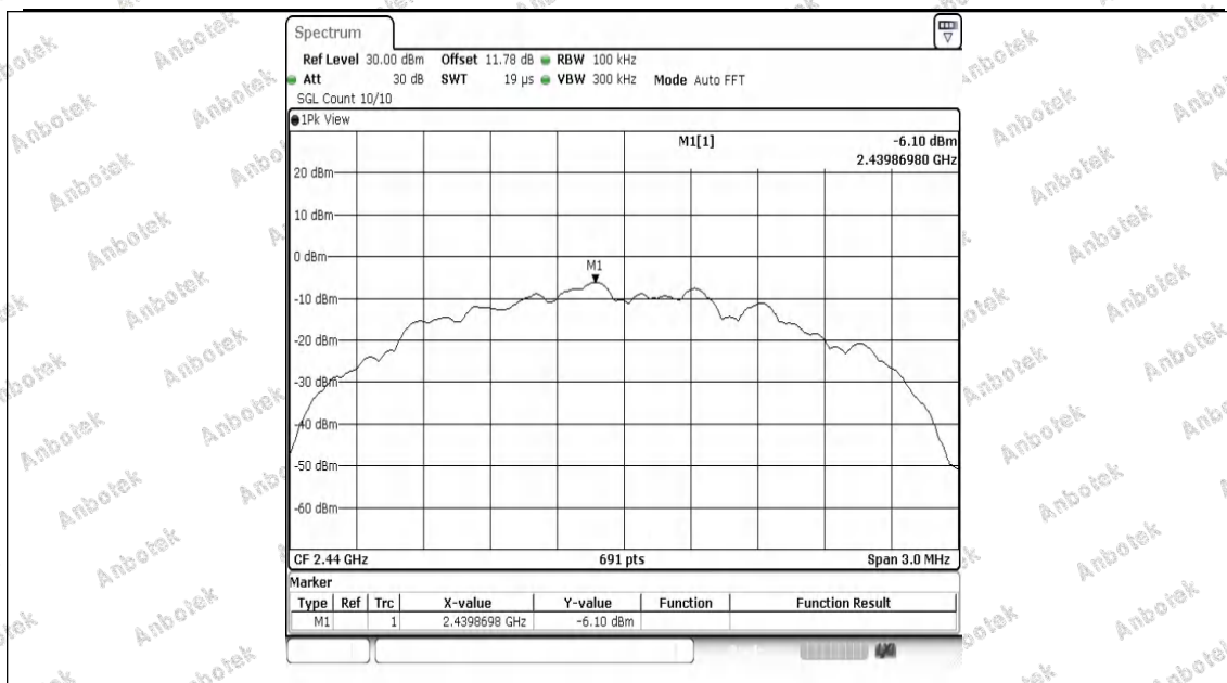
BLE_2M-Ant1-2440-0~Reference-PASS
