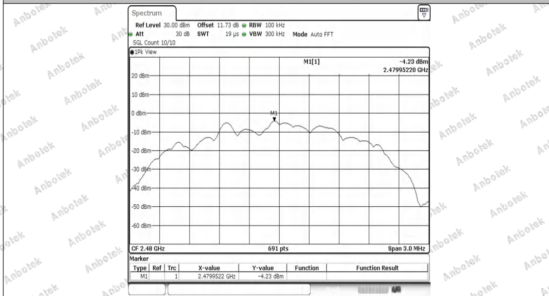
BLE_2M-Ant1-2480-0~Reference-PASS
