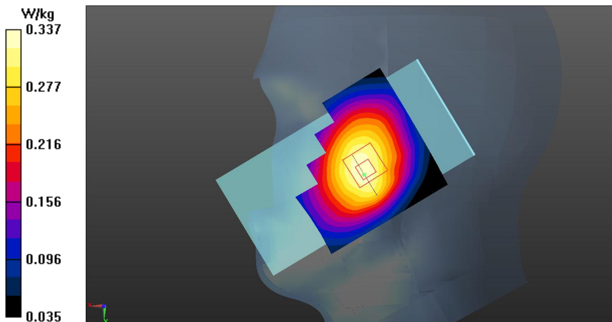
Fig.1 GSM 850 Head
