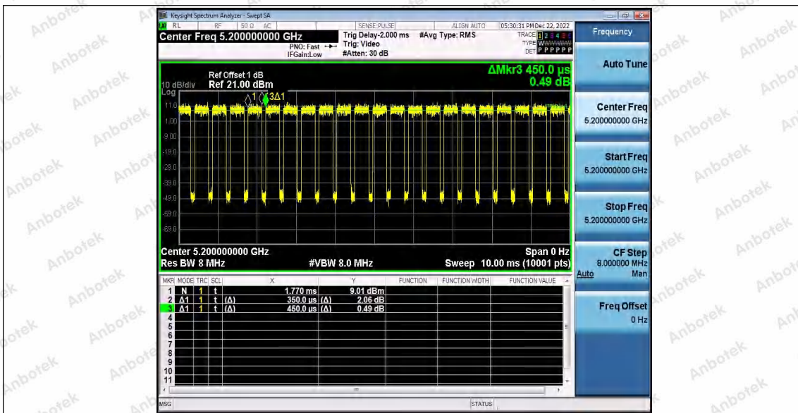
11AC20SISO_Ant2_5200
