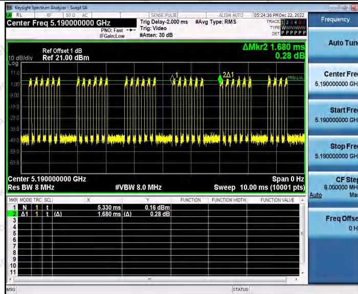
11N40SISO_Ant2_5190
