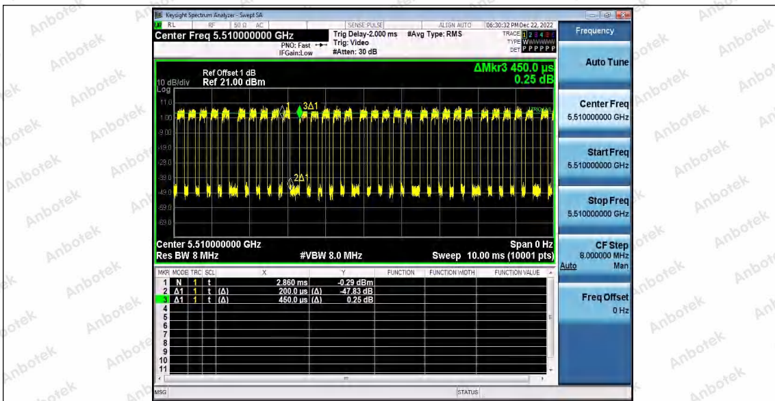
11AC40SISO_Ant2_5510
