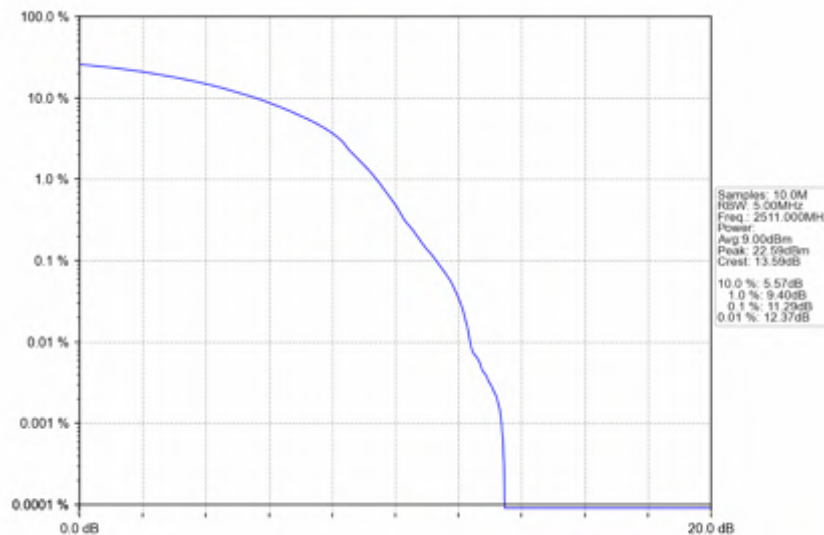
n41_30kHz_SISO_NTNV_30MHz_DFT-s-OFDM_256_QAM_2511MHz_Outer_Full
