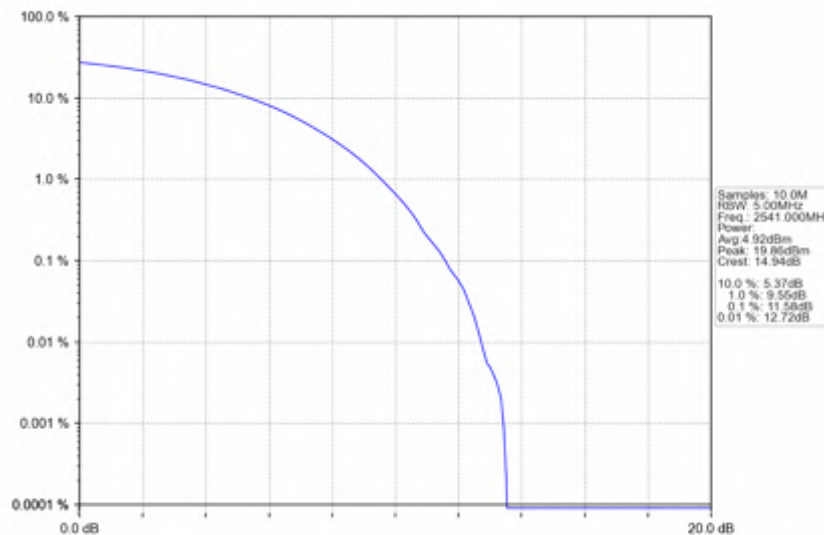
n41_30kHz_SISO_NTNV_90MHz_CP-OFDM_64_QAM_2541MHz_Outer_Full
