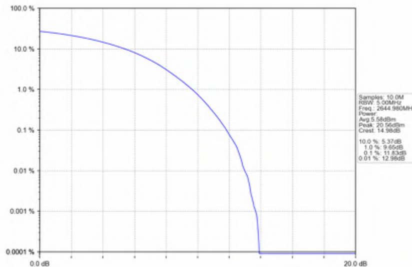
n41_30kHz_SISO_NTNV_90MHz_CP-OFDM_16_QAM_2644.98MHz_Outer_Full
