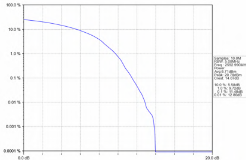
n41_30kHz_SISO_NTNV_90MHz_DFT-s-OFDM QPSK_2592.99MHz_Outer_Full
