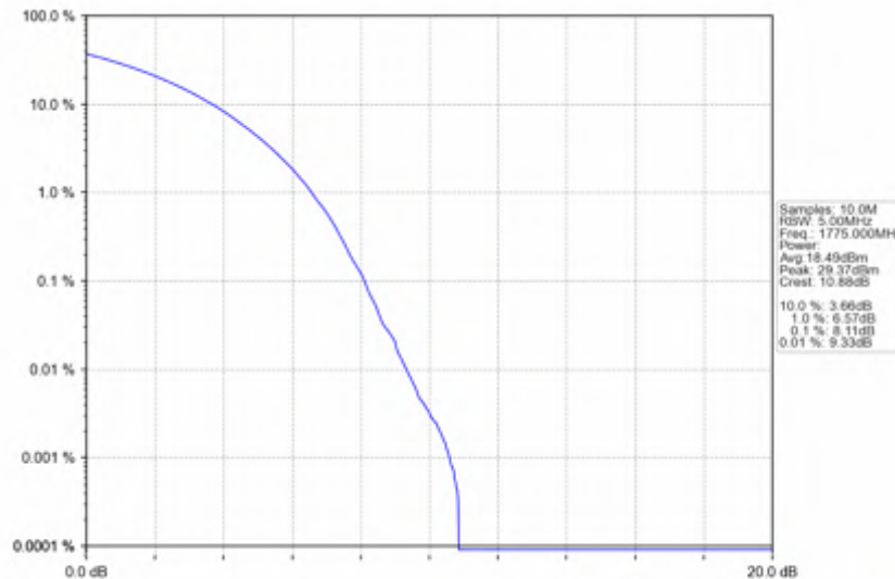
n66_15kHz_SISO_NTNV_10MHz_CP-OFDM 16 QAM_1775MHz_Outer_Full
