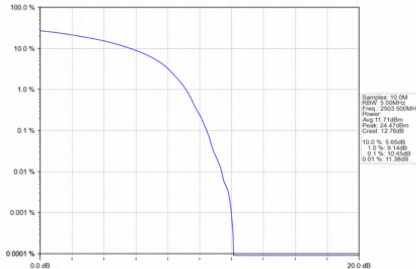
n41_30kHz_SISO_NTNV_15MHz_DFT-s-OFDM_256_QAM_2503.5MHz_Outer_Full
