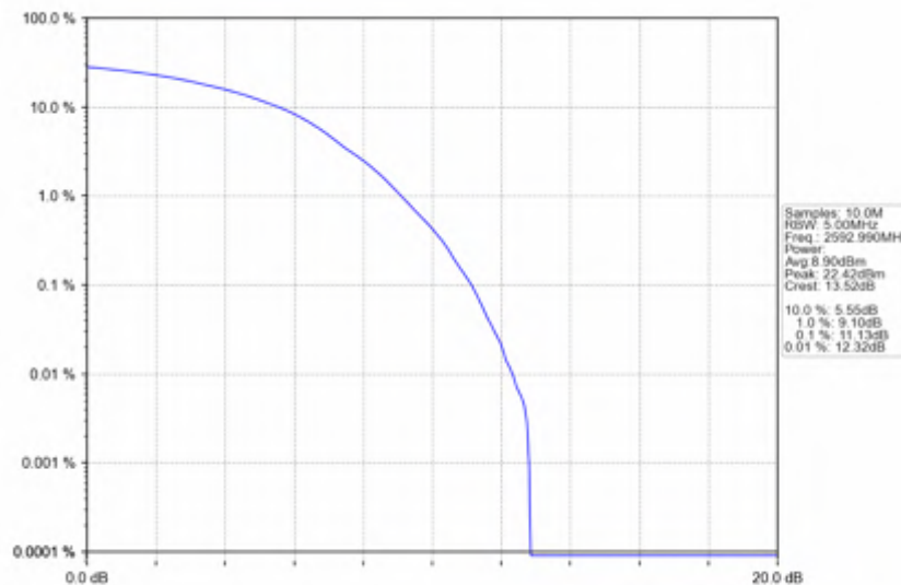
n41_30kHz_SISO_NTNV_60MHz_DFT-s-OFDM QPSK_2592.99MHz_Outer_Full
