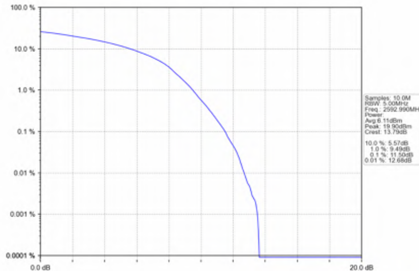
n41_30kHz_SISO_NTNV_100MHz_DFT-s-OFDM QPSK_2592.99MHz_Outer_Full
