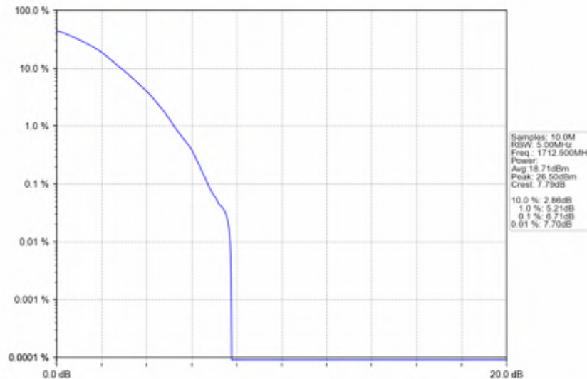
n66_15kHz_SISO_NTNV_5MHz_DFT-s-OFDM_256_QAM_1712.5MHz_Outer_Full
