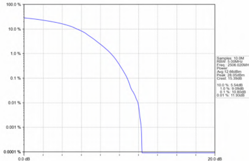
n41_30kHz_SISO_NTNV_20MHz_DFT-s-OFDM_16_QAM_2506.02MHz_Outer_Full
