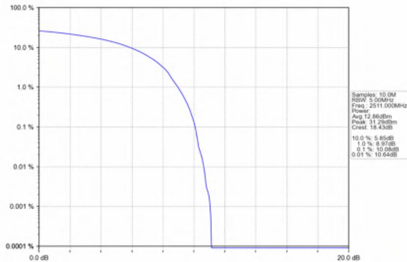
n41_30kHz_SISO_NTNV_30MHz_DFT-s-OFDM_PI/2_BPSK_2511MHz_Outer_Full
