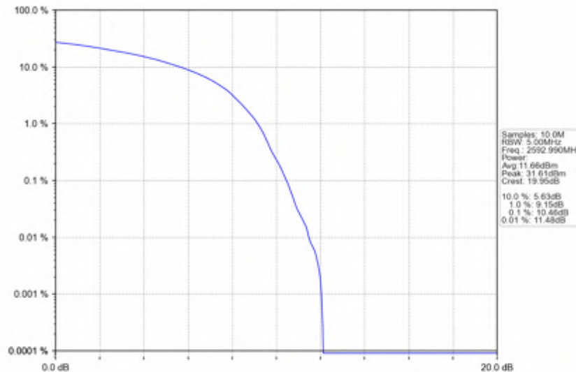
n41_30kHz_SISO_NTNV_15MHz_DFT-s-OFDM_256_QAM_2592.99MHz_Outer_Full
