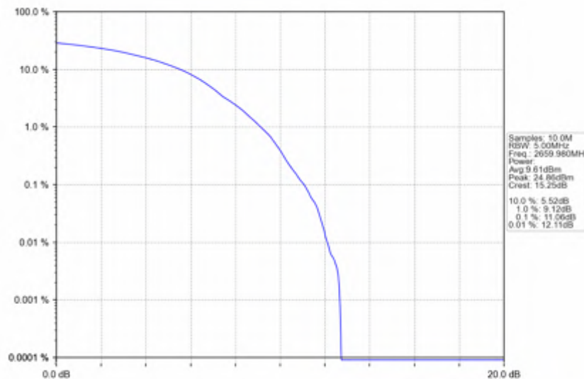
n41_30kHz_SISO_NTNV_60MHz_DFT-s-OFDM_PI/2_BPSK_2659.98MHz_Outer_Full
