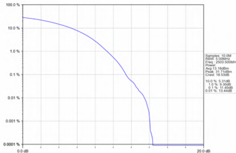
n41_30kHz_SISO_NTNV_15MHz_CP-OFDM_16_QAM_2503.5MHz_Outer_Full
