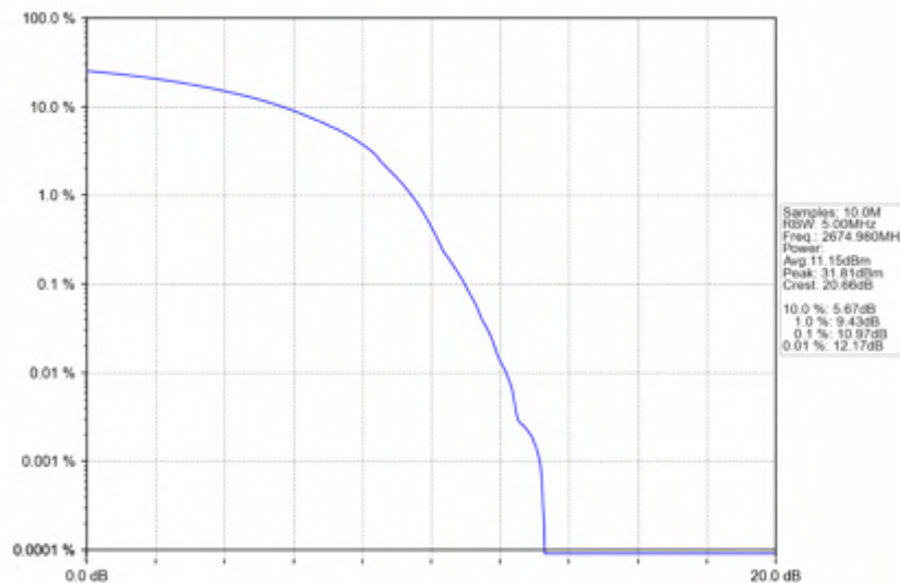
n41_30kHz_SISO_NTNV_30MHz_DFT-s-OFDM_64_QAM_2674.98MHz_Outer_Full
