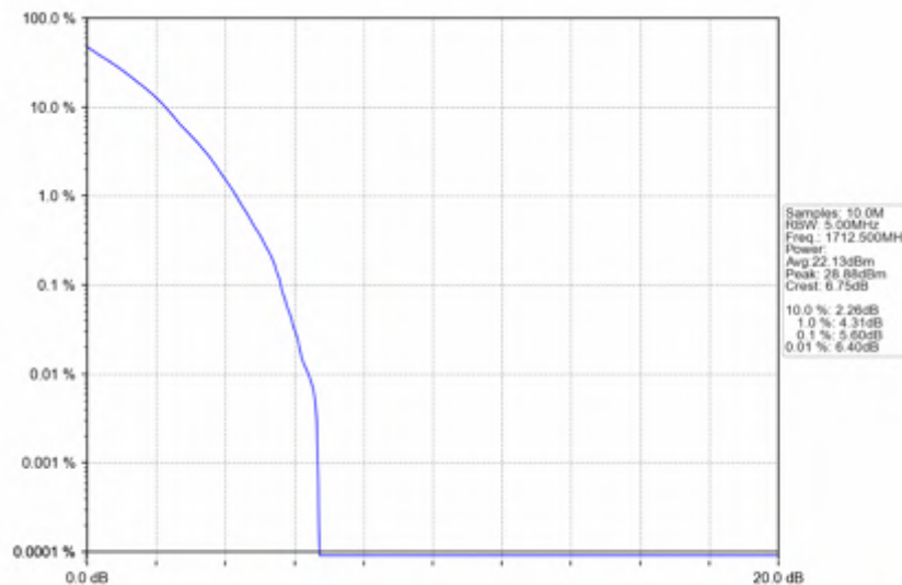
n66_15kHz_SISO_NTNV_5MHz_DFT-s-OFDM QPSK_1712.5MHz_Outer_Full
