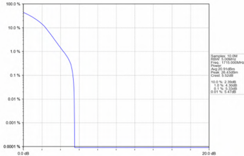
n66_15kHz_SISO_NTNV_10MHz_DFT-s-OFDM_PI/2_BPSK_1715MHz_Outer_Full
