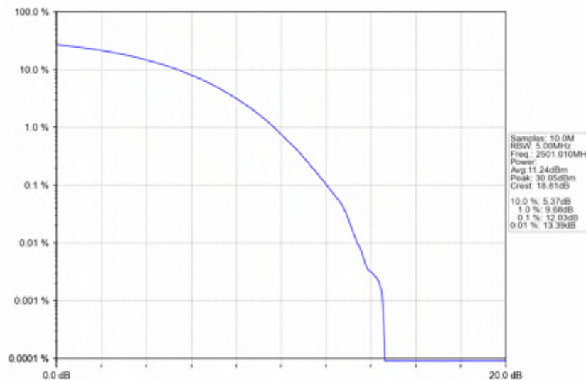
n41_30kHz_SISO_NTNV_10MHz_CP-OFDM_256_QAM_2501.01MHz_Outer_Full
