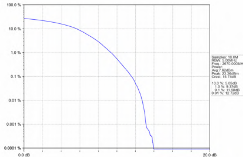
n41_30kHz_SISO_NTNV_40MHz_DFT-s-OFDM 256 QAM_2670MHz_Outer_Full
