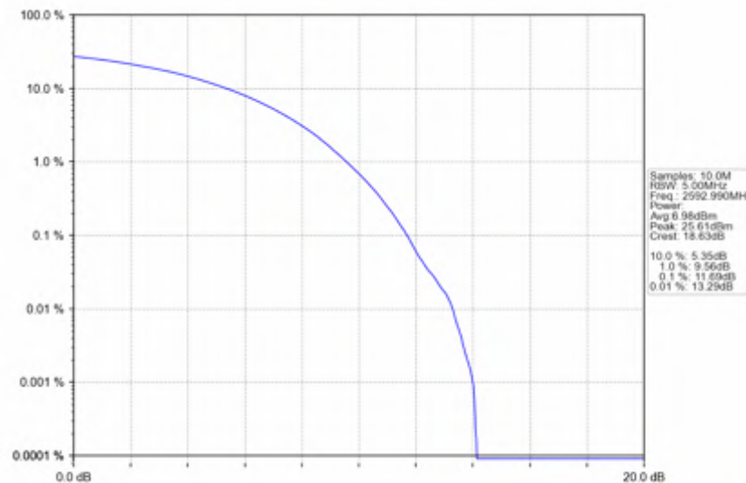
n41_30kHz_SISO_NTNV_60MHz_CP-OFDM QPSK_2592.99MHz_Outer_Full
