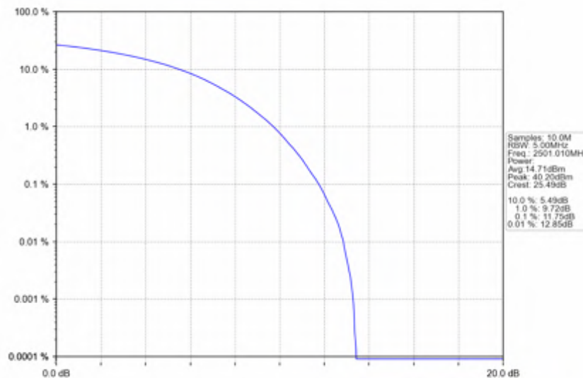
n41_30kHz_SISO_NTNV_10MHz_CP-OFDM_16_QAM_2501.01MHz_Outer_Full
