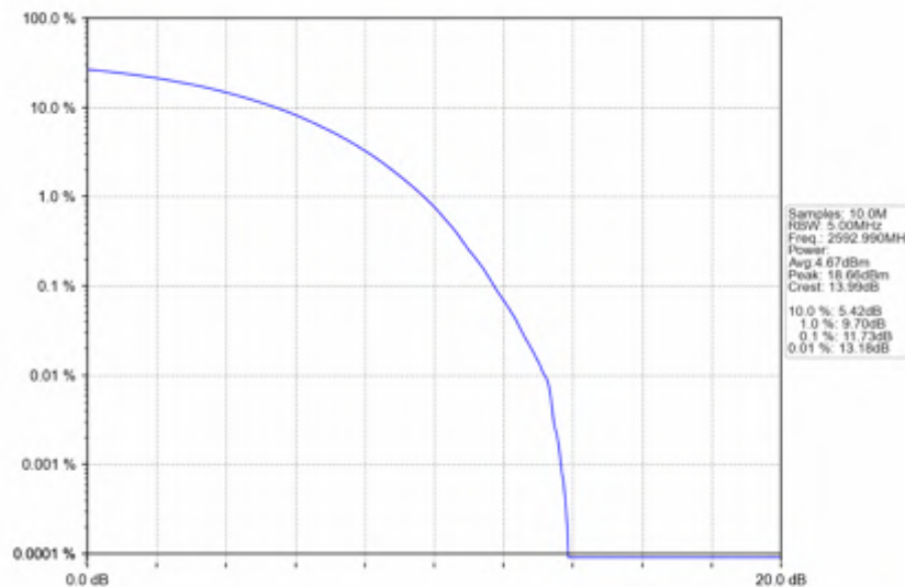
n41_30kHz_SISO_NTNV_90MHz_CP-OFDM QPSK_2592.99MHz_Outer_Full
