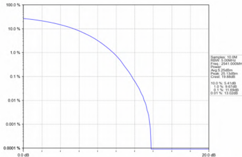
n41_30kHz_SISO_NTNV_90MHz_CP-OFDM QPSK_2541MHz_Outer_Full
