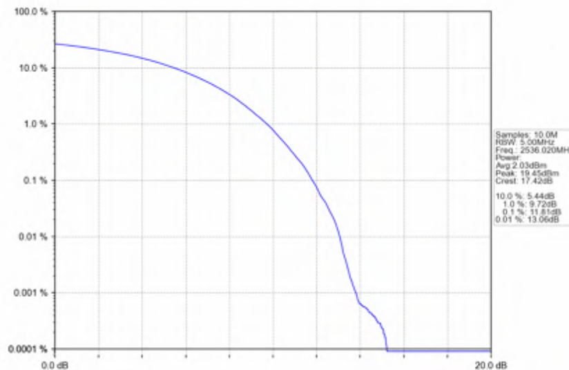
n41_30kHz_SISO_NTNV_80MHz_CP-OFDM_256_QAM_2536.02MHz_Outer_Full
