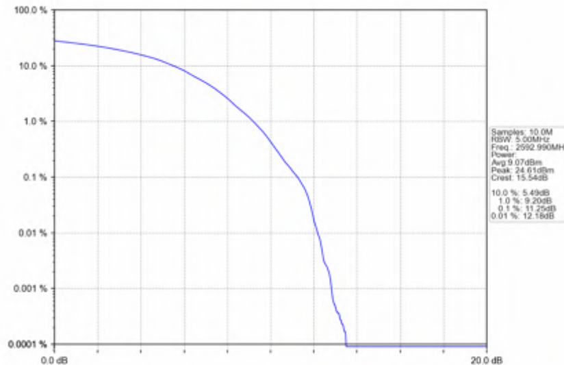
n41_30kHz_SISO_NTNV_50MHz_DFT-s-OFDM_16_QAM_2592.99MHz_Outer_Full
