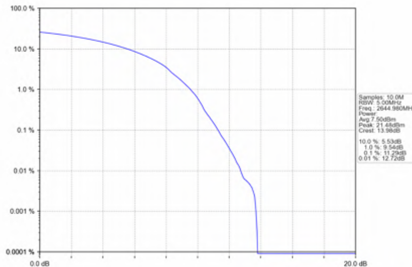
n41_30kHz_SISO_NTNV_90MHz_DFT-s-OFDM QPSK_2644.98MHz_Outer_Full
