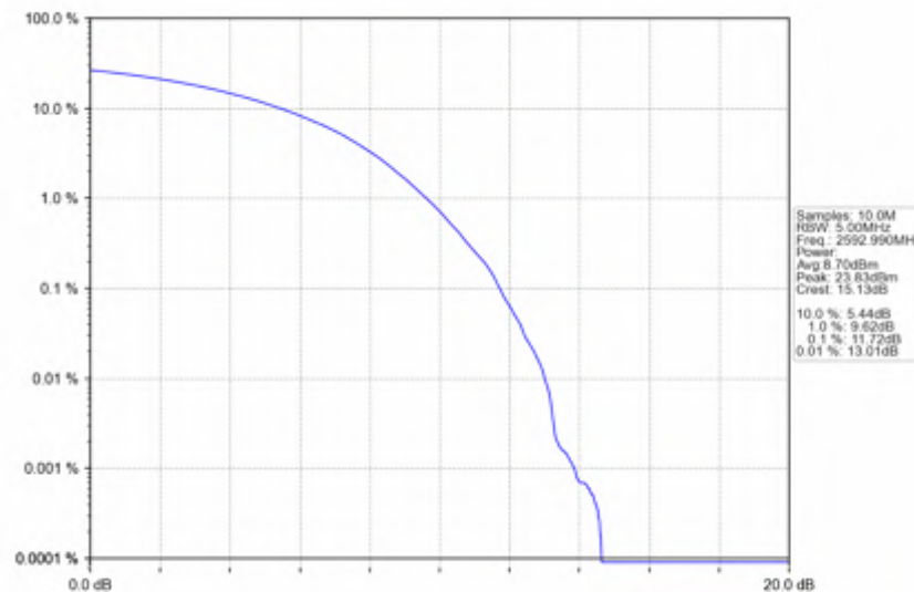
n41_30kHz_SISO_NTNV_40MHz_CP-OFDM_16_QAM_2592.99MHz_Outer_Full
