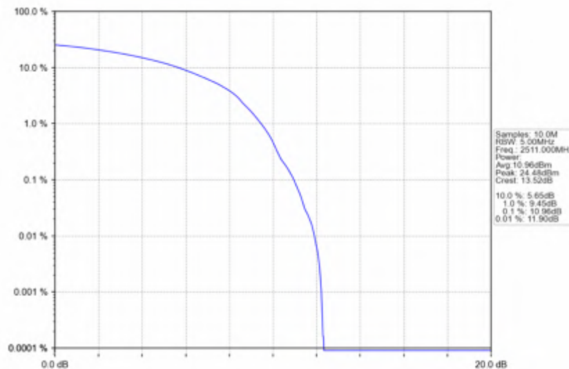
n41_30kHz_SISO_NTNV_30MHz_DFT-s-OFDM_64_QAM_2511MHz_Outer_Full
