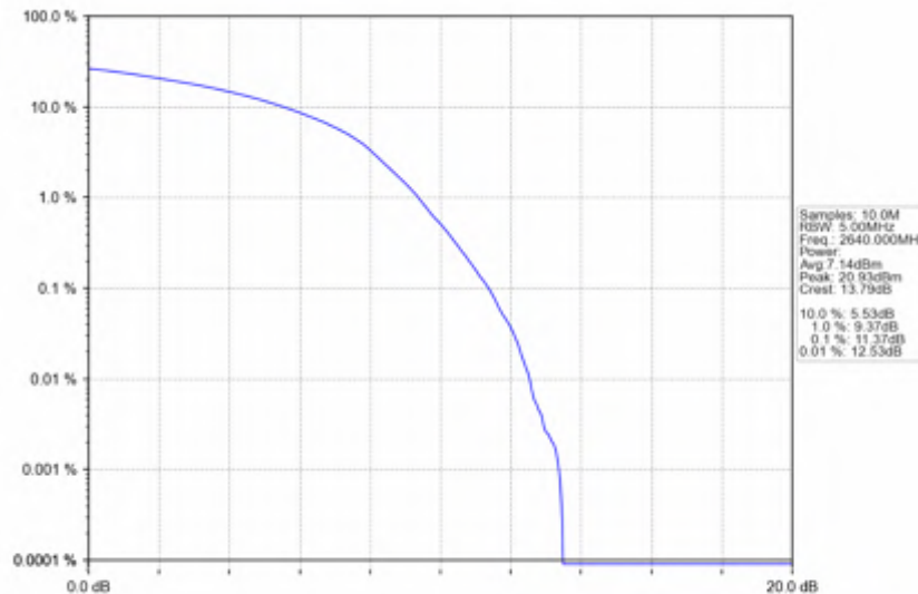
n41_30kHz_SISO_NTNV_100MHz_DFT-s-OFDM QPSK_2640MHz_Outer_Full
