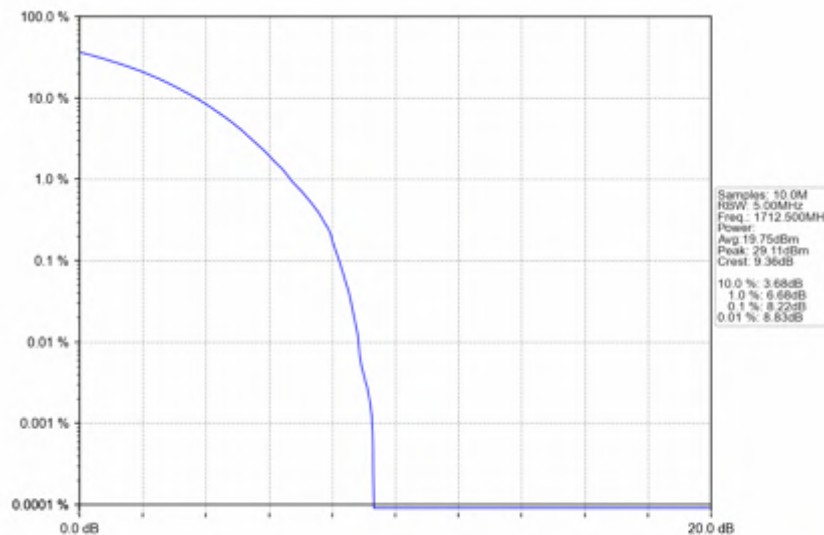
n66_15kHz_SISO_NTNV_5MHz_CP-OFDM_64_QAM_1712.5MHz_Outer_Full
