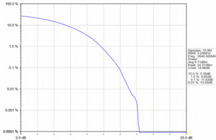
n41_30kHz_SISO_NTNV_100MHz_CP-OFDM 64 QAM_2640MHz_Outer_Full
