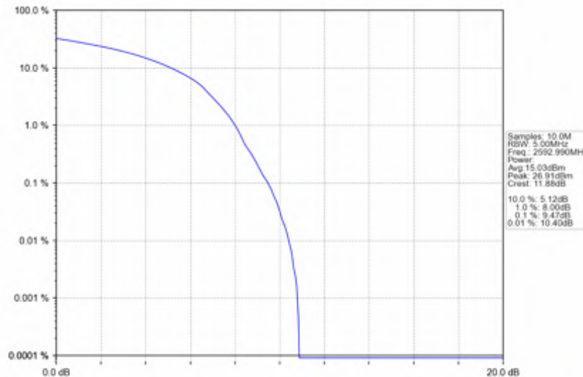
n41_30kHz_SISO_NTNV_15MHz_DFT-s-OFDM_64_QAM_2592.99MHz_Outer_Full
