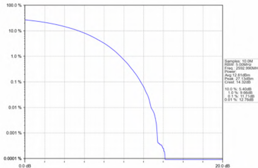
n41_30kHz_SISO_NTNV_15MHz_CP-OFDM QPSK_2592.99MHz_Outer_Full
