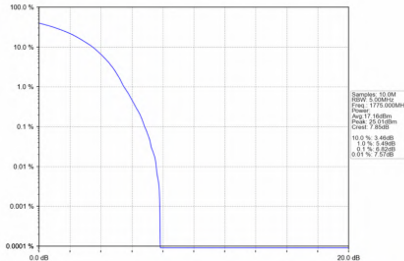
n66_15kHz_SISO_NTNV_10MHz_DFT-s-OFDM 256 QAM_1775MHz_Outer_Full
