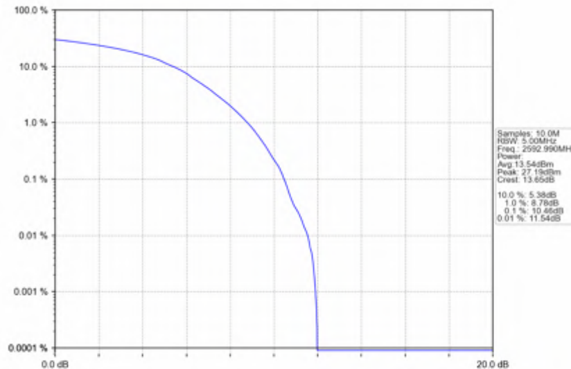
n41_30kHz_SISO_NTNV_20MHz_DFT-s-OFDM_16_QAM_2592.99MHz_Outer_Full
