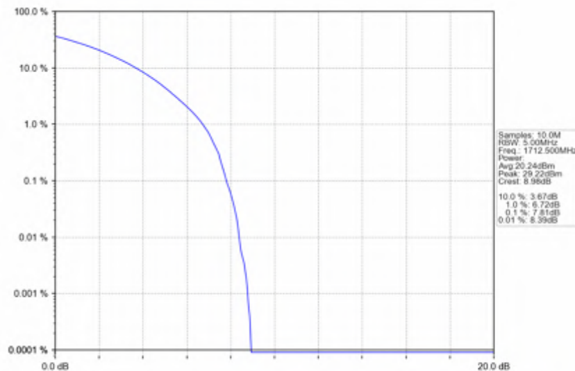
n66_15kHz_SISO_NTNV_5MHz_CP-OFDM QPSK_1712.5MHz_Outer_Full
