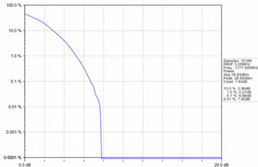
n66_15kHz_SISO_NTNV_5MHz_DFT-s-OFDM 256 QAM_1777.5MHz_Outer_Full
