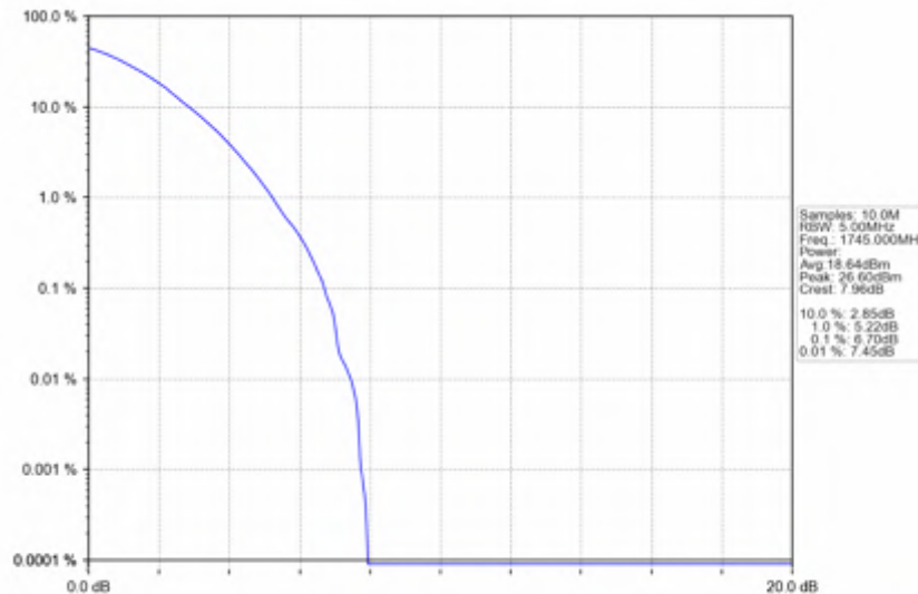
n66_15kHz_SISO_NTNV_5MHz_DFT-s-OFDM_256_QAM_1745MHz_Outer_Full
