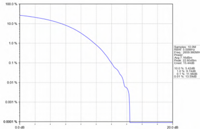
n41_30kHz_SISO_NTNV_60MHz_CP-OFDM QPSK_2659.98MHz_Outer_Full
