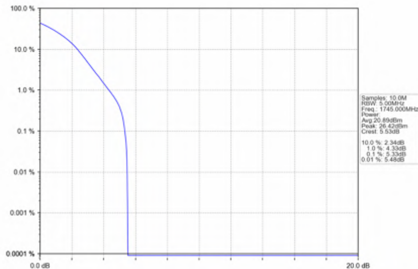
n66 15kHz SISO NTNV 10MHz DFT-s-OFDM PI/2 BPSK 1745MHz Outer Full
