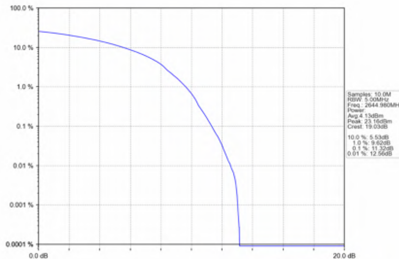
n41_30kHz_SISO_NTNV_90MHz_DFT-s-OFDM 256 QAM_2644.98MHz_Outer_Full
