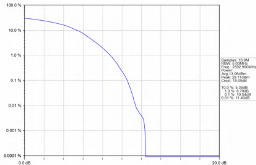
n41_30kHz_SISO_NTNV_20MHz_DFT-s-OFDM 64 QAM_2592.99MHz_Outer_Full
