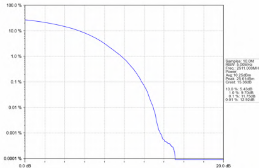
n41_30kHz_SISO_NTNV_30MHz_CP-OFDM QPSK_2511MHz_Outer_Full
