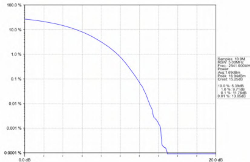
n41_30kHz_SISO_NTNV_90MHz_CP-OFDM 256 QAM_2541MHz_Outer_Full
