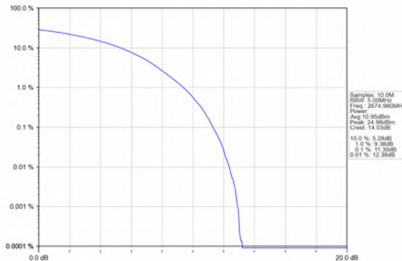
n41_30kHz_SISO_NTNV_30MHz_CP-OFDM QPSK_2674.98MHz_Outer_Full
