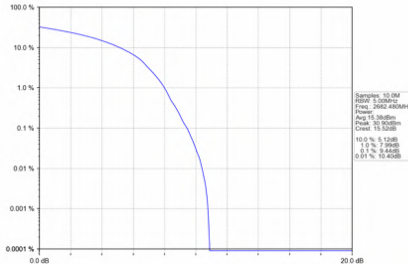
n41_30kHz_SISO_NTNV_15MHz_DFT-s-OFDM_64_QAM_2682.48MHz_Outer_Full
