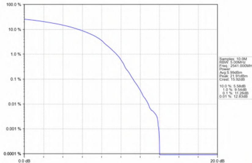
n41_30kHz_SISO_NTNV_90MHz_DFT-s-OFDM_64_QAM_2541MHz_Outer_Full
