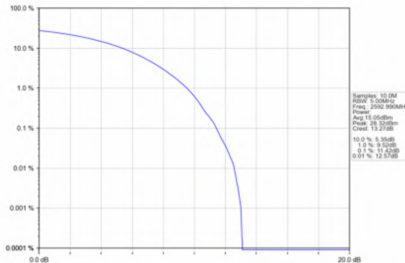
n41_30kHz_SISO_NTNV_10MHz_CP-OFDM_16_QAM_2592.99MHz_Outer_Full
