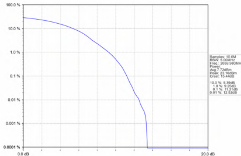
n41_30kHz_SISO_NTNV_60MHz_DFT-s-OFDM 64 QAM_2659.98MHz_Outer_Full
