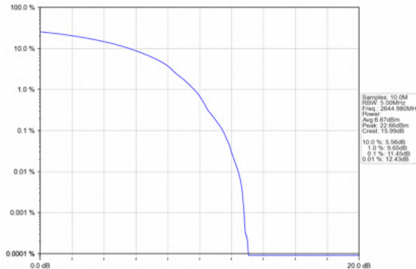
n41_30kHz_SISO_NTNV_90MHz_DFT-s-OFDM_16_QAM_2644.98MHz_Outer_Full
