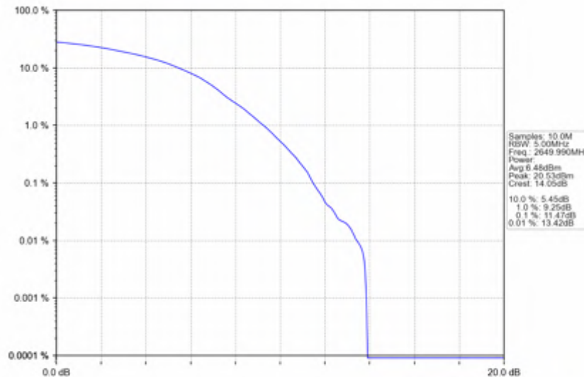
n41_30kHz_SISO_NTNV_80MHz_DFT-s-OFDM 64 QAM_2649.99MHz_Outer_Full
