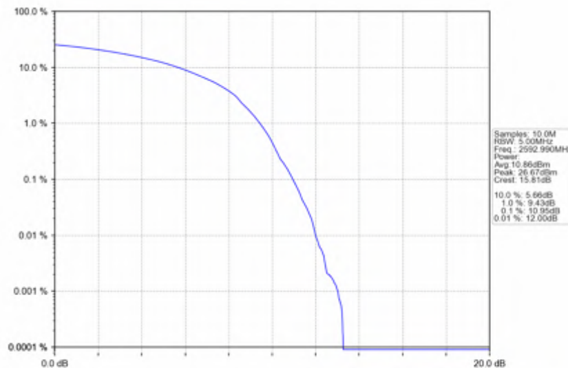
n41_30kHz_SISO_NTNV_30MHz_DFT-s-OFDM_64_QAM_2592.99MHz_Outer_Full
