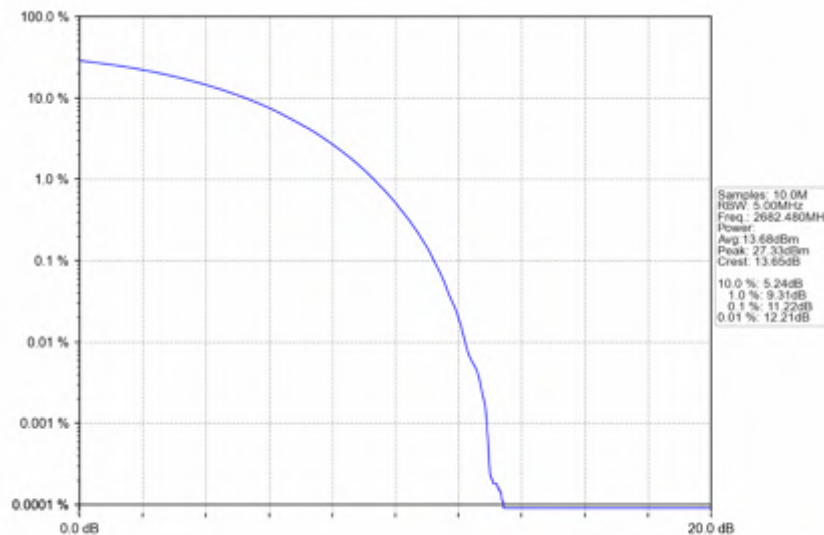
n41_30kHz_SISO_NTNV_15MHz_CP-OFDM QPSK_2682.48MHz_Outer_Full
