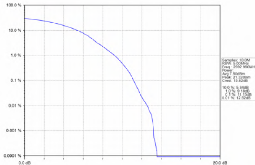
n41_30kHz_SISO_NTNV_60MHz_DFT-s-OFDM 64 QAM_2592.99MHz_Outer_Full
