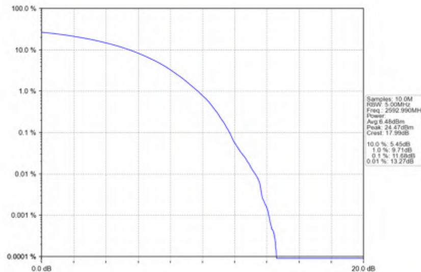
n41_30kHz_SISO_NTNV_30MHz_CP-OFDM 256 QAM_2592.99MHz_Outer_Full
