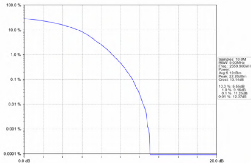
n41_30kHz_SISO_NTNV_60MHz_DFT-s-OFDM QPSK_2659.98MHz_Outer_Full
