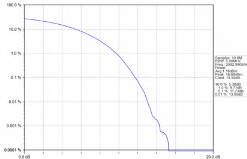
n41_30kHz_SISO_NTNV_90MHz_CP-OFDM 256 QAM_2592.99MHz_Outer_Full
