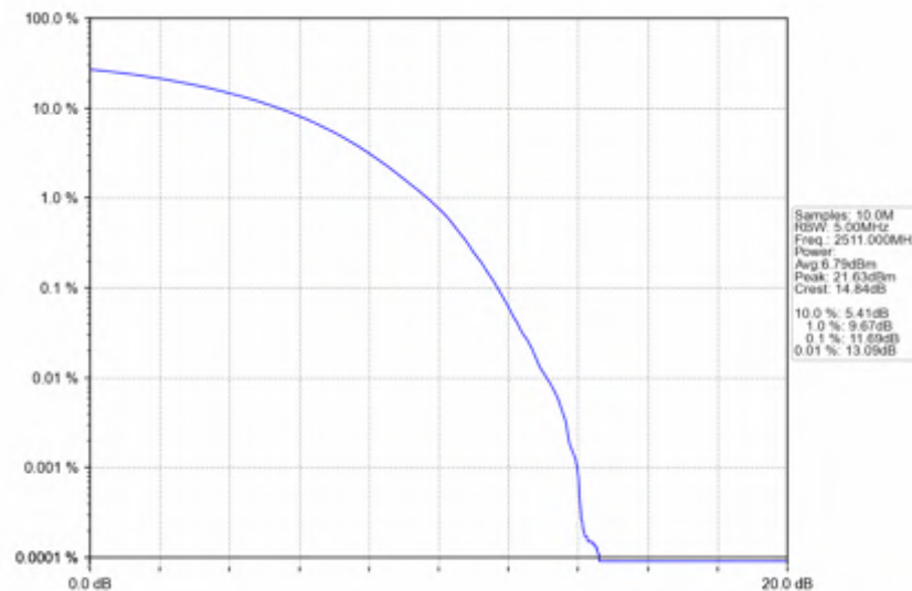
n41_30kHz_SISO_NTNV_30MHz_CP-OFDM 256 QAM_2511MHz_Outer_Full
