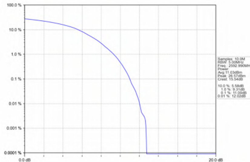
n41_30kHz_SISO_NTNV_40MHz_DFT-s-OFDM QPSK_2592.99MHz_Outer_Full
