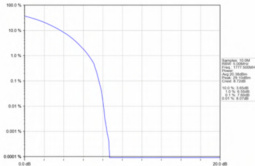
n66_15kHz_SISO_NTNV_5MHz_CP-OFDM_16_QAM_1777.5MHz_Outer_Full
