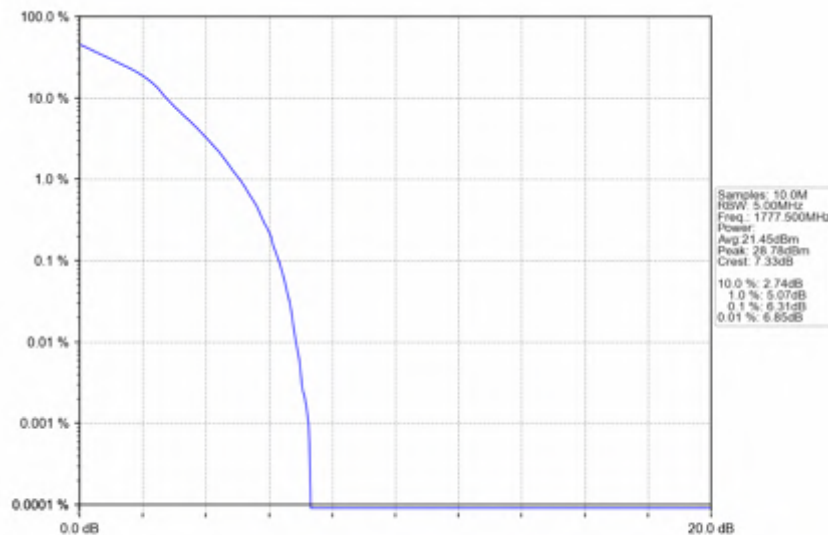
n66_15kHz_SISO_NTNV_5MHz_DFT-s-OFDM_16_QAM_1777.5MHz_Outer_Full
