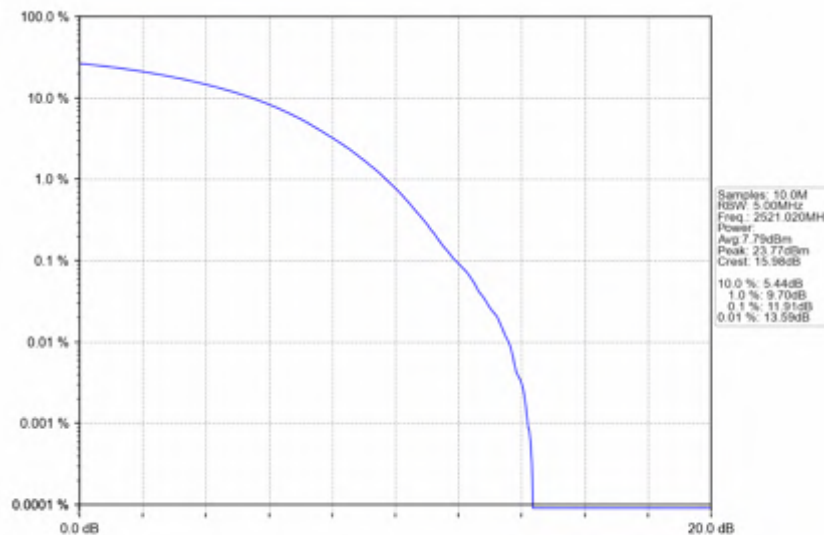
n41_30kHz_SISO_NTNV_50MHz_CP-OFDM_16_QAM_2521.02MHz_Outer_Full
