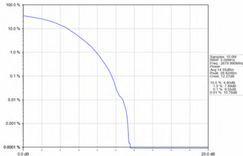
n41_30kHz_SISO_NTNV_20MHz_DFT-s-OFDM 64 QAM_2679.99MHz_Outer_Full
