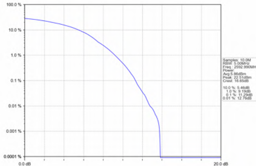
n41_30kHz_SISO_NTNV_80MHz_DFT-s-OFDM 64 QAM_2592.99MHz_Outer_Full
