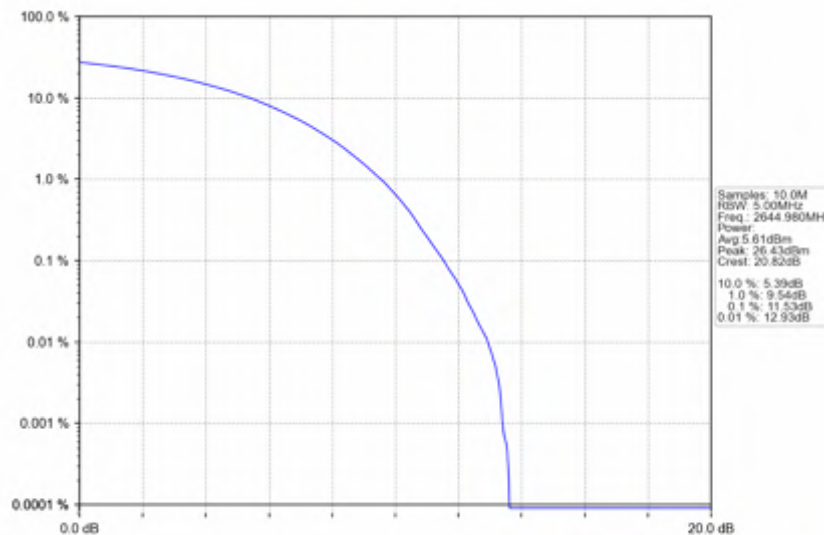
n41_30kHz_SISO_NTNV_90MHz_CP-OFDM QPSK_2644.98MHz_Outer_Full
