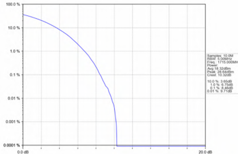
n66_15kHz_SISO_NTNV_10MHz_CP-OFDM QPSK_1715MHz_Outer_Full
