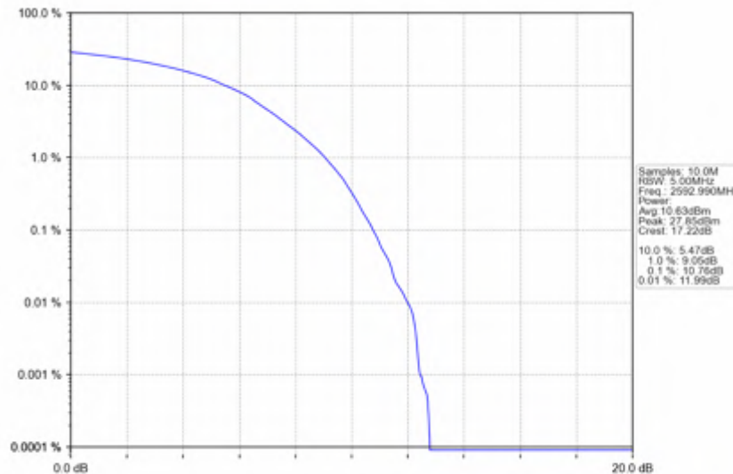
n41_30kHz_SISO_NTNV_20MHz_DFT-s-OFDM_256_QAM_2592.99MHz_Outer_Full
