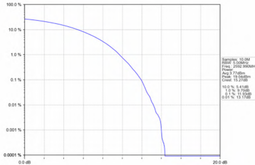
n41_30kHz_SISO_NTNV_100MHz_CP-OFDM 64 QAM_2592.99MHz_Outer_Full
