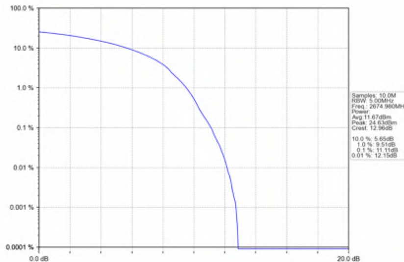
n41_30kHz_SISO_NTNV_30MHz_DFT-s-OFDM_16_QAM_2674.98MHz_Outer_Full
