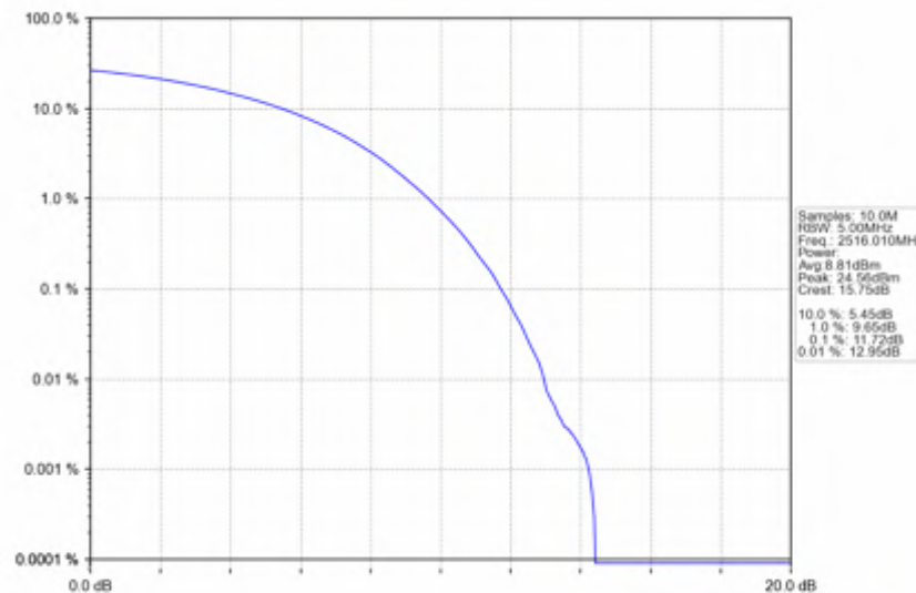
n41_30kHz_SISO_NTNV_40MHz_CP-OFDM QPSK_2516.01MHz_Outer_Full
