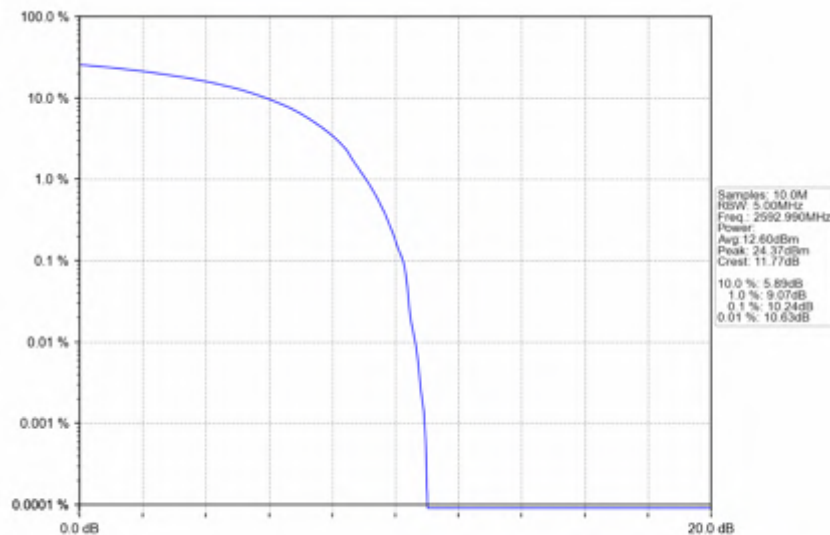
n41_30kHz_SISO_NTNV_30MHz_DFT-s-OFDM_PI/2_BPSK_2592.99MHz_Outer_Full
