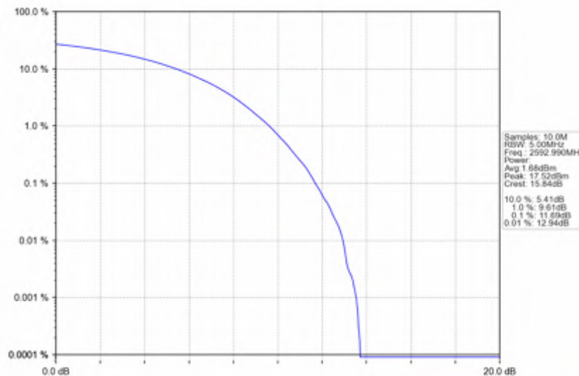
n41_30kHz_SISO_NTNV_80MHz_CP-OFDM_256_QAM_2592.99MHz_Outer_Full
