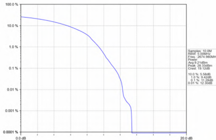
n41_30kHz_SISO_NTNV_30MHz_DFT-s-OFDM 256 QAM_2674.98MHz_Outer_Full
