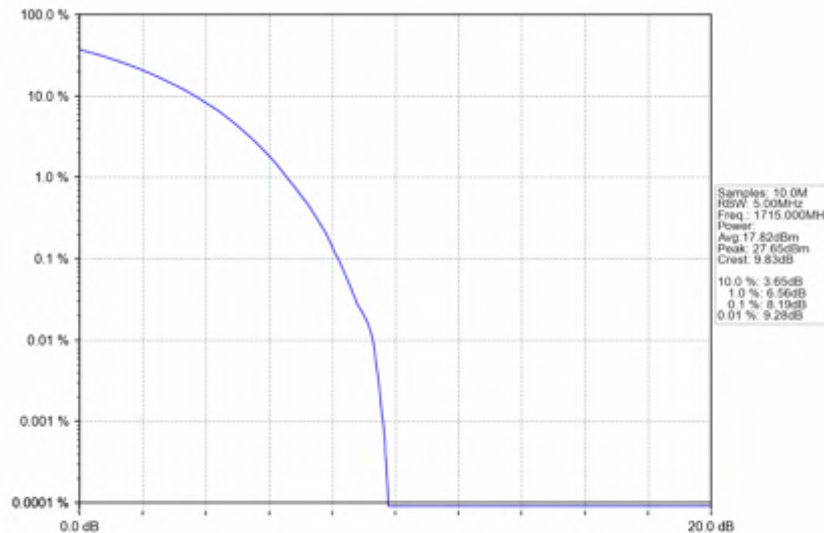
n66_15kHz_SISO_NTNV_10MHz_CP-OFDM 64 QAM_1715MHz_Outer_Full
