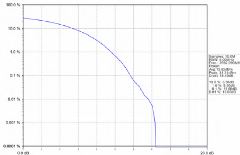
n41_30kHz_SISO_NTNV_15MHz_CP-OFDM_16_QAM_2592.99MHz_Outer_Full
