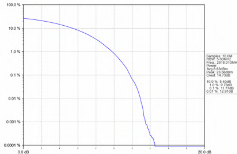
n41_30kHz_SISO_NTNV_40MHz_CP-OFDM_16_QAM_2516.01MHz_Outer_Full
