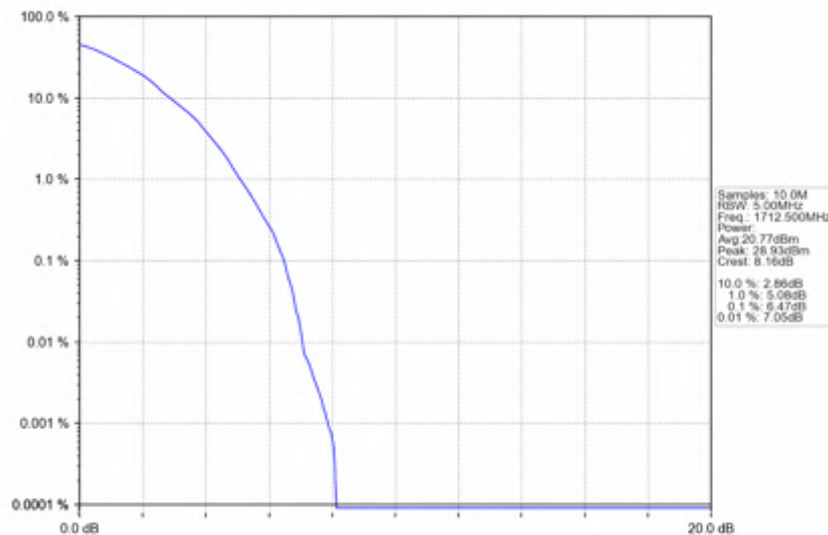
n66_15kHz_SISO_NTNV_5MHz_DFT-s-OFDM_64_QAM_1712.5MHz_Outer_Full
