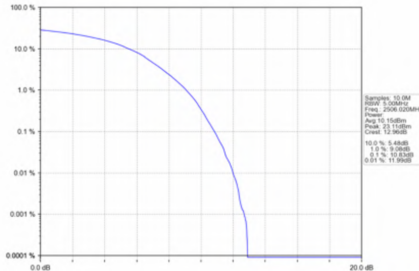
n41_30kHz_SISO_NTNV_20MHz_DFT-s-OFDM_256_QAM_2506.02MHz_Outer_Full
