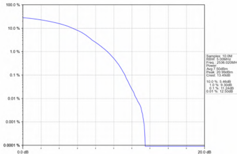
n41_30kHz_SISO_NTNV_80MHz_DFT-s-OFDM QPSK_2536.02MHz_Outer_Full
