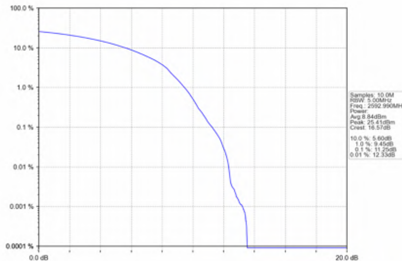
n41_30kHz_SISO_NTNV_30MHz_DFT-s-OFDM_256_QAM_2592.99MHz_Outer_Full
