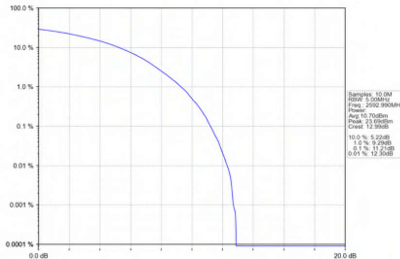
n41_30kHz_SISO_NTNV_30MHz_CP-OFDM QPSK_2592.99MHz_Outer_Full
