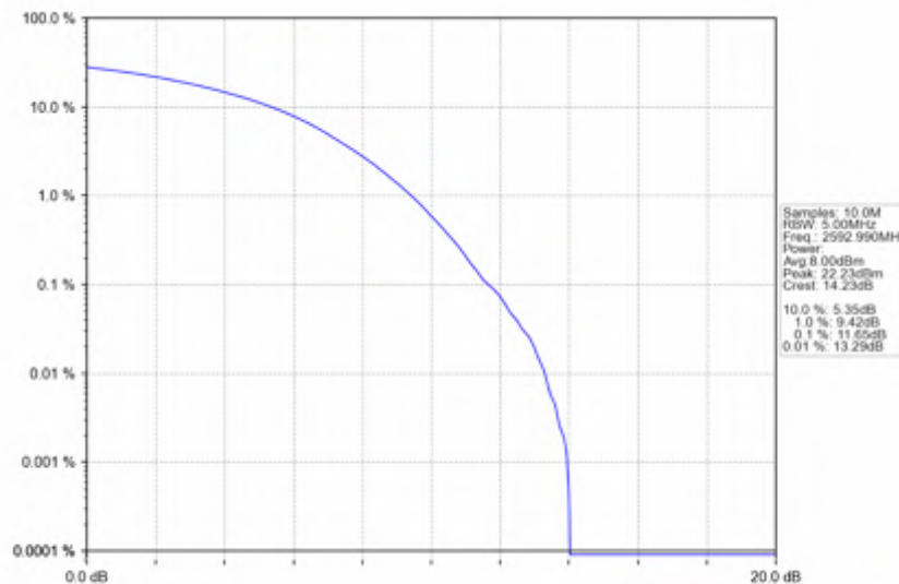
n41_30kHz_SISO_NTNV_50MHz_CP-OFDM_16_QAM_2592.99MHz_Outer_Full
