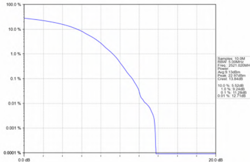
n41_30kHz_SISO_NTNV_50MHz_DFT-s-OFDM_16_QAM_2521.02MHz_Outer_Full
