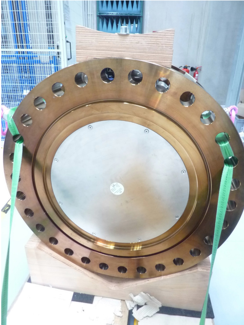
EUT view 4
