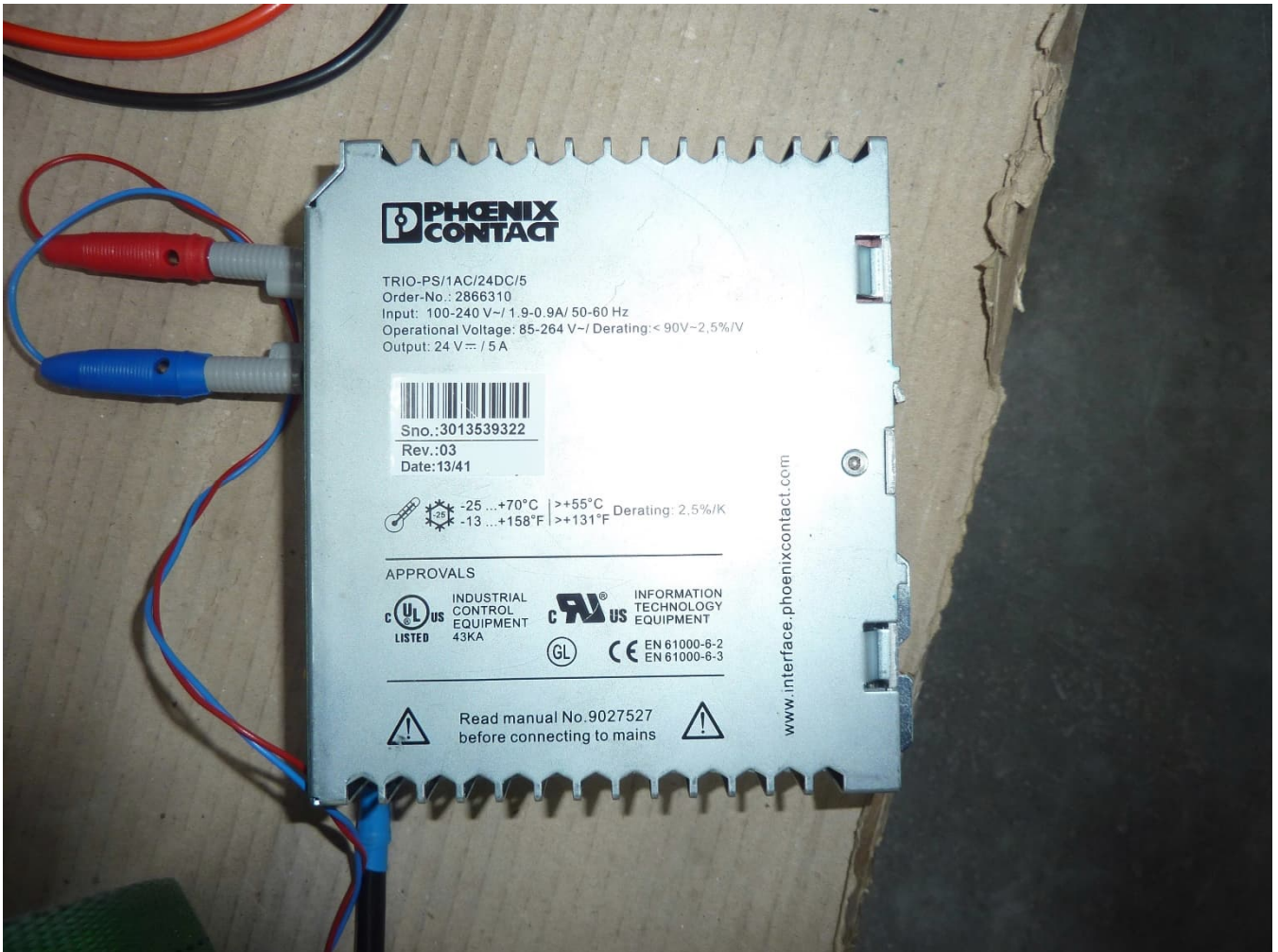
AC Adapter used for conducted emission measurement
