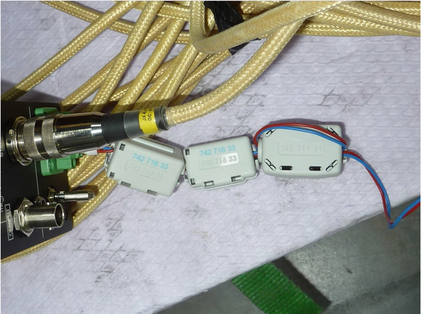
Three ferrites at DC supply control unit
