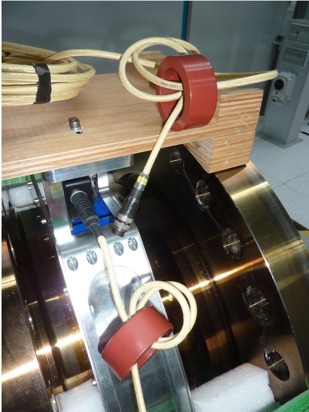
Ferrite cokes with 3 turns at connection cable startor control unit.
