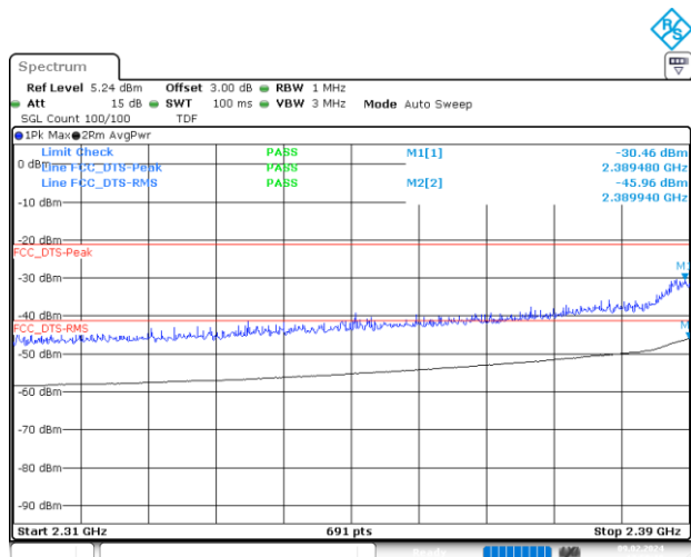
BE-R-LOW, MIMO-A, 802.11n20-HT8, Ch1
