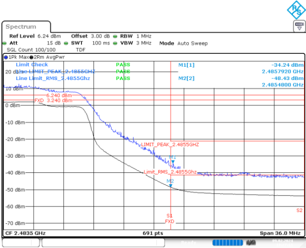
BE-R-HIGH, MIMO-A, 802.11n40-HT8, Ch10
