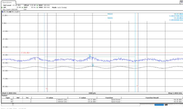
BE-R-HIGH-2MHz, MIMO-B, 802.11n40-HT8, Ch9
