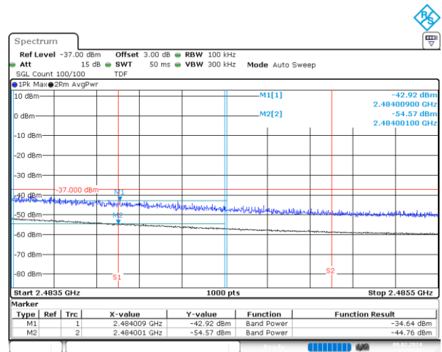
BE-R-HIGH-2MHz, MIMO-A, 802.11ax20-HE0, Ch12
