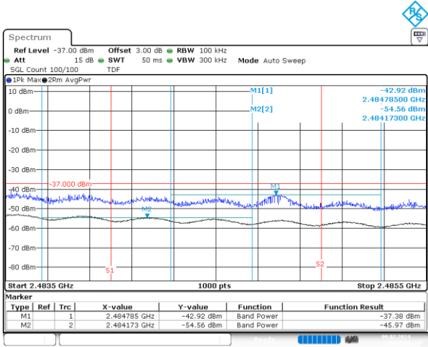
BE-R-HIGH-2MHz, MIMO-A, 802.11n40-HT8, Ch10
