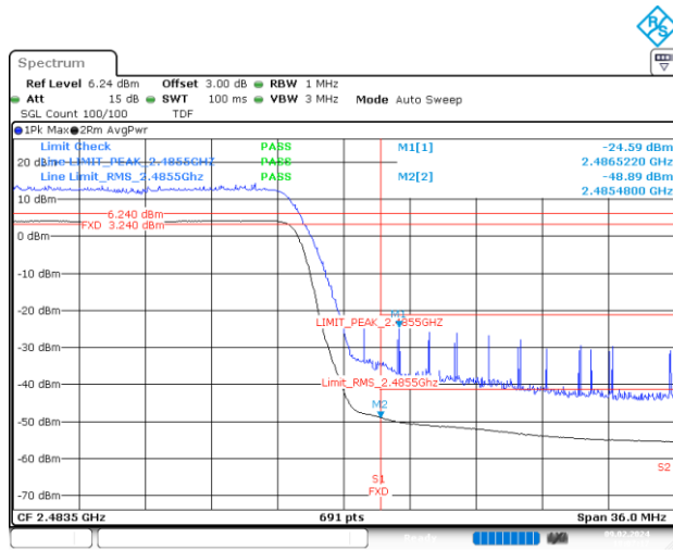
BE-R-HIGH, MIMO-A, 802.11n20-HT8, Ch13
