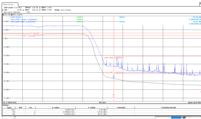
BE-R-HIGH, MIMO-B, 802.11n20-HT8, Ch13
