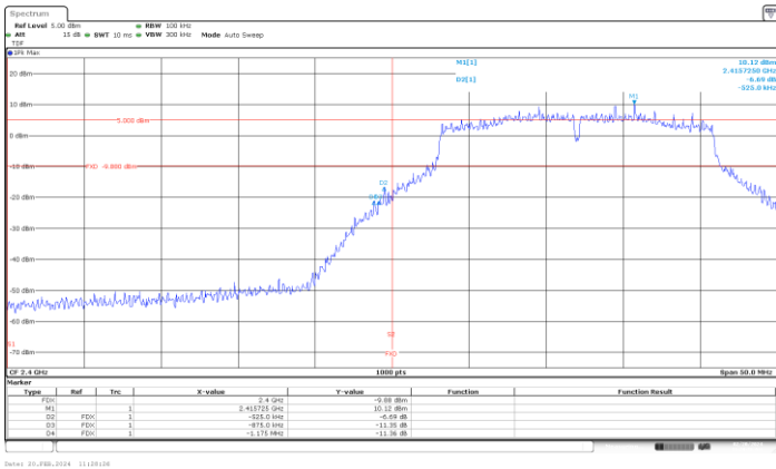
BE-NR, MIMO-B, 802.11n20-HT8 Ch1
