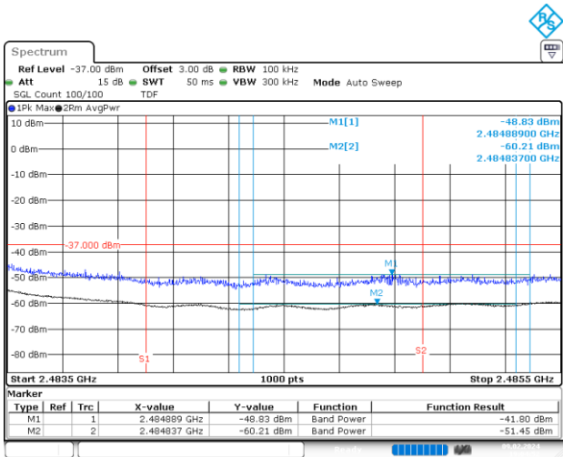
BE-R-HIGH-2MHz, MIMO-A, 802.11n40-HT8, Ch11
