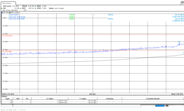
BE-R-LOW, MIMO-B, 802.11n20-HT8, Ch1
