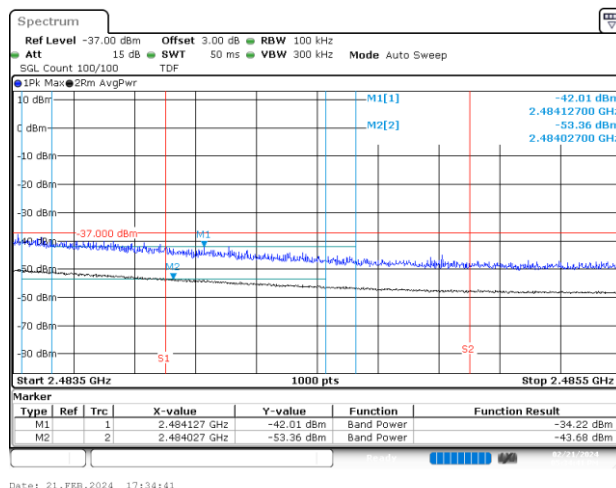
BE-R-HIGH-2MHz, SISO-B, 802.11ax20-HE0, Ch12
