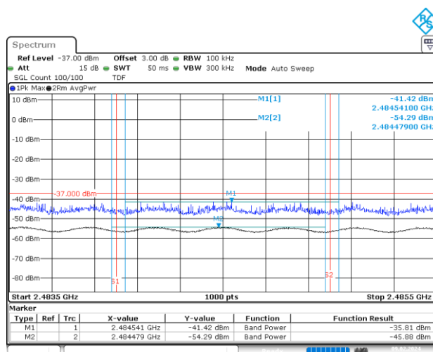
BE-R-HIGH-2MHz, MIMO-A, 802.11n20-HT8, Ch11
