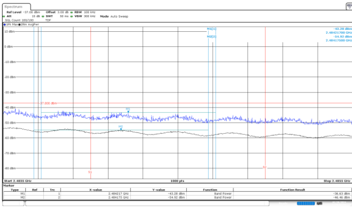
BE-R-HIGH-2MHz, MIMO-B, 802.11n40-HT8, Ch10
