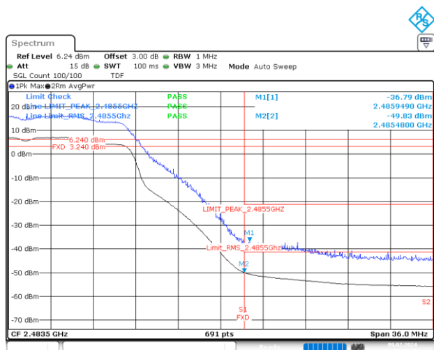
BE-R-HIGH, MIMO-A, 802.11n20-HT8, Ch12
