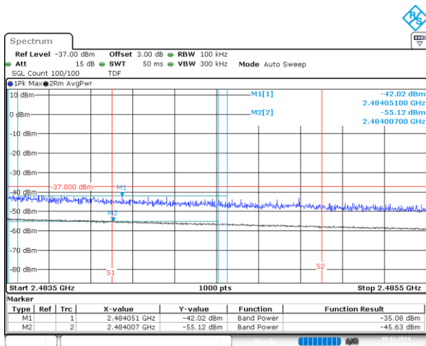
BE-R-HIGH-2MHz, MIMO-A, 802.11ax40-HE0, Ch10
