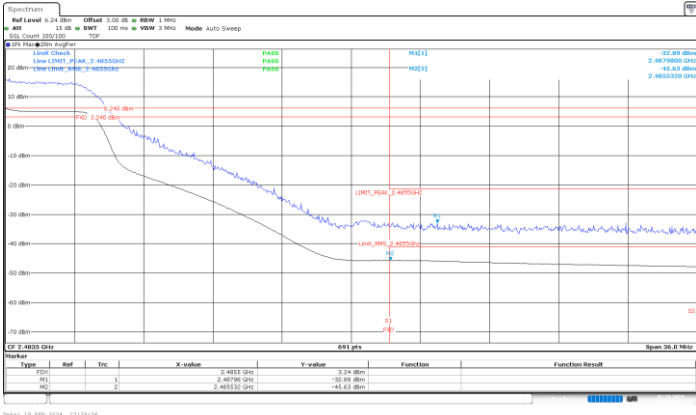
BE-R-HIGH, MIMO-B, 802.11n40-HT8, Ch9
