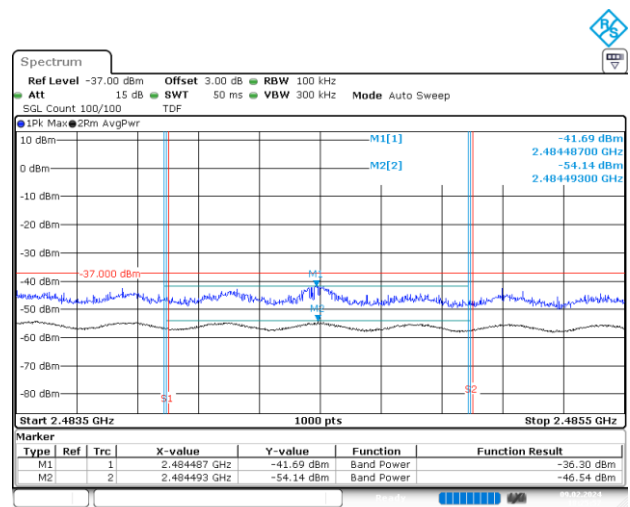
BE-R-HIGH-2MHz, MIMO-A, 802.11n40-HT8, Ch9
