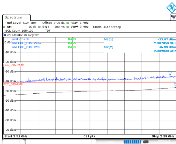
BE-R-LOW, MIMO-A, 802.11n40-HT8, Ch3
