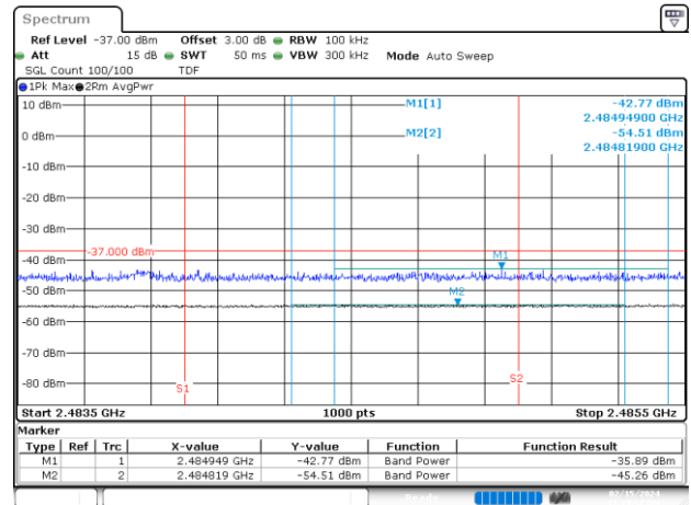
BE-R-HIGH-2MHz, SISO-B, 802.11ax40-HE0, Ch9
