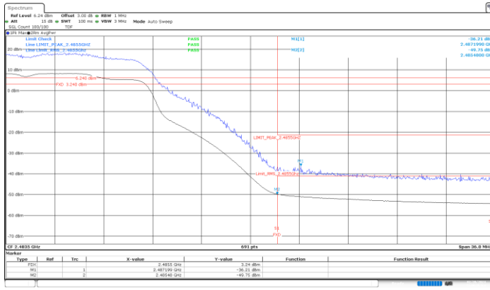
BE-R-HIGH, MIMO-B, 802.11n20-HT8, Ch12
