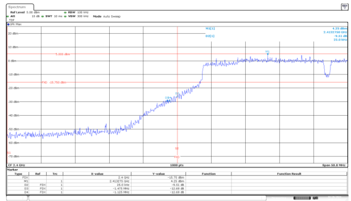
BE-NR, MIMO-B, 802.11n40-HT8, Ch3
