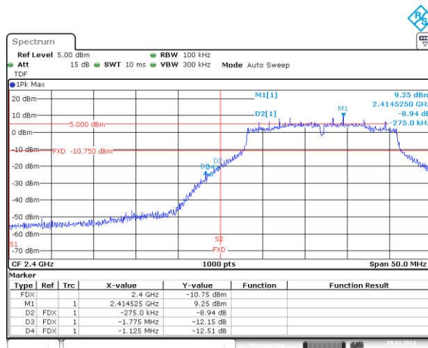
BE-NR, MIMO-A, 802.11n20-HT8 Ch1
