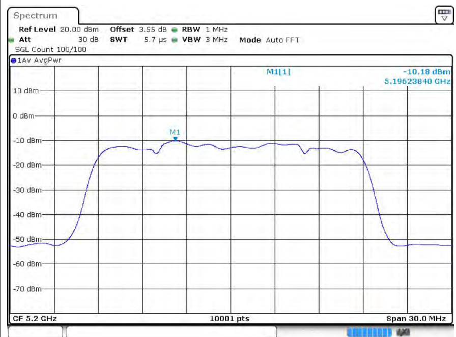
PSD n20 5200MHz Ant2
