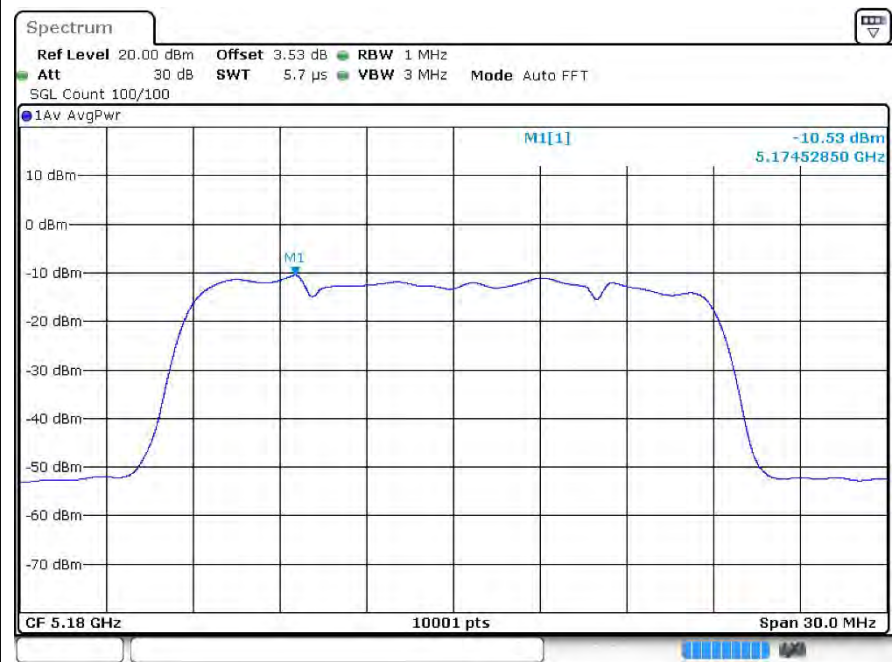
PSD n20 5180MHz Ant2
