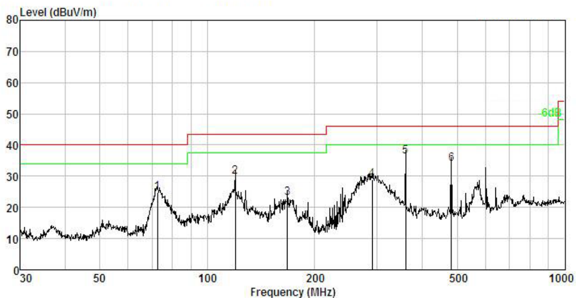
Test plot for Horizontal: Mode: GFSK (2441MHz)
