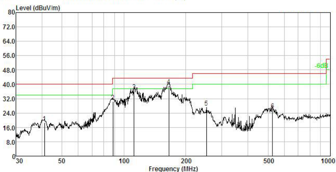
Test plot for Horizontal: Mode: GFSK (2402MHz)
