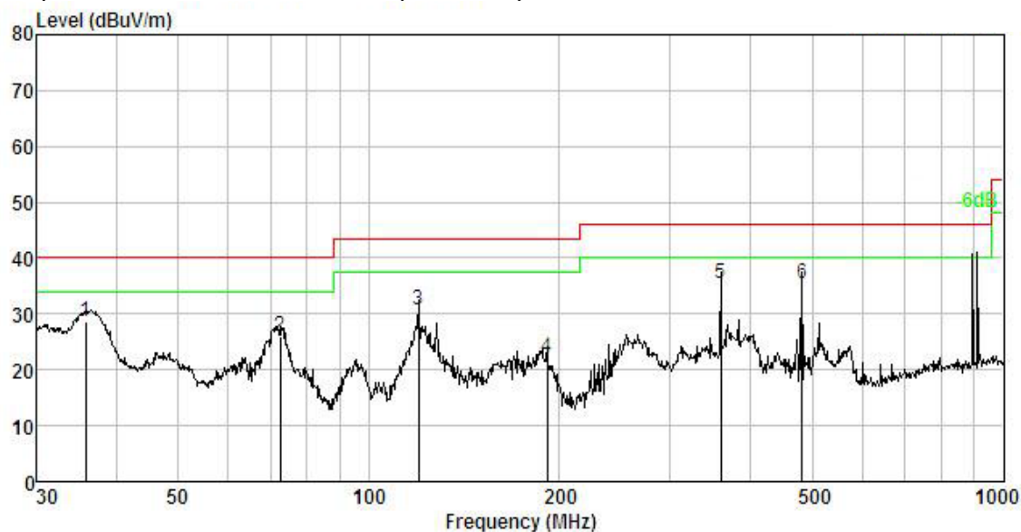
Test plot for Vertical: Mode: GFSK (2480MHz)
