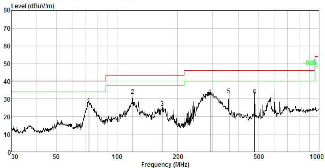
Test plot for Horizontal: Mode: GFSK (2480MHz)
