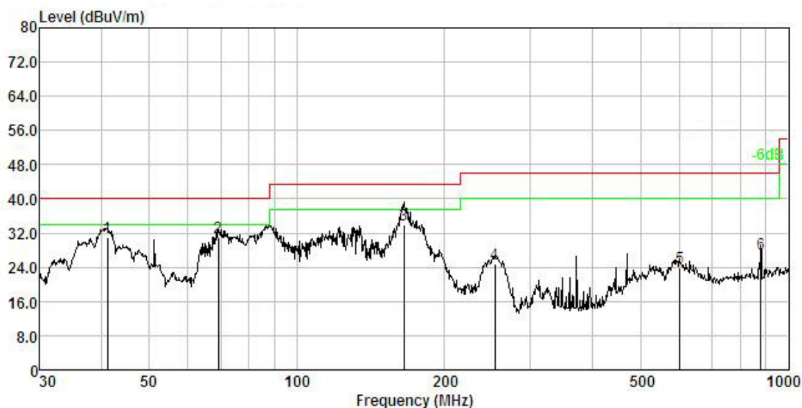
Test plot for Vertical: Mode: GFSK (2402MHz)
