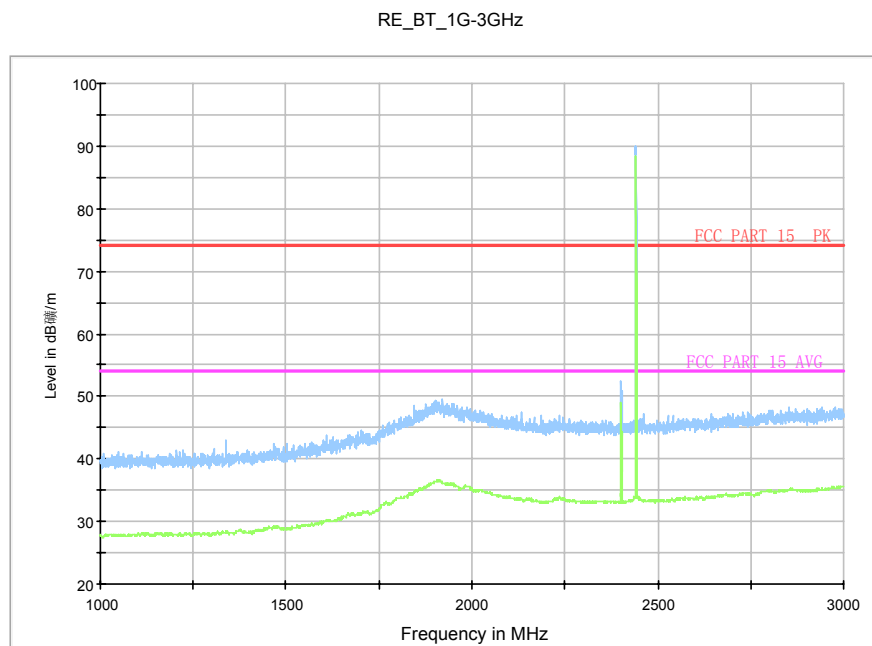
Fig.71. Radiated emission: \pi/4 DQPSK, Channel 39, 1 GHz - 3 GHz
