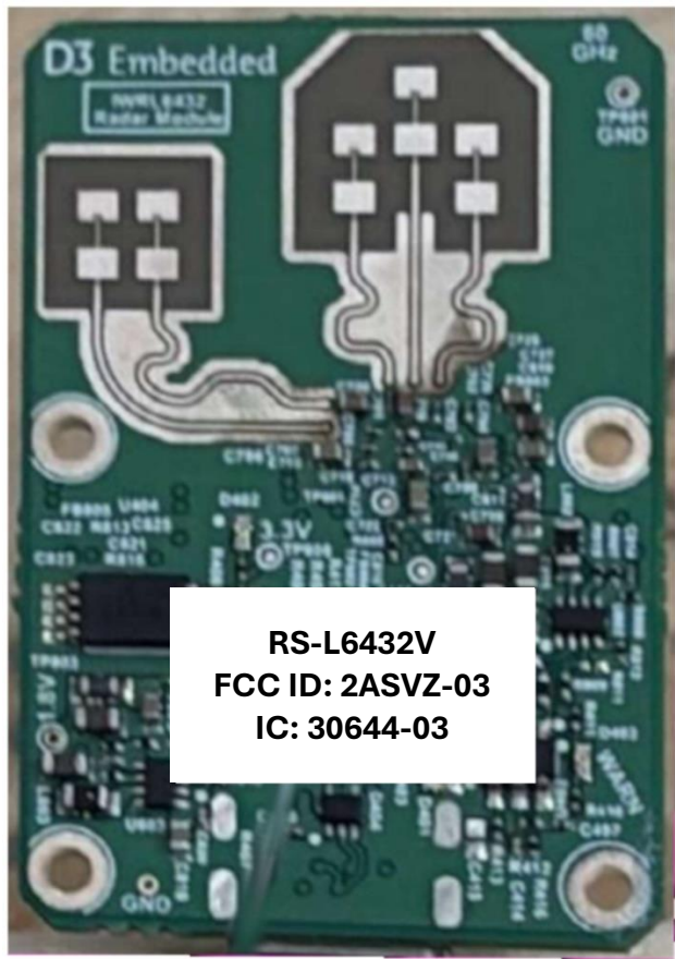
RS-L6432V variant
