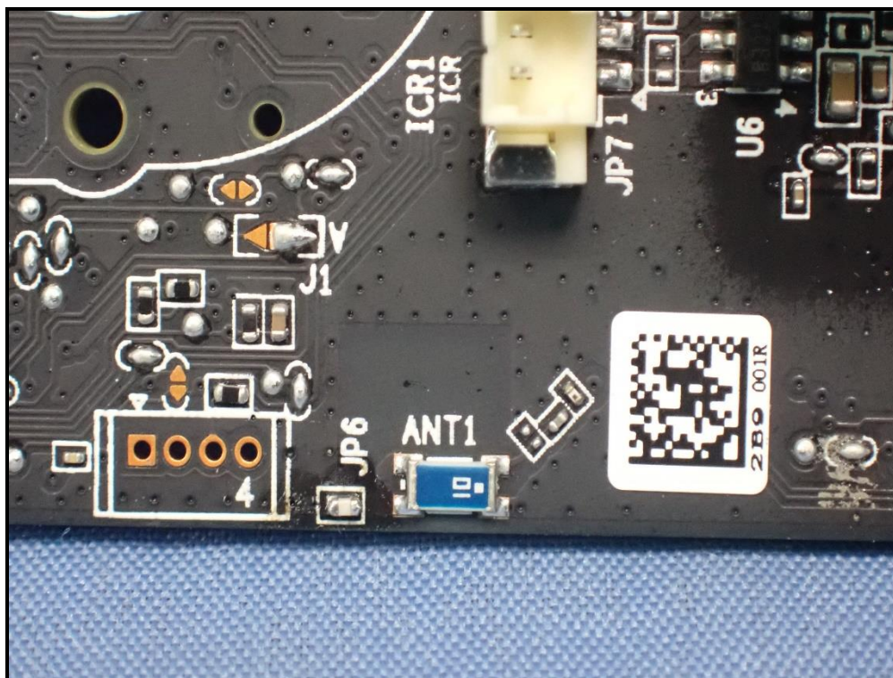
Bluetooth Antenna
