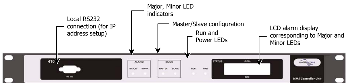
Figure 4-18. MobileAccess 410 Front Panel
