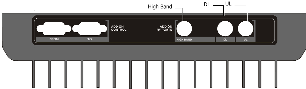
Figure 4-8. RHU 1200 Rear Panel
