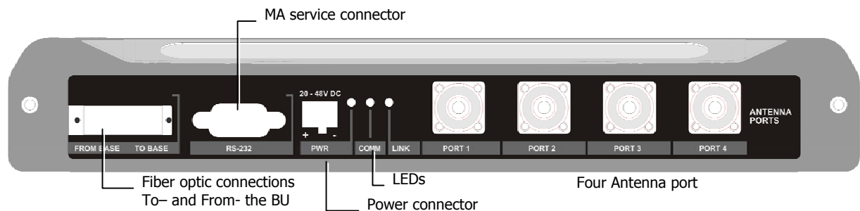
Figure 4-5. RU 2000 Front Panel
