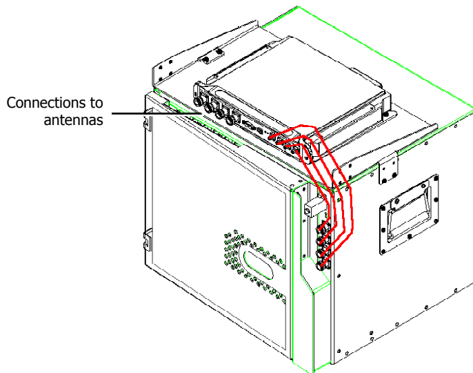
Figure 3-12. Illustration of RC Antenna port connections
