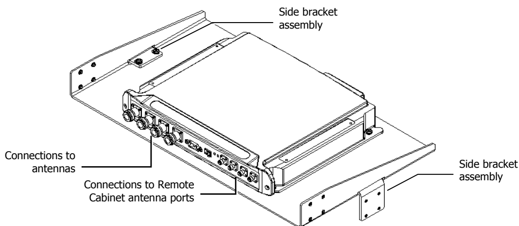
Figure 3-10. MA 850 Rack Installation
