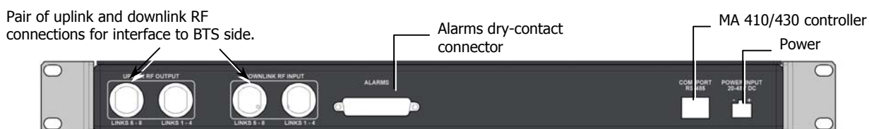
Figure 4-17. MA BU Rear Panel (RF Connections)
