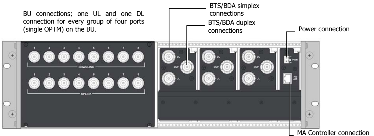
Figure 4-13. RIU Rear Panel showing the RF Connection
