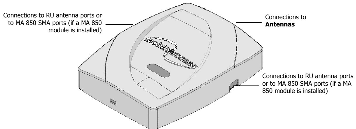
Figure 3-14. 2000 Lite System coax connections
