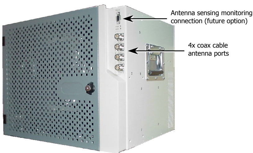
Figure 4-1. RC 2000 Closed Cabinet View
