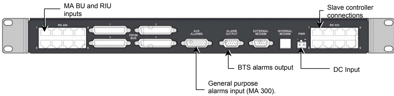
Figure 4-20. MobileAccess 410/430 Rear Panel
