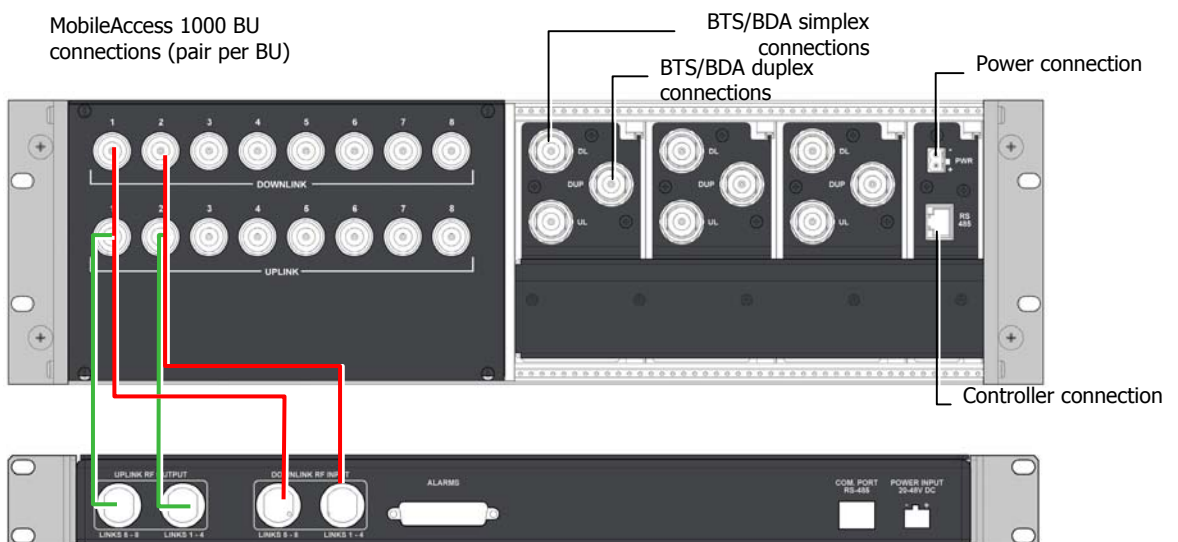
Figure 4-14. RIU Rear Panel showing the RF Connection
