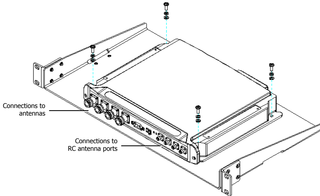
Figure 3-13. MA 850 to Bracket Installation
