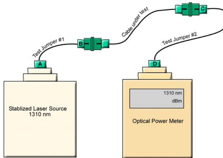
Figure 5-3. Connecting CUT
