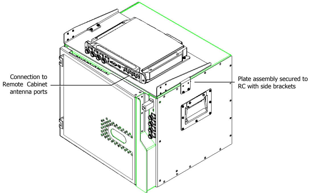
Figure 3-11. Illustration of MA 850 Mounted on MA 2000 RC
