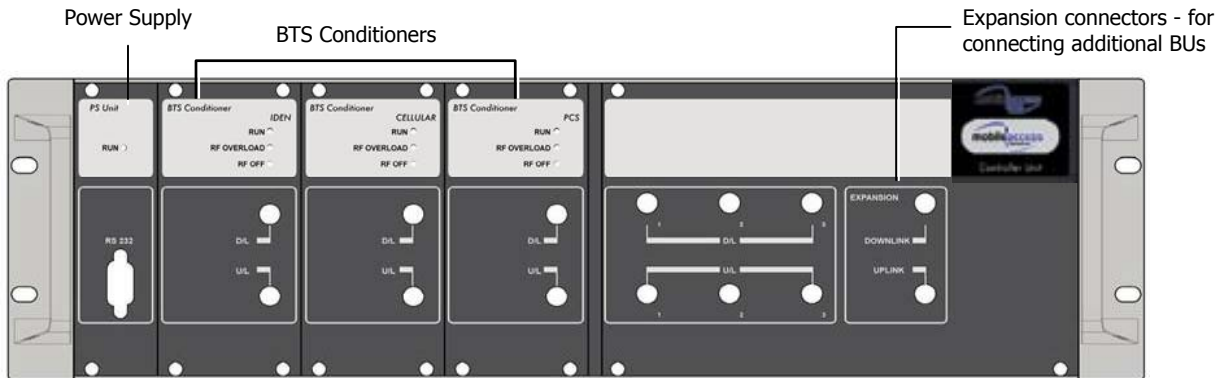
Figure 4-12. RIU Front Panel
