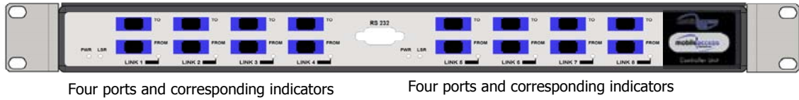
Figure 4-15. Eight-Port MA BU Front Panel
