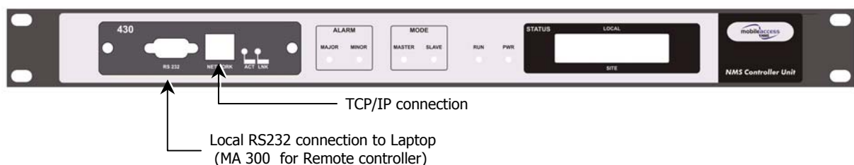
Figure 4-19. MobileAccess 430 Front Panel
