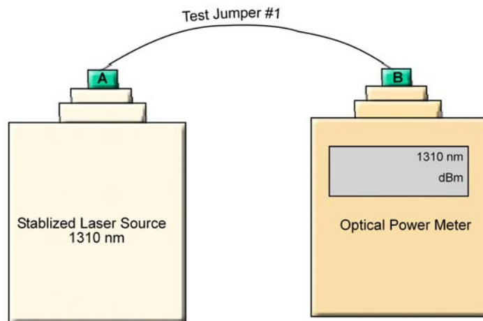
Figure 5-1. Set Up
