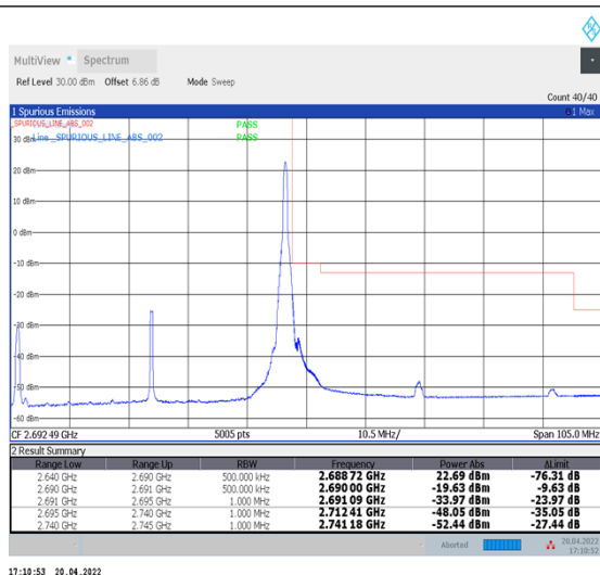
1-N41--30-50-H-2-DFT-PI2BPSK-Edge_1RB_Right-1@132-Ant1-PASS-see graph
