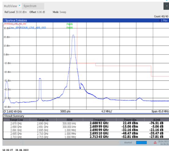
1-N41--30-20-H-2-DFT-PI2BPSK-Edge_1RB_Right-1@50-Ant1-PASS-see graph
