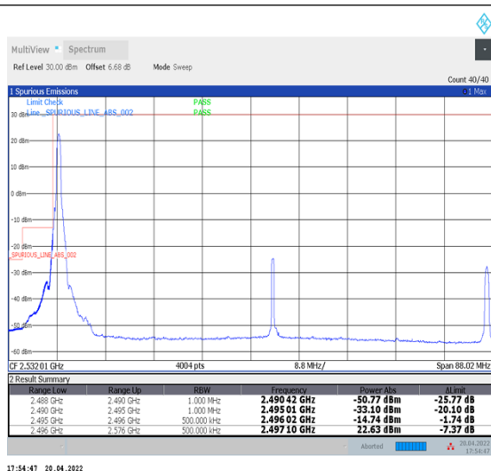
1-N41--30-80-L-1-DFT-PI2BPSK-Edge_1RB_Left-1@0-Ant1-PASS-see graph
