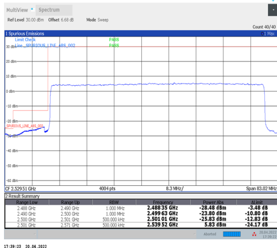
1-N41--30-70-L-3-DFT-PI2BPSK-Outer_Full-180@0-Ant1-PASS-see graph
