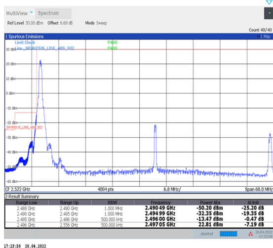
1-N41--30-60-L-4-CP-QPSK-Edge_1RB_Left-1@0-Ant1-PASS-see graph
