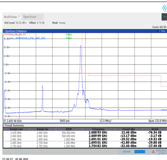
1-N41--30-60-H-2-DFT-PI2BPSK-Edge_1RB_Right-1@161-Ant1-PASS-see graph
