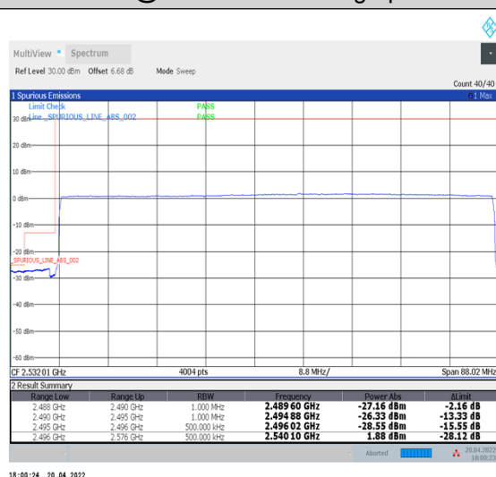
1-N41--30-80-L-6-CP-QPSK-Outer_Full-217@0-Ant1-PASS-see graph
