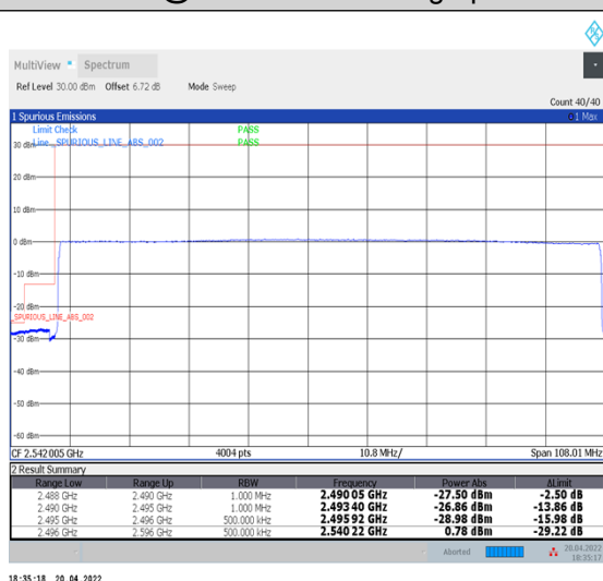
1-N41--30-100-L-6-CP-QPSK-Outer_Full-273@0-Ant1-PASS-see graph
