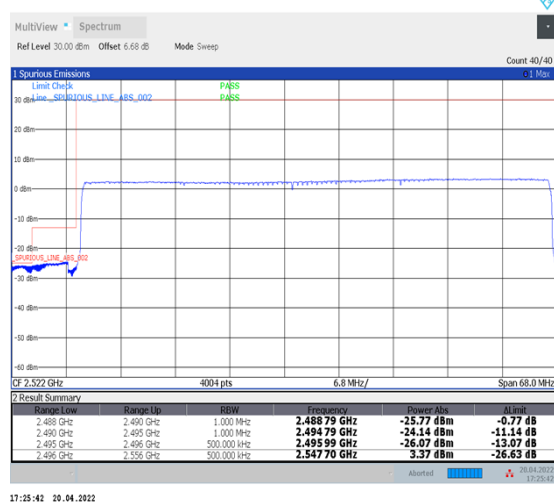
1-N41--30-60-L-6-CP-QPSK-Outer_Full-162@0-Ant1-PASS-see graph
