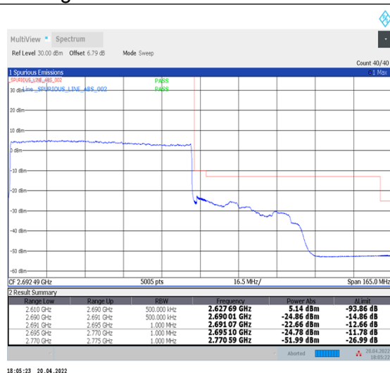
1-N41--30-80-H-3-DFT-PI2BPSK-Outer_Full-216@0-Ant1-PASS-see graph
