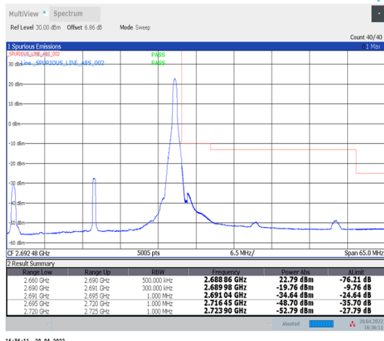
1-N41--30-30-H-2-DFT-PI2BPSK-Edge_1RB_Right-1@77-Ant1-PASS-see graph
