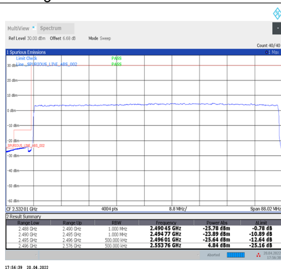
1-N41--30-80-L-3-DFT-PI2BPSK-Outer_Full-216@0-Ant1-PASS-see graph
