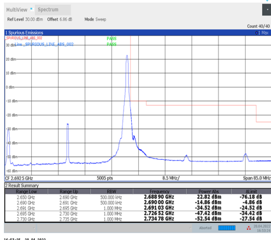
1-N41--30-40-H-2-DFT-PI2BPSK-Edge_1RB_Right-1@105-Ant1-PASS-see graph
