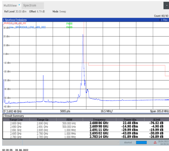
1-N41--30-90-H-2-DFT-PI2BPSK-Edge_1RB_Right-1@244-Ant1-PASS-see graph
