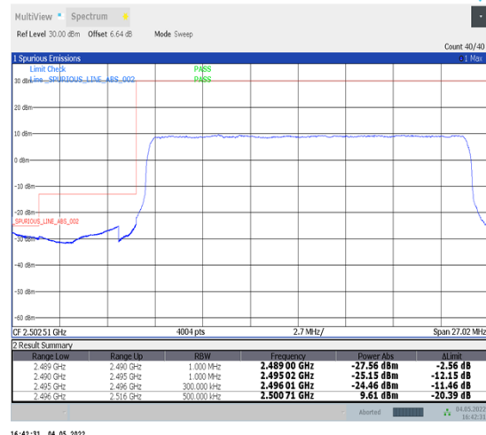
1-N41--30-20-L-3-DFT-PI2BPSK-Outer_Full-50@0-Ant1-PASS-see graph
