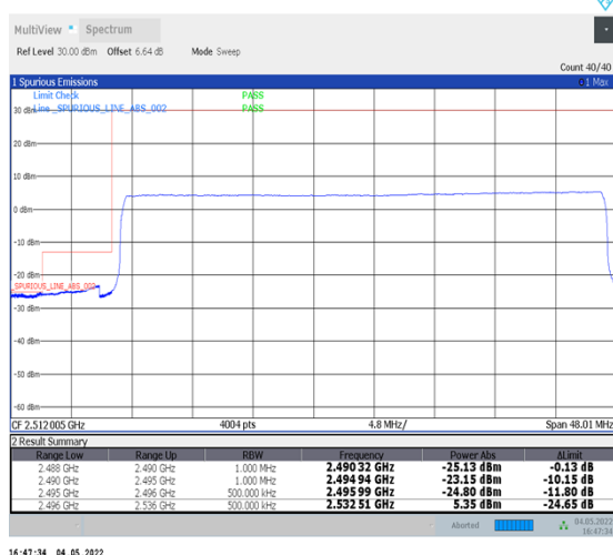
1-N41--30-40-L-6-CP-QPSK-Outer_Full-106@0-Ant1-PASS-see graph
