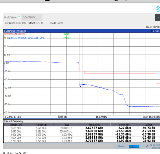
1-N41--30-80-H-6-CP-QPSK-Outer_Full-217@0-Ant1-PASS-see graph
