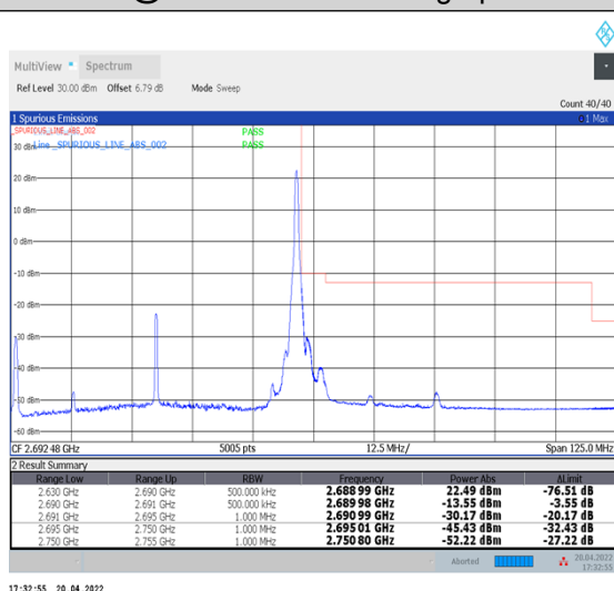
1-N41--30-60-H-5-CP-QPSK-Edge_1RB_Right-1@161-Ant1-PASS-see graph
