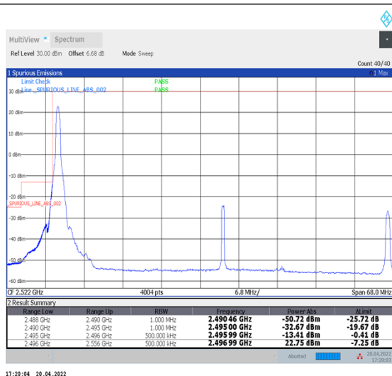
1-N41--30-60-L-1-DFT-PI2BPSK-Edge_1RB_Left-1@0-Ant1-PASS-see graph
