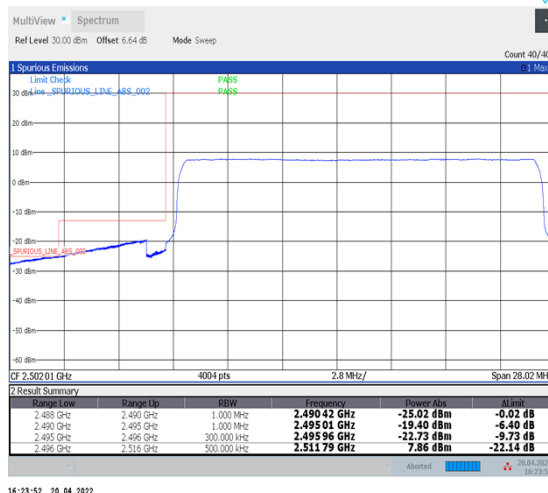
1-N41--30-20-L-6-CP-QPSK-Outer_Full-51@0-Ant1-PASS-see graph
