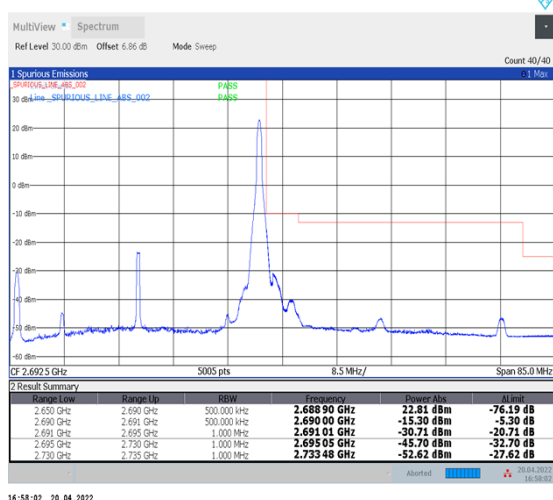
1-N41--30-40-H-5-CP-QPSK-Edge_1RB_Right-1@105-Ant1-PASS-see graph
