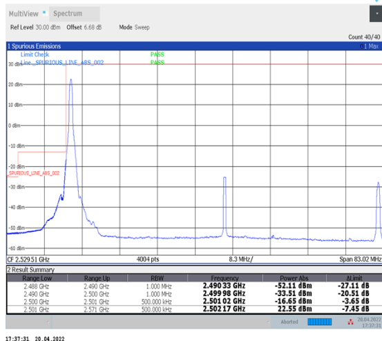
1-N41--30-70-L-1-DFT-PI2BPSK-Edge_1RB_Left-1@0-Ant1-PASS-see graph
