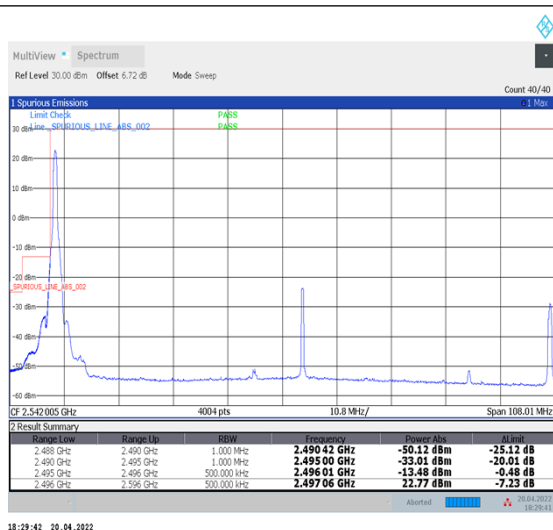
1-N41--30-100-L-1-DFT-PI2BPSK-Edge_1RB_Left-1@0-Ant1-PASS-see graph
