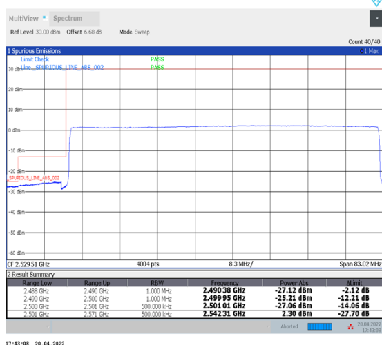
1-N41--30-70-L-6-CP-QPSK-Outer_Full-189@0-Ant1-PASS-see graph
