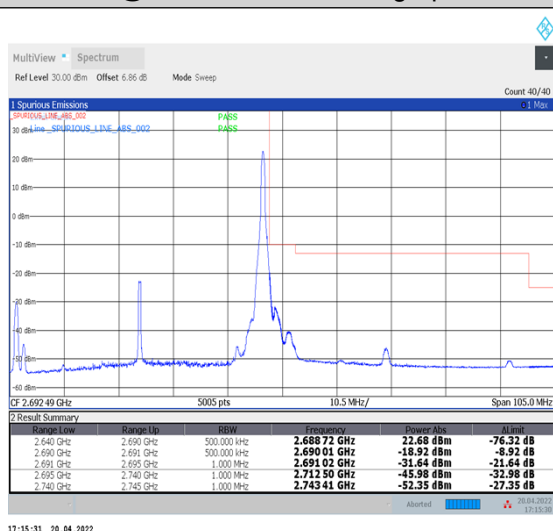
1-N41--30-50-H-5-CP-QPSK-Edge_1RB_Right-1@132-Ant1-PASS-see graph
