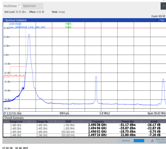
1-N41--30-50-L-1-DFT-PI2BPSK-Edge_1RB_Left-1@0-Ant1-PASS-see graph
