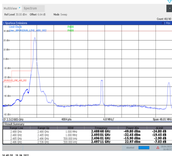
1-N41--30-40-L-4-CP-QPSK-Edge_1RB_Left-1@0-Ant1-PASS-see graph
