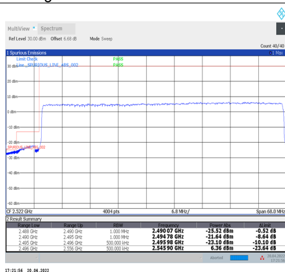
1-N41--30-60-L-3-DFT-PI2BPSK-Outer_Full-162@0-Ant1-PASS-see graph
