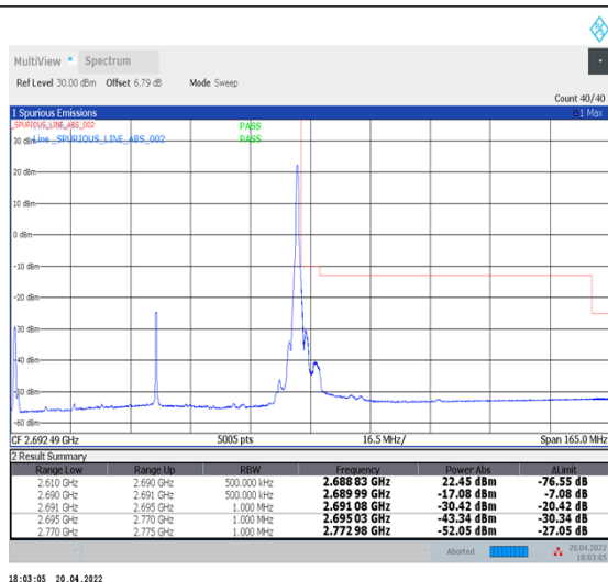
1-N41--30-80-H-2-DFT-PI2BPSK-Edge_1RB_Right-1@216-Ant1-PASS-see graph
