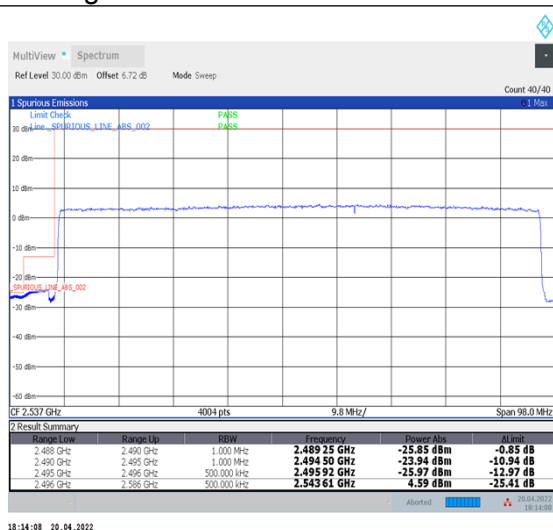
1-N41--30-90-L-3-DFT-PI2BPSK-Outer_Full-240@0-Ant1-PASS-see graph
