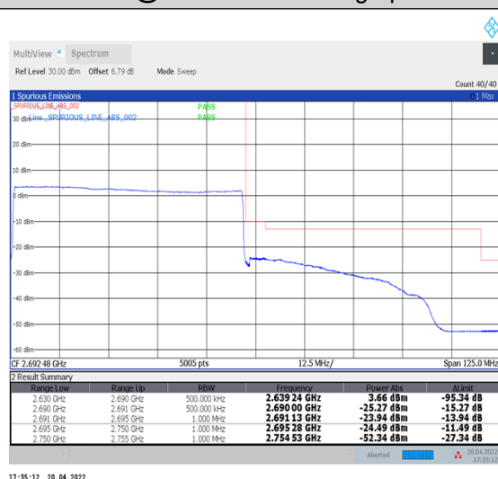
1-N41--30-60-H-6-CP-QPSK-Outer_Full-162@0-Ant1-PASS-see graph
