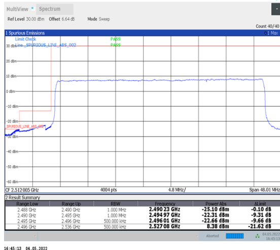
1-N41--30-40-L-3-DFT-PI2BPSK-Outer_Full-100@0-Ant1-PASS-see graph
