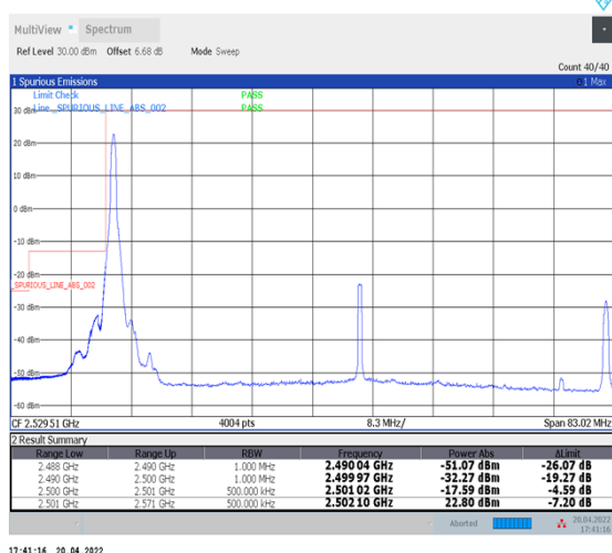
1-N41--30-70-L-4-CP-QPSK-Edge_1RB_Left-1@0-Ant1-PASS-see graph
