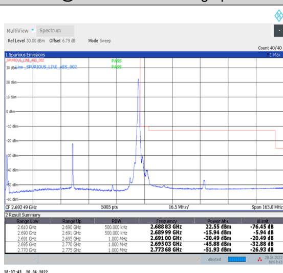
1-N41--30-80-H-5-CP-QPSK-Edge_1RB_Right-1@216-Ant1-PASS-see graph
