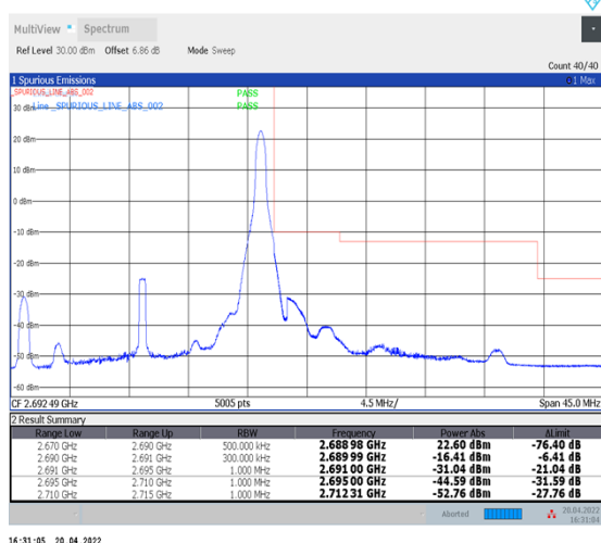
1-N41--30-20-H-5-CP-QPSK-Edge_1RB_Right-1@50-Ant1-PASS-see graph
