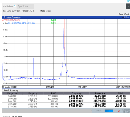
1-N41--30-90-H-5-CP-QPSK-Edge_1RB_Right-1@244-Ant1-PASS-see graph
