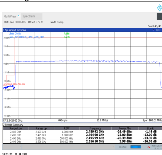
1-N41--30-100-L-3-DFT-PI2BPSK-Outer_Full-270@0-Ant1-PASS-see graph
