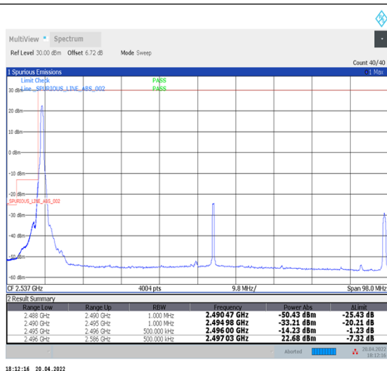
1-N41--30-90-L-1-DFT-PI2BPSK-Edge_1RB_Left-1@0-Ant1-PASS-see graph
