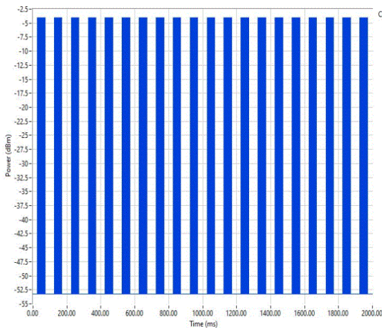
BLE/GFSK 2 Mbps Low Channel, 2402 MHz
