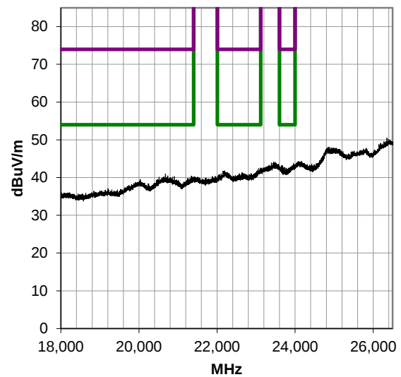
18000-26500 MHz, Run 77
