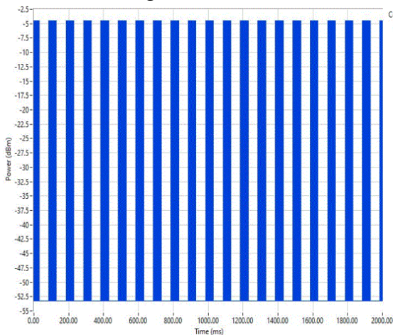
BLE/GFSK 2 Mbps Mid Channel, 2442 MHz
