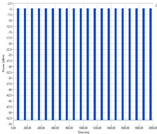
BLE/GFSK 1 Mbps Mid Channel, 2442 MHz
