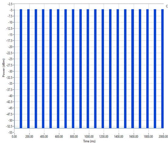
BLE/GFSK 1 Mbps High Channel, 2480 MHz
