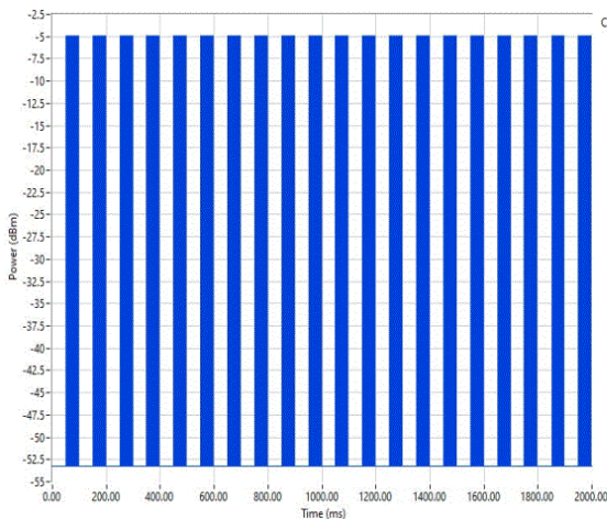
BLE/GFSK 2 Mbps High Channel, 2480 MHz
