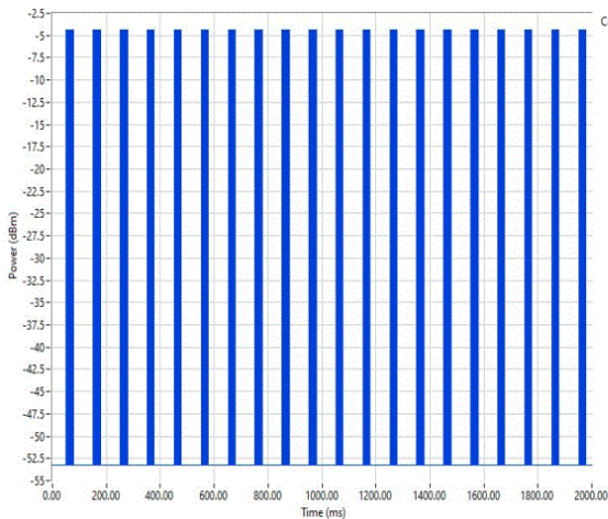
BLE/GFSK 1 Mbps Low Channel, 2402 MHz
