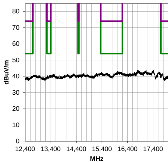
12400-18000 MHz, Run 58
