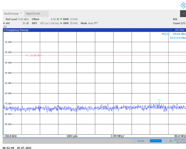
Band12-10MHz-QPSK-23035-1RB#0-Range2:0.15~30MHz
