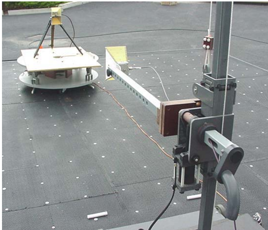
Substitution Horn antenna and Horn receive antenna
