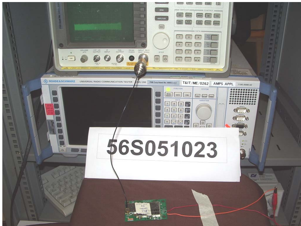
Average Frequency Dwell Time Test Setup MAXIMUM PEAK POWER TEST
