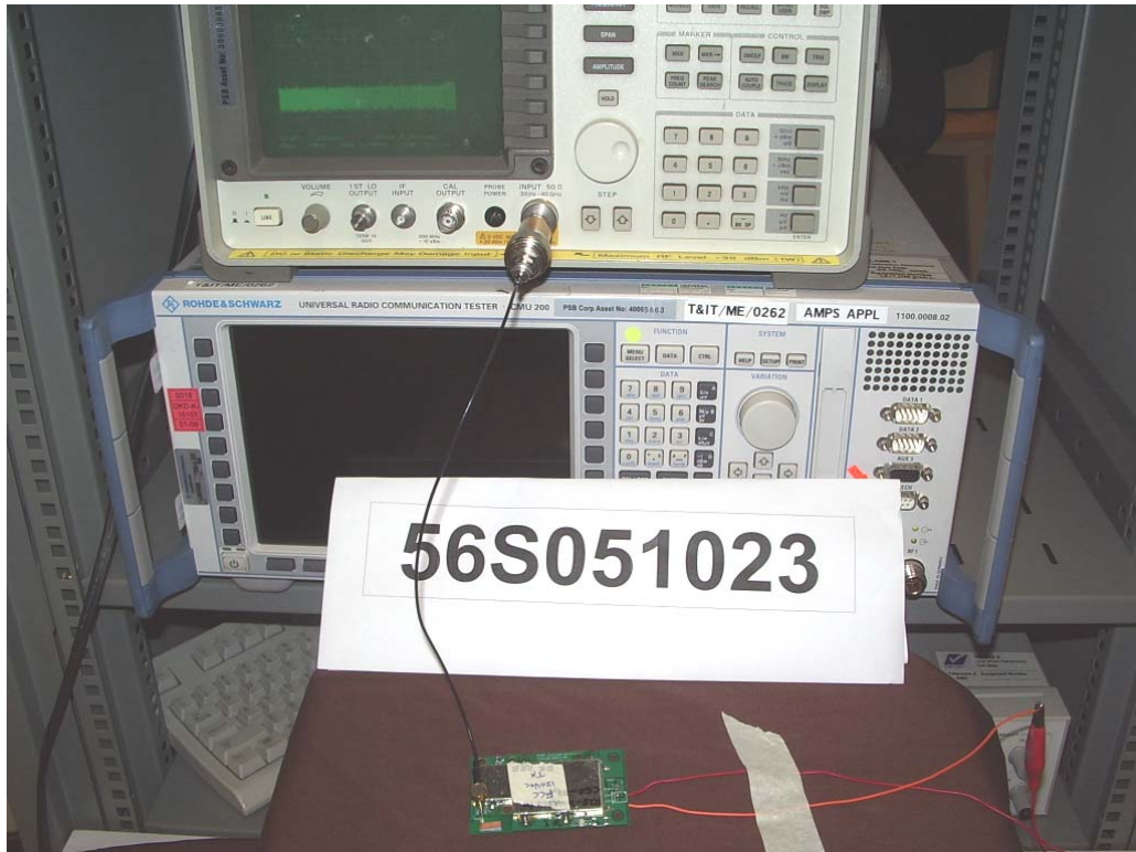
Peak Power Spectral Density Test Setup MAXIMUM PERMISSIBLE EXPOSURE (MPE) TEST
