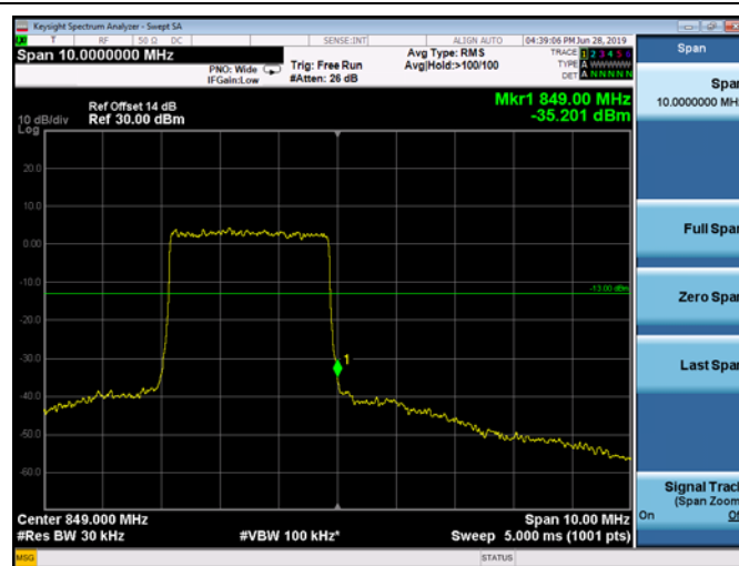
HighRange_FDD05_5MHz_846.5_OneRB _high_QPSK
