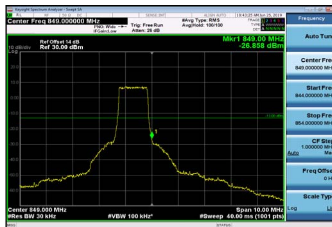
HighRange_FDD05_3MHz_847.5_OneRB _high_QPSK
