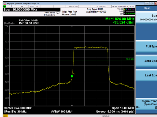
LowRange_FDD05_5MHz_826.5_OneRB _low_QPSK
