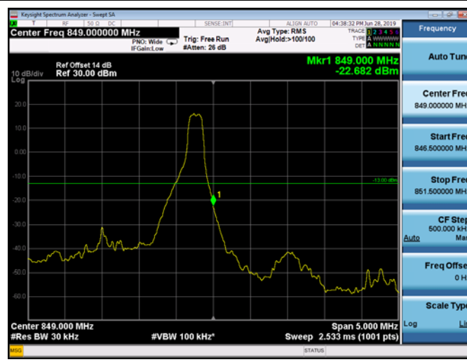
HighRange_FDD05_3MHz_847.5_OneRB _high_QPSK
