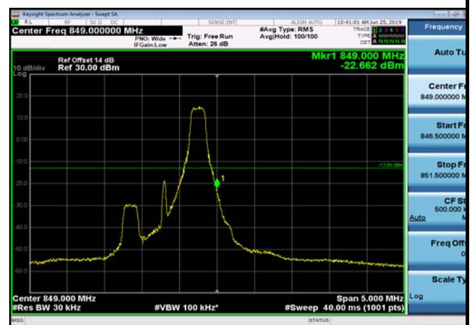
HighRange_FDD05_1.4MHz_848.3_fullRB _High_Q16
