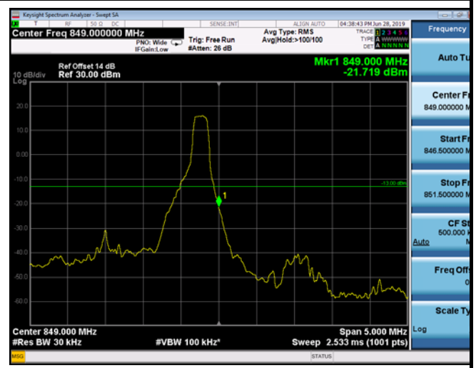
HighRange_FDD05_3MHz_847.5_OneRB _high_Q16
