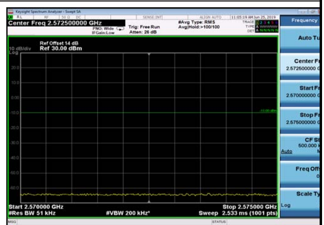
FDD07_10MHz_2505_Q16_fullRB_ExtraBand s_Range_2570~2575
