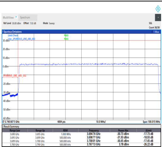
1-N78-3700-3800--30-90-L-3-DFT-PI2BPSK-Outer_Full-243@0-Ant1-1--PASS-see graph
