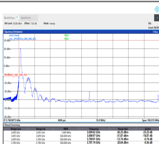
1-N78-3700-3800--30-90-L-4-CP-QPSK-Edge_1RB_Left-1@0-Ant1-1--PASS-see graph
