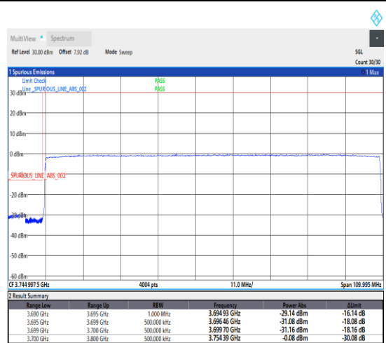
1-N78-3700-3800--30-100-L-6-CP-QPSK-Outer_Full-273@0-Ant1-1--PASS-see graph
