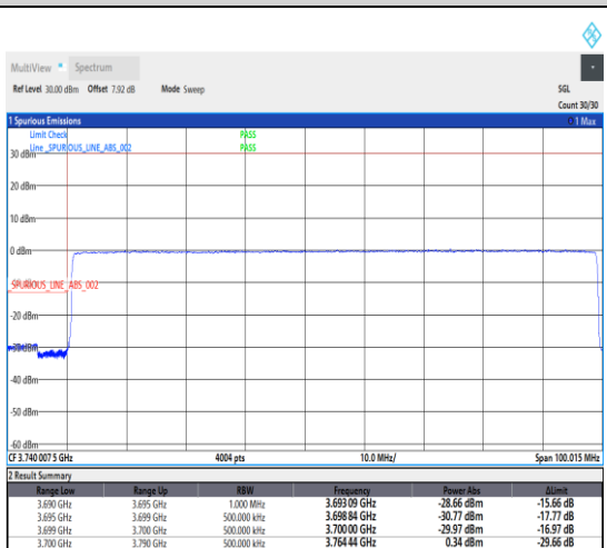
1-N78-3700-3800--30-90-L-6-CP-QPSK-Outer_Full-245@0-Ant1-1--PASS-see graph
