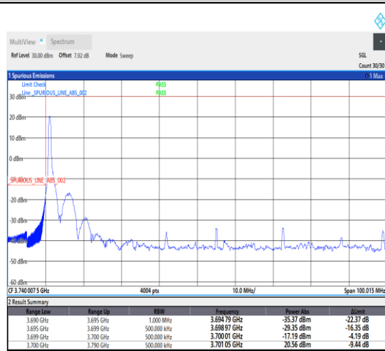
1-N78-3700-3800--30-90-L-1-DFT-PI2BPSK-Edge_1RB_Left-1@0-Ant1-1--PASS-see graph
