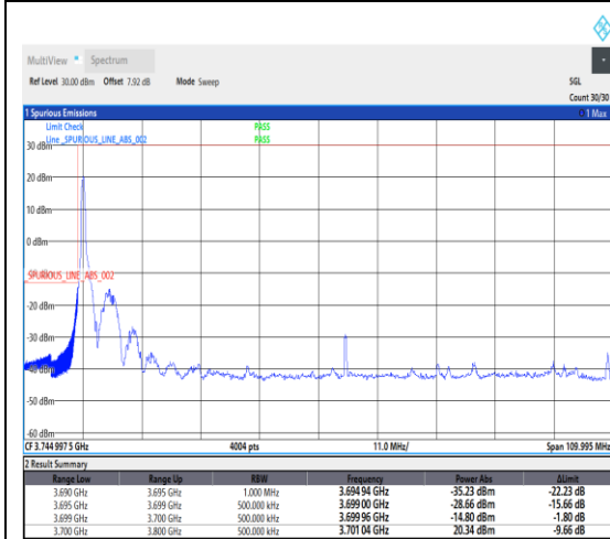
1-N78-3700-3800--30-100-L-4-CP-QPSK-Edge_1RB_Left-1@0-Ant1-1--PASS-see graph
