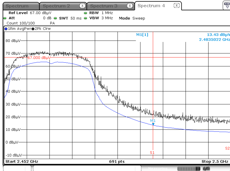
Radiated Restricted Band Edges plot – Average Result (802.11g , 6 Mbps, Ch.11, Z-H) (Integration method Used)
