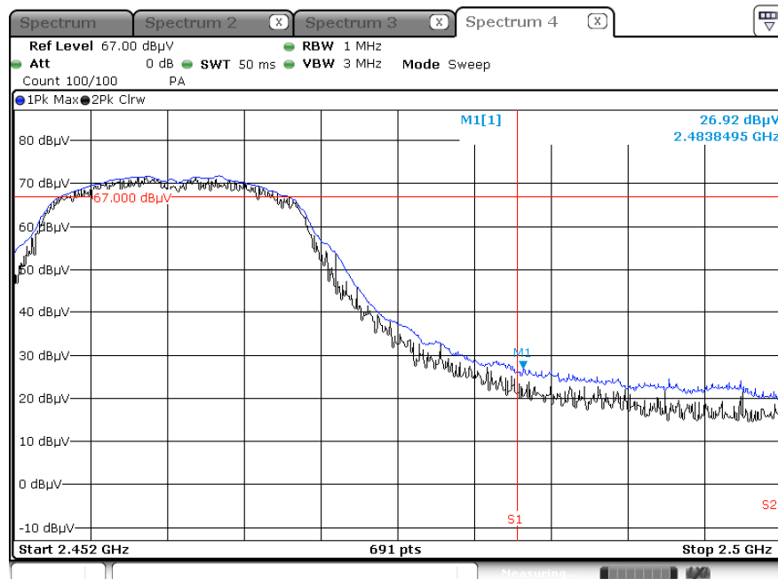
Radiated Restricted Band Edges plot – Peak Result (802.11g , 6 Mbps, Ch.11, Z-H)
