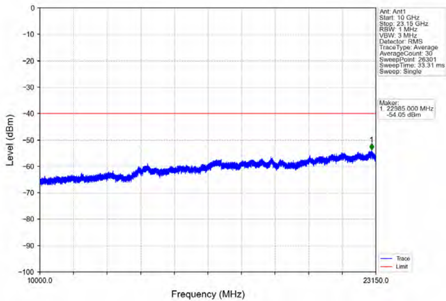
Band30_10MHz_64QAM_HCH_2310MHz_RB_1_49_NTNV
