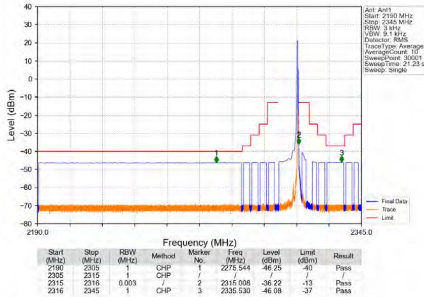
Band30_5MHz_16QAM_HCH_2312.5MHz_RB_1_24_NTNV
