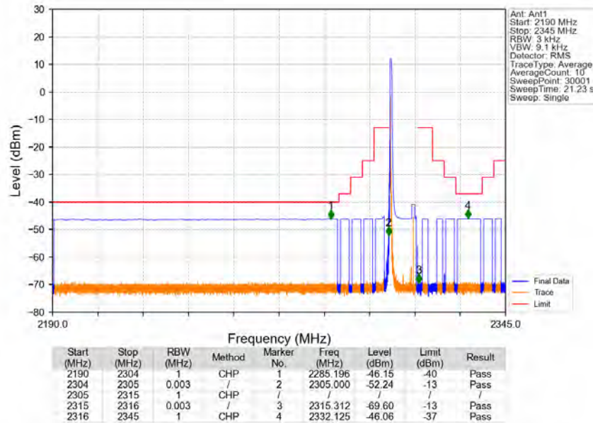
Band30_10MHz_64QAM_MCH_2310MHz_RB_1_0_NTNV
