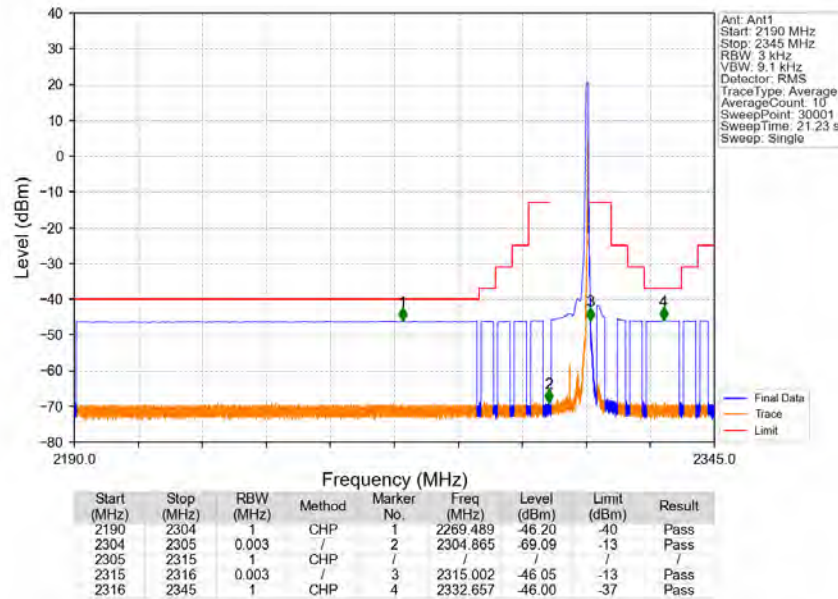
Band30_10MHz_16QAM_HCH_2310MHz_RB_50_0_NTNV
