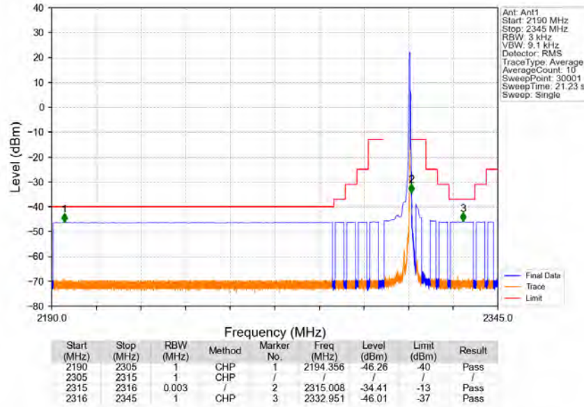
Band30_5MHz_QPSK_HCH_2312.5MHz_RB_25_0_NTNV
