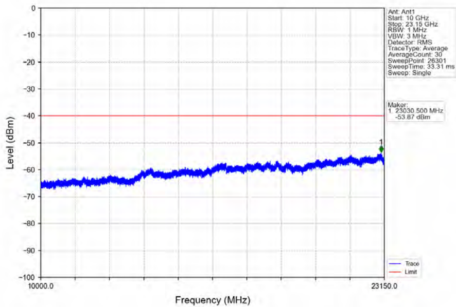
Band30_10MHz_64QAM_LCH_2310MHz_RB_50_0_NTNV
