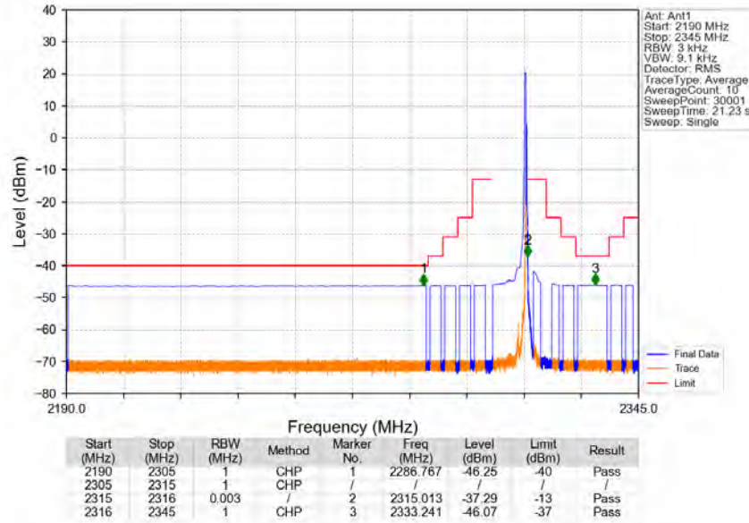
Band30_5MHz_64QAM_HCH_2312.5MHz_RB_25_0_NTNV
