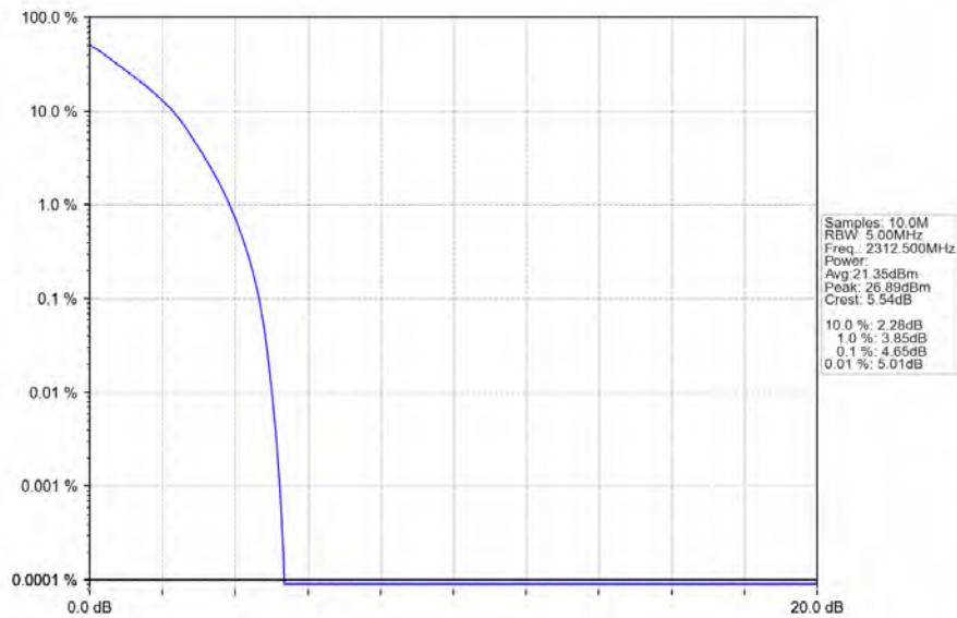
Band30 5MHz_QPSK_HCH_2312.5MHz_RB_25_0_NTNV
