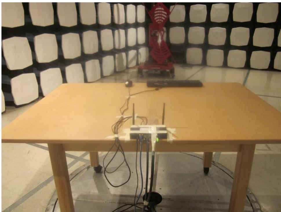
Figure B.2.4 - Radiated Emissions Test Setup - Rear View; 30 MHz-1000 MHz; PoE PS
