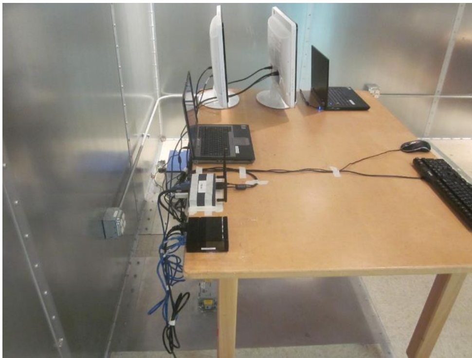
Figure B.6.6 - Conducted Emissions Test Setup - Side View 2; PoE PS
