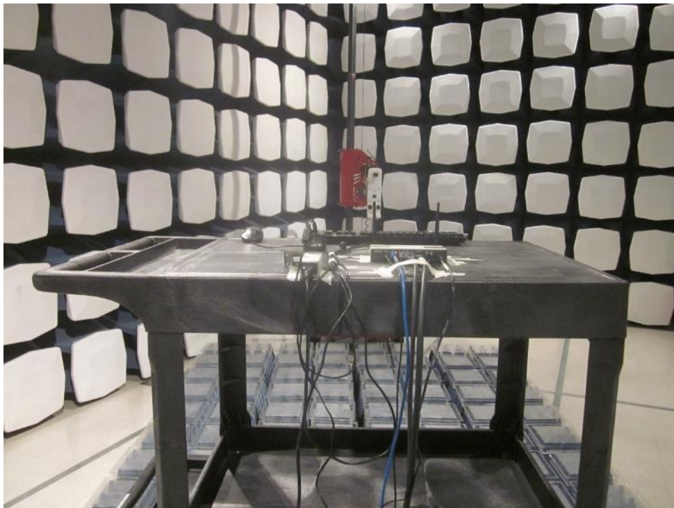
Figure B.4.2 - Radiated Emissions Test Setup - Rear View; 18 GHz-40 GHz
