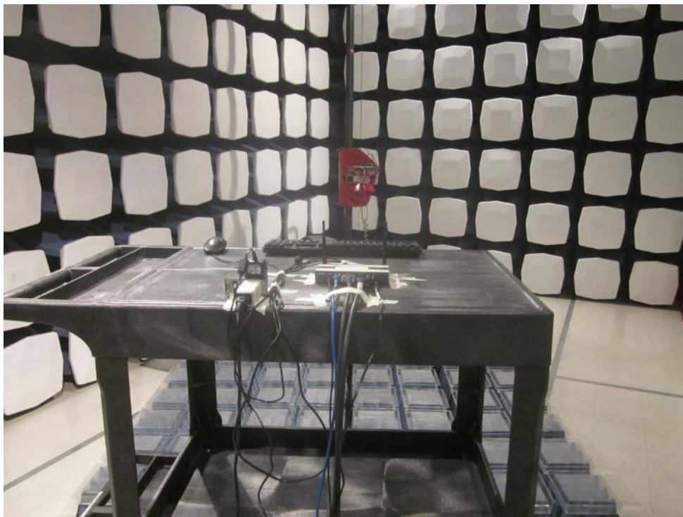
Figure B.3.2 - Radiated Emissions Test Setup - Rear View; 1 GHz-18 GHz
