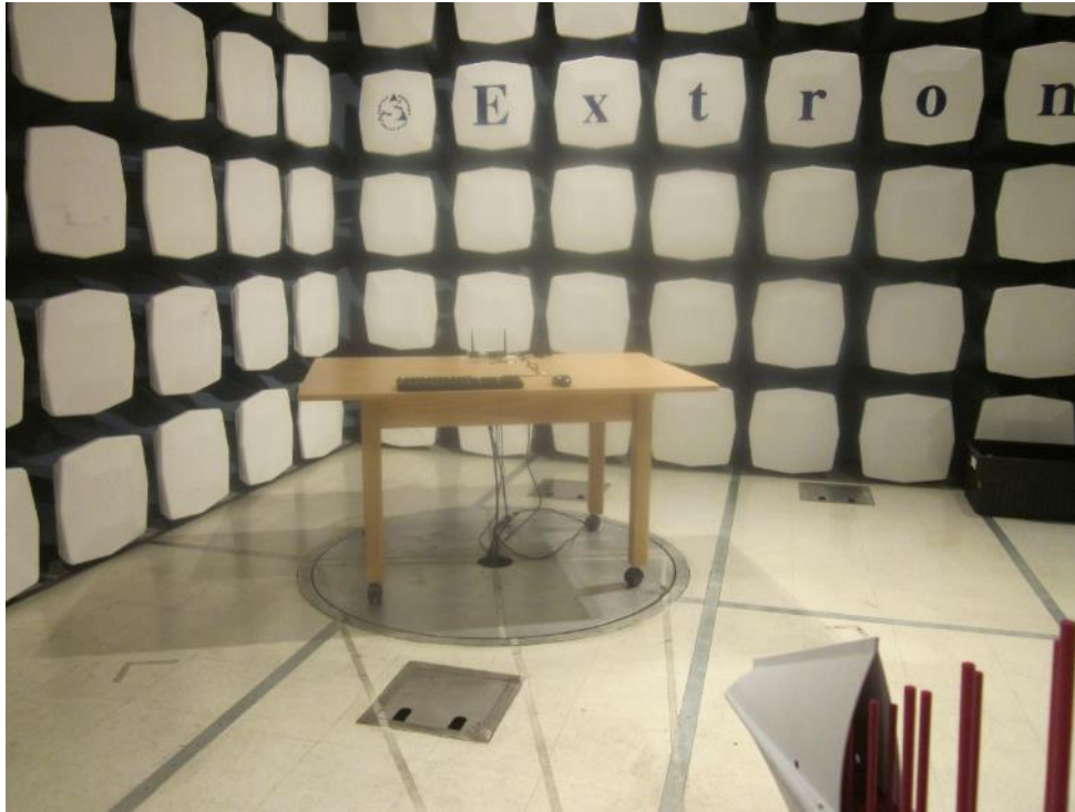
Figure B.2.1 - Radiated Emissions Test Setup - Front View; 30 MHz-1000 MHz; 5Vdc PS
