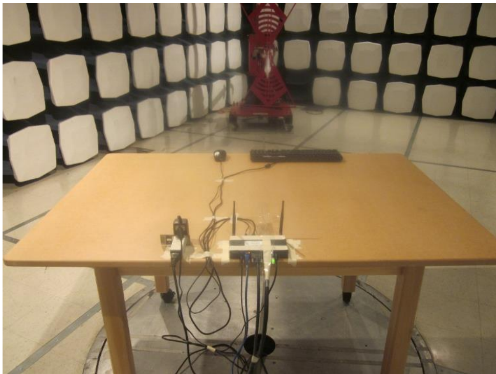
Figure B.2.2 - Radiated Emissions Test Setup - Rear View; 30 MHz-1000 MHz; 5Vdc PS
