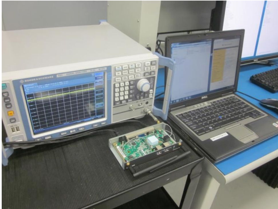
Figure B.1 – RF Conducted Measurement Test Setup 1
