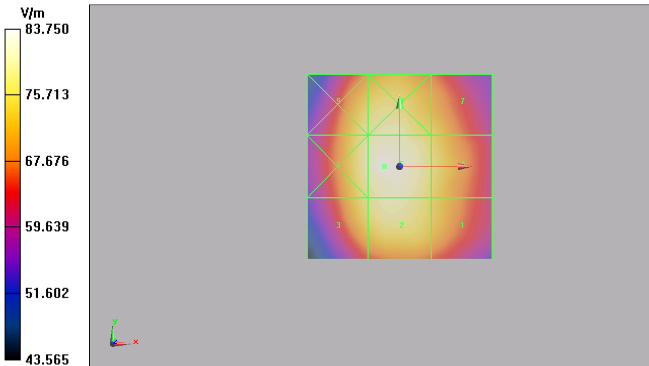
Figure 9 HAC RF E-Field GSM 850 Channel 190
