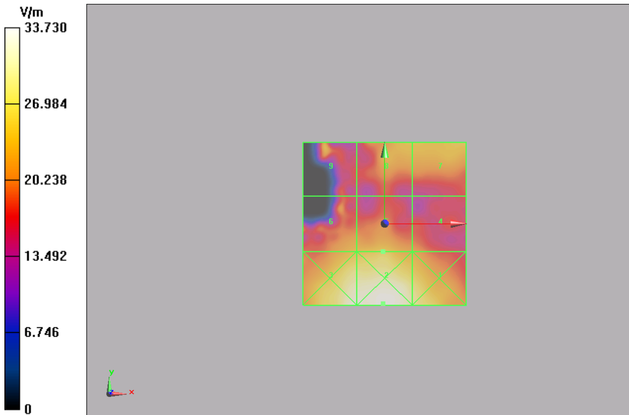
Figure 13 HAC RF E-Field GSM 1900 Channel 512
