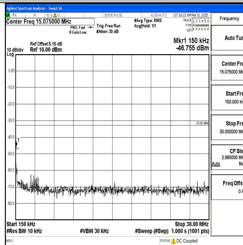
Band4_1.4MHz_QPSK_19957_1RB#0_0.15~30_0.15~30
