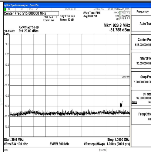
Band4 1.4MHz QPSK 19957 1RB#0 30~1000 30~1000
