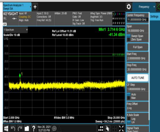
Band25-15MHz-QPSK-26115-75RB#0-Range3:2000~20000MHz
