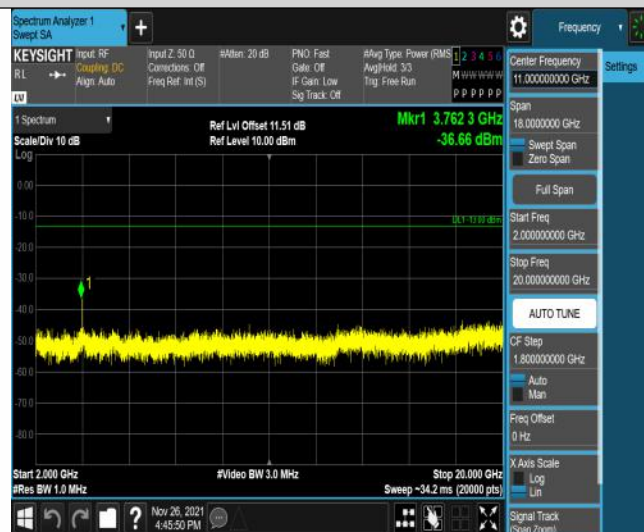
Band25-5MHz-16QAM-26365-25RB#0-Range3:2000~20000MHz
