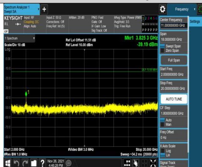
Band25-5MHz-QPSK-26665-25RB#0-Range3:2000~20000MHz
