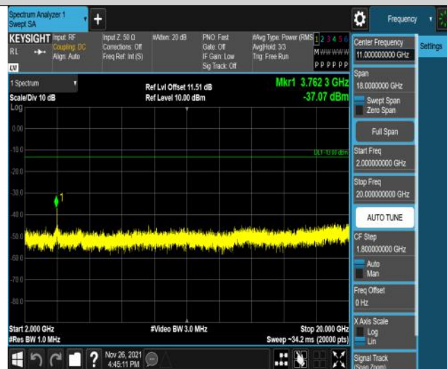
Band25-5MHz-QPSK-26365-25RB#0-Range3:2000~20000MHz
