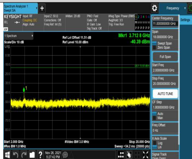
Band25-15MHz-16QAM-26115-75RB#0-Range3:2000~20000MHz
