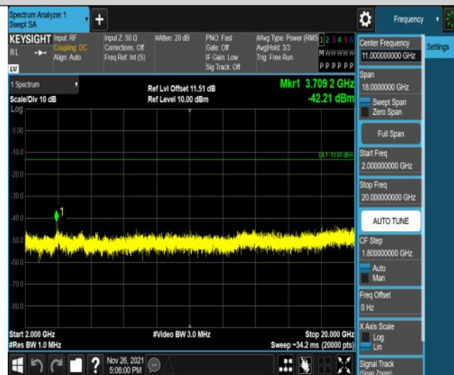
Band25-10MHz-16QAM-26090-50RB#0-Range3:2000~20000MHz
