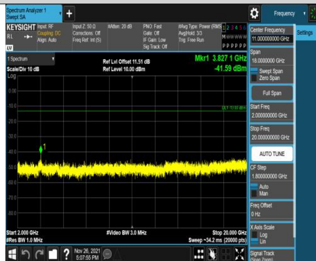
Band25-10MHz-QPSK-26640-50RB#0-Range3:2000~20000MHz
