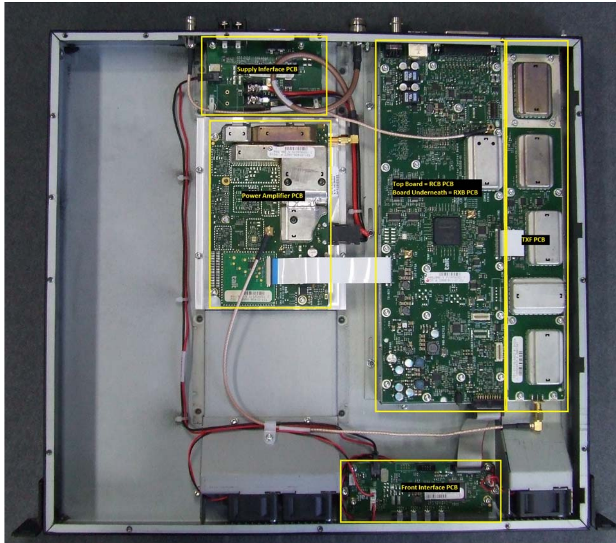
Photograph 02: Internal view – Labelled
