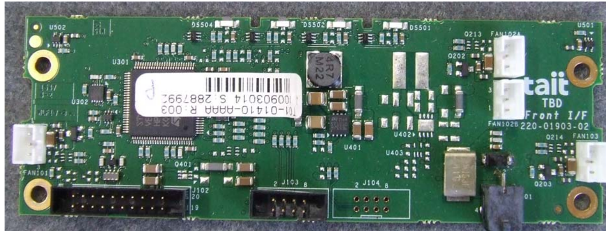
Photograph 03: Front Interface PCB - Top
