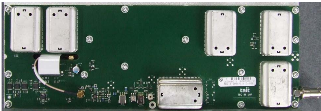
Photograph 12: Reciter Control Board (RCB) – Bottom
