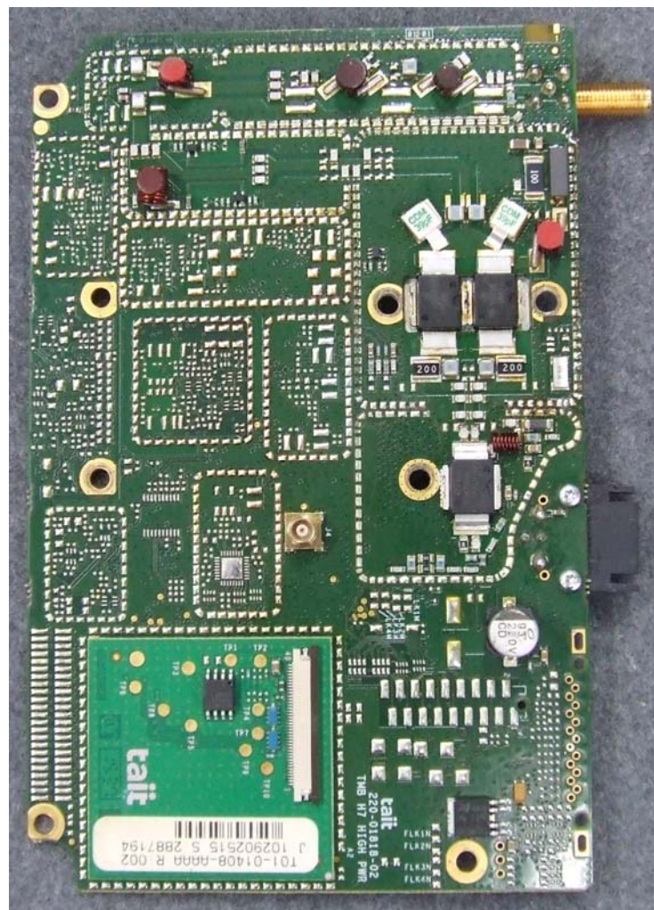
Photograph 08: Power Amplifier PCB – Top, cans off
