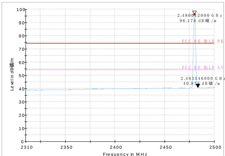
Fig.25 Bandedge:ch39
