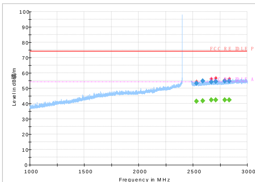
Fig.31 Radiated emission: Ch0, 1GHz~3GHz
