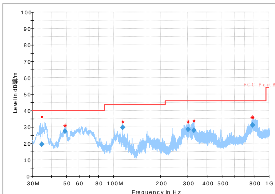
Fig.30 Radiated emission: Ch0, 30MHz~1GHz
