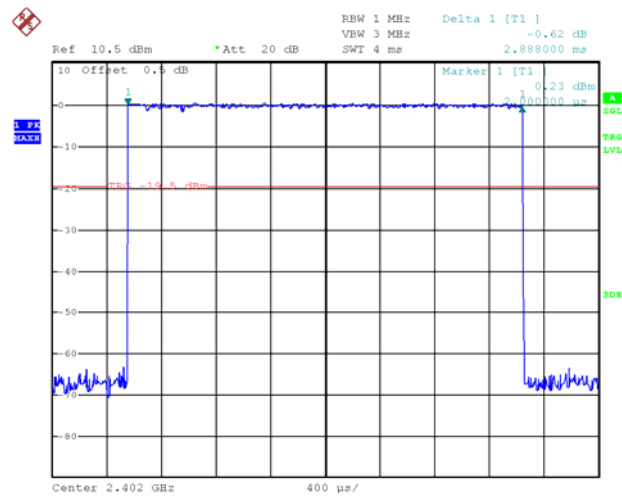
3DH5.Low channel
