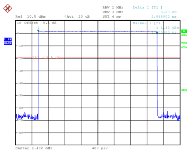
DH5.Low channel
