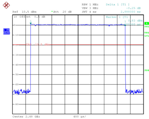
2DH5,High channel
