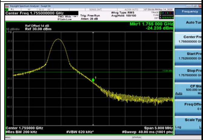
HighRange_FDD04_20MHz_1745_OneRB _high_Q16
