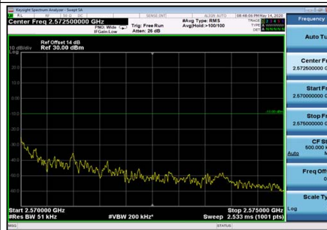
FDD07_10MHz_2565_Q16_OneRB_high _ExtraBands_Range_2570~2575
