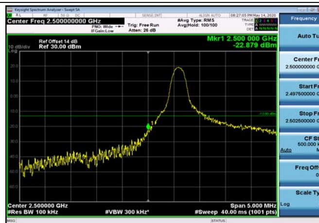
FDD07_10MHz_2505_Q16_OneRB_low
