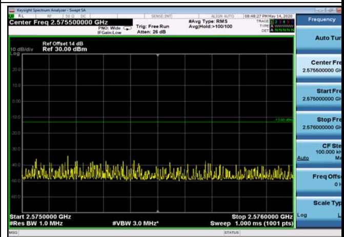
FDD07_10MHz_2565_Q16_OneRB_high _ExtraBands_Range_2575~2576
