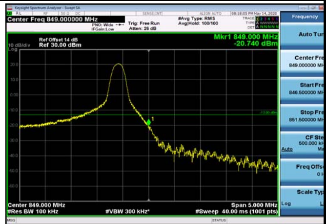
HighRange_FDD05_10MHz_844_fullIRB _High_Q16
