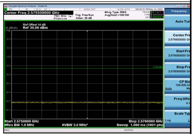
FDD07_5MHz_2502.5_QPSK_OneRB_high _ExtraBands_Range_2575~2576
