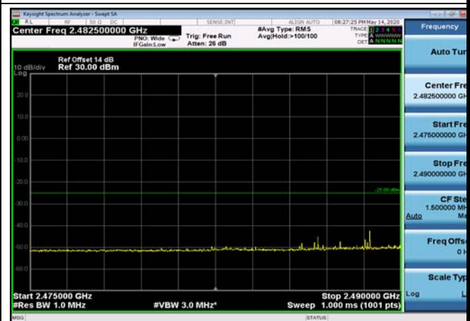
LowRange_FDD07_10MHz_2505_fullRB
