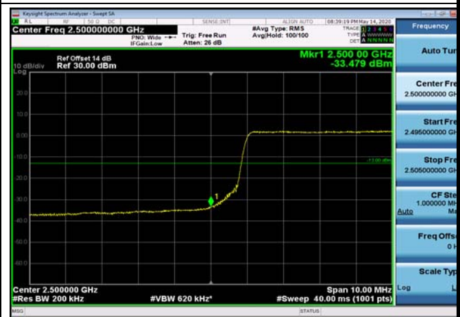
LowRange_FDD07_20MHz_2510_fullRB _Low_QPSK
