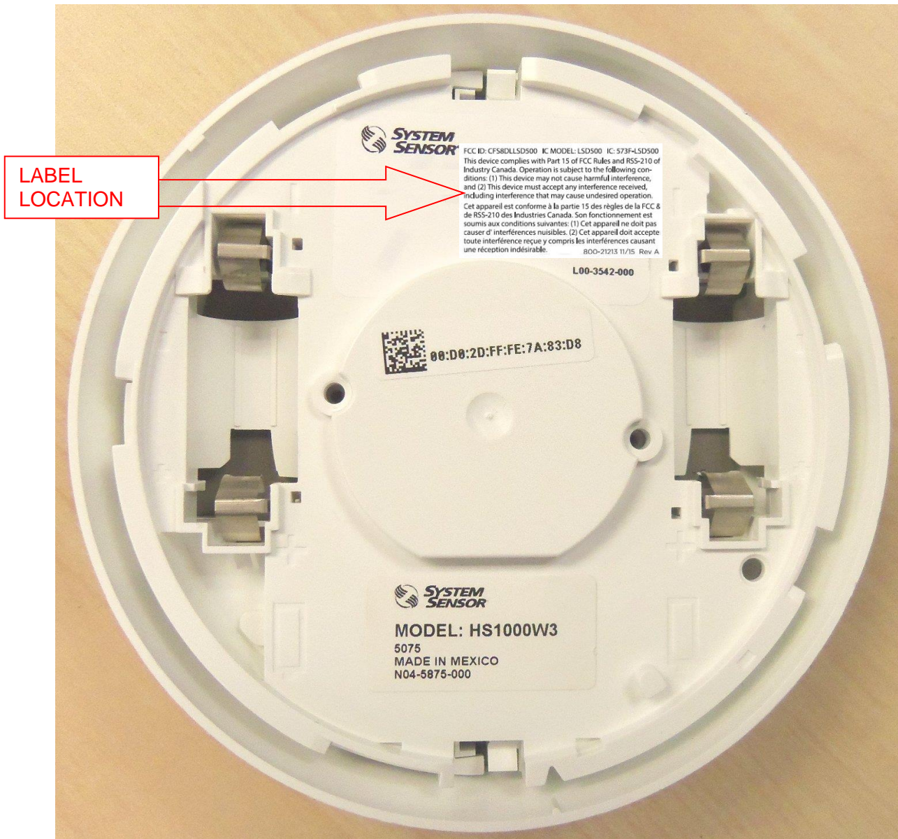
Case Back, Mounting Plate Removed
