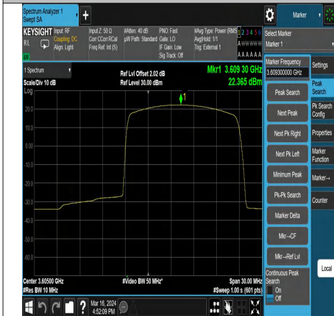
43(3600-3700)-10MHz-QPSK-43640-1RB#49-PASS
