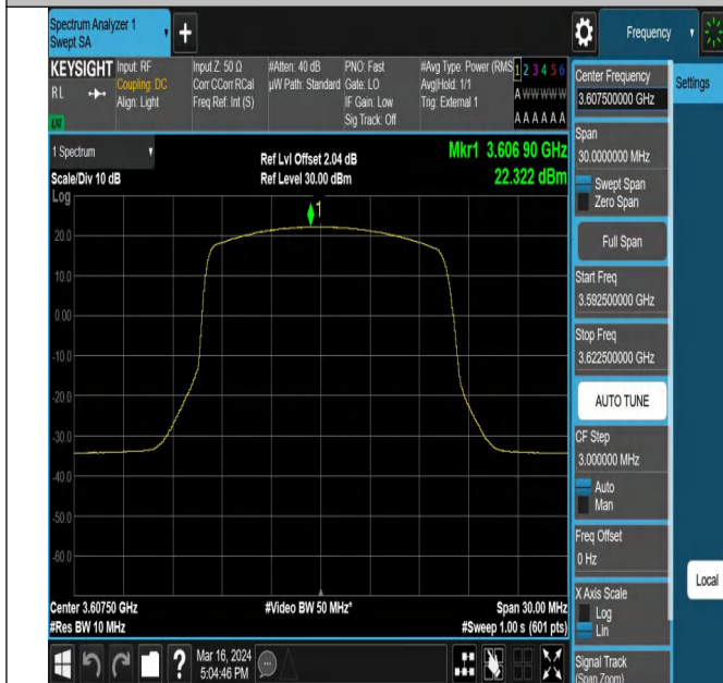
43(3600-3700)-15MHz-QPSK-43665-1RB#38-PASS
