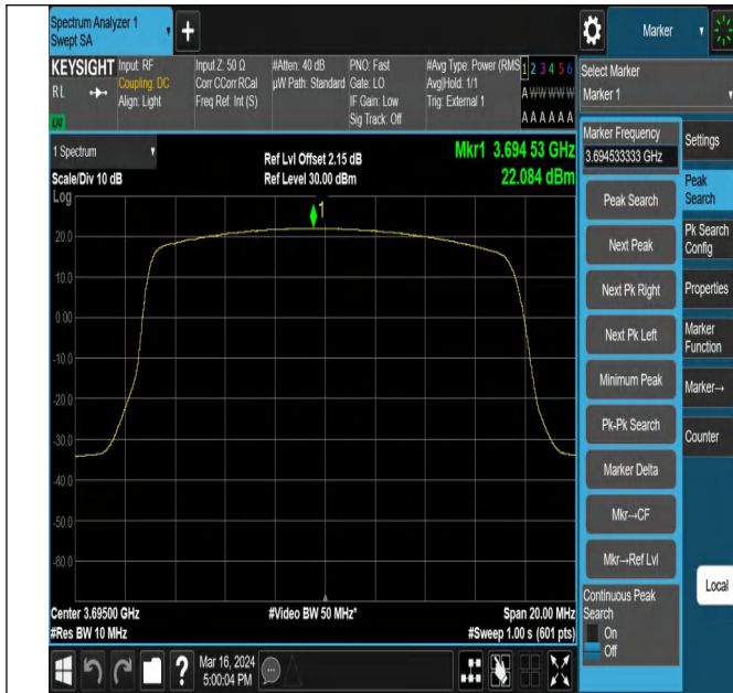
43(3600-3700)-10MHz-QPSK-44540-1RB#24-PASS
