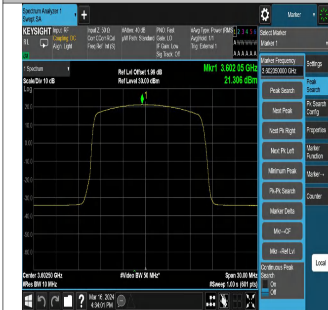
43(3600-3700)-5MHz-16QAM-43615-1RB#12-PASS
