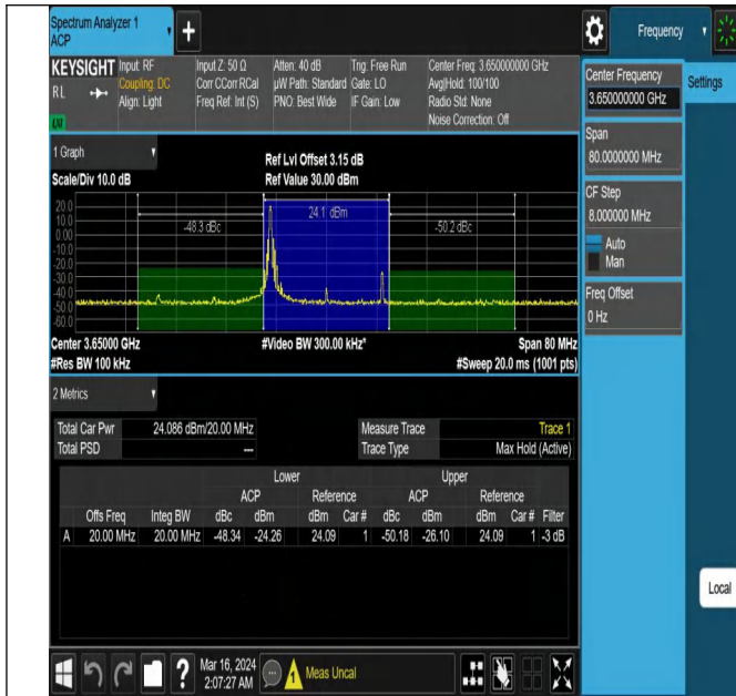
43(3600-3700)-20MHz-QPSK-44090-1RB#0-PASS
