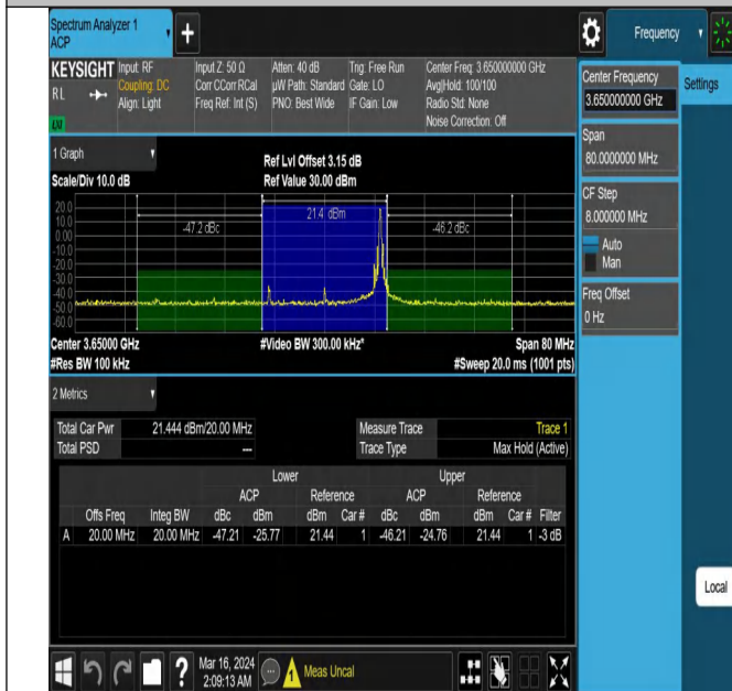
43(3600-3700)-20MHz-QPSK-44090-1RB#99-PASS
