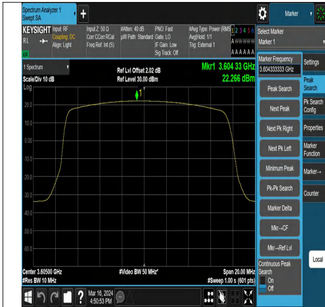
43(3600-3700)-10MHz-QPSK-43640-1RB#24-PASS
