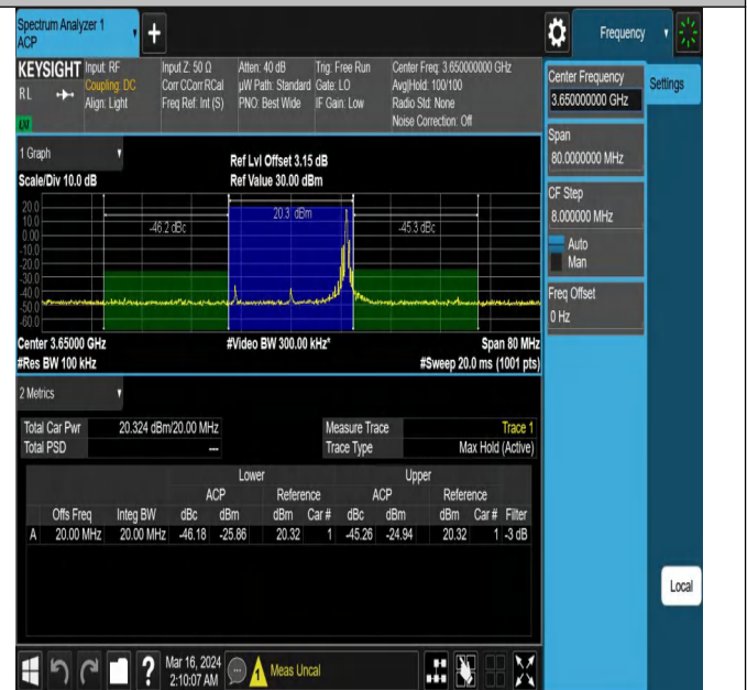
43(3600-3700)-20MHz-16QAM-44090-1RB#99-PASS
