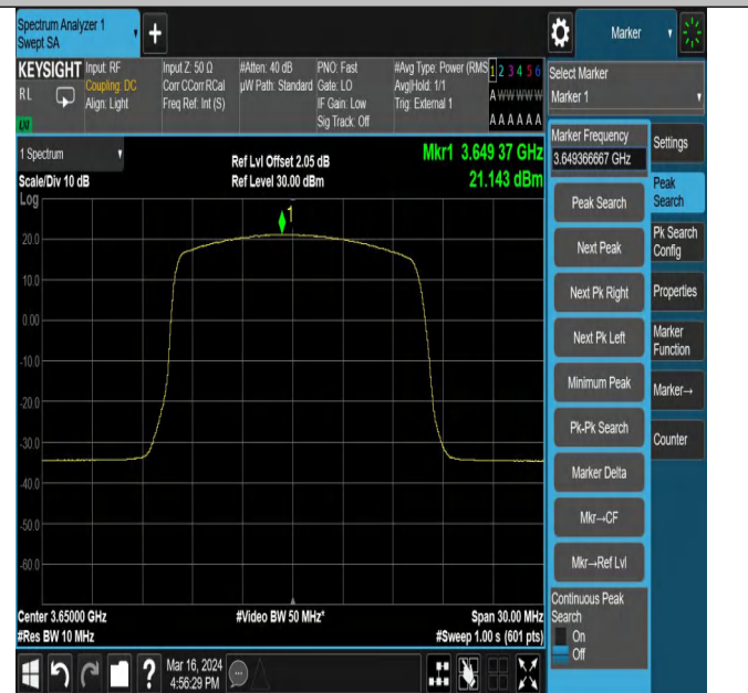
43(3600-3700)-10MHz-16QAM-44090-1RB#24-PASS
