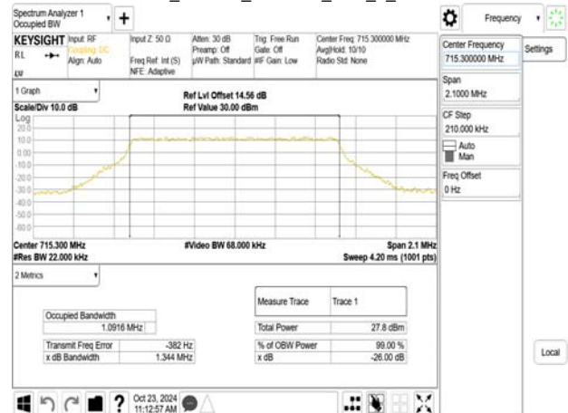
Band12_1.4MHz_256QAM_RB6_0_CH23173
