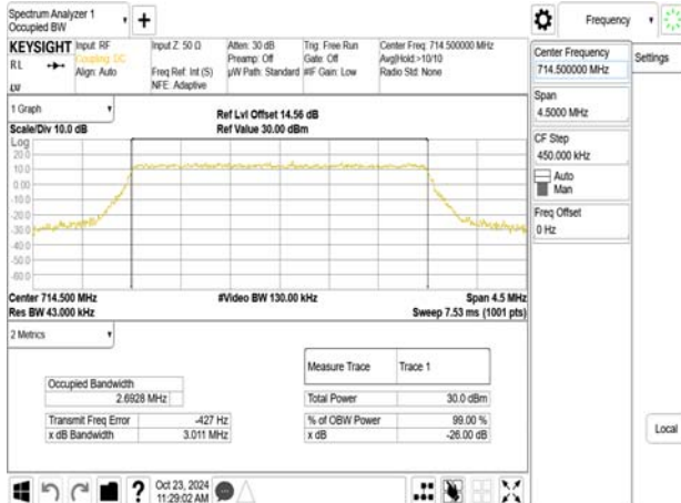
Band12_3MHz_64QAM_RB15_0_CH23165
