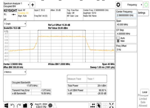
Band7_20MHz_256QAM_RB100_0_CH21350
