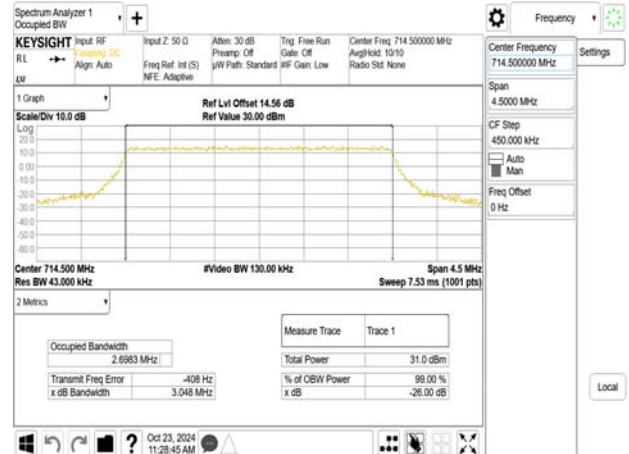
Band12_3MHz_16QAM_RB15_0_CH23165
