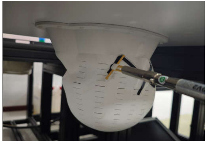
2.4GHz Dipole Placed at Location C in 90° Orientation (10mm Spacer)
