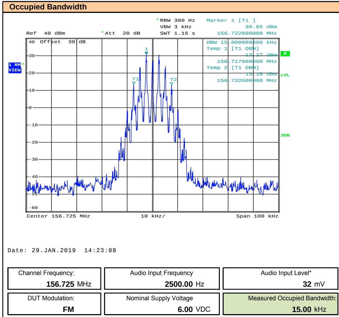
Plot 10.2 – Occupied Bandwidth Channel 74
