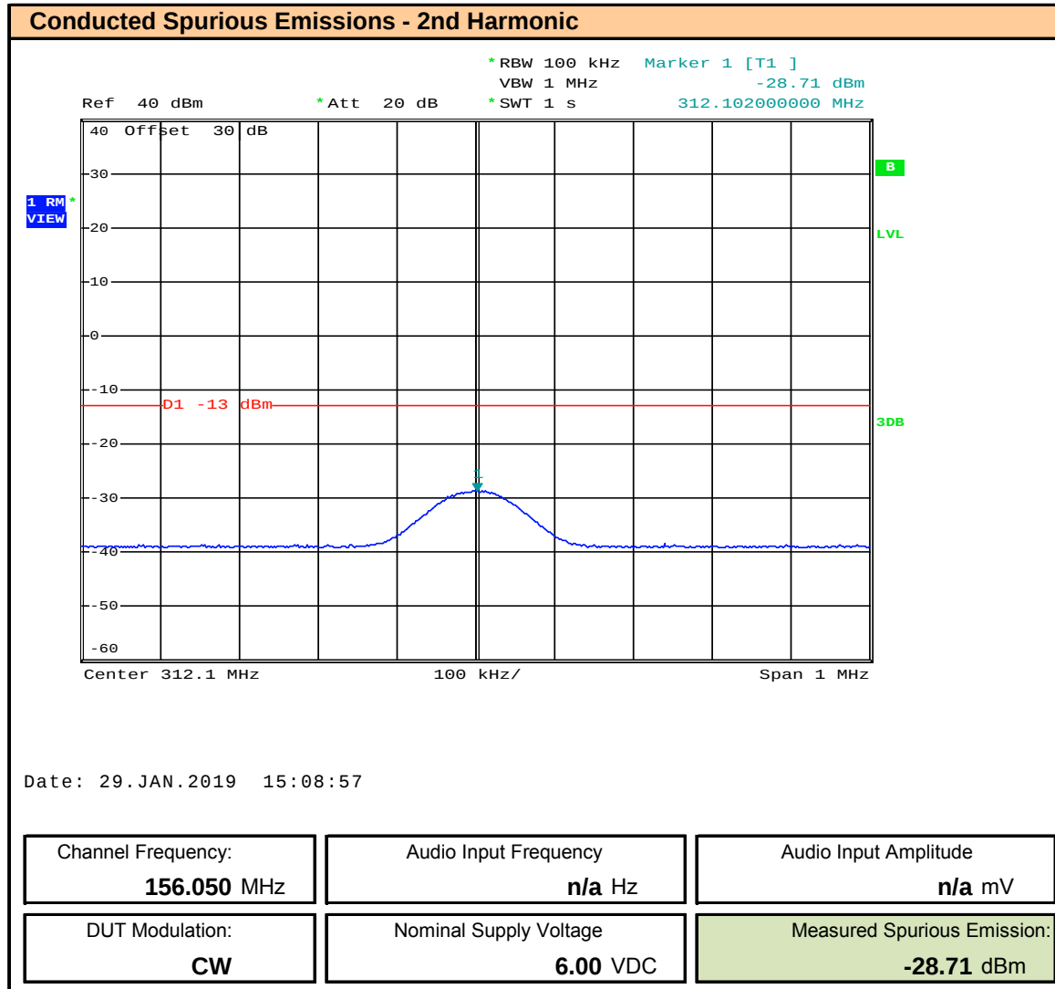
Plot 11.2 – Conducted Out of Band Emissions, Channel 1, 2 nd Harmonic
