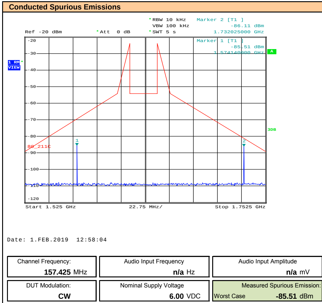
Plot 12.2 – Conducted Out of Band Emissions, Restricted Band, Channel 88
