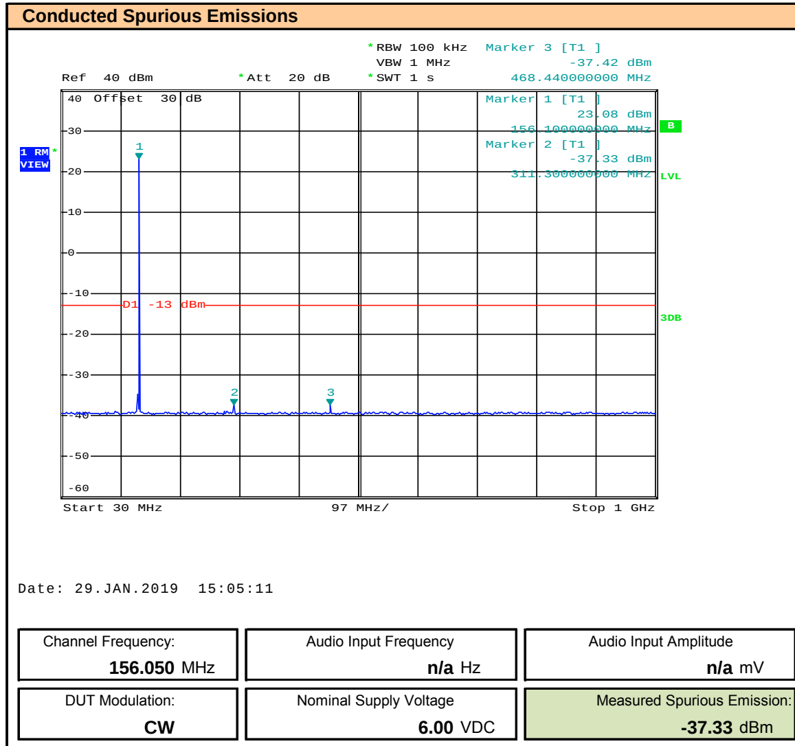
Plot 11.1 – Conducted Out of Band Emissions, 30MHz – 1000MHz, Channel 1
