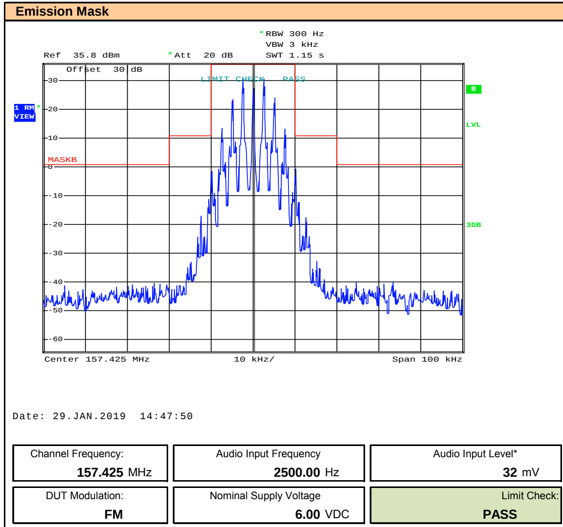
Plot 10.6 – Emission Mask Channel 88
