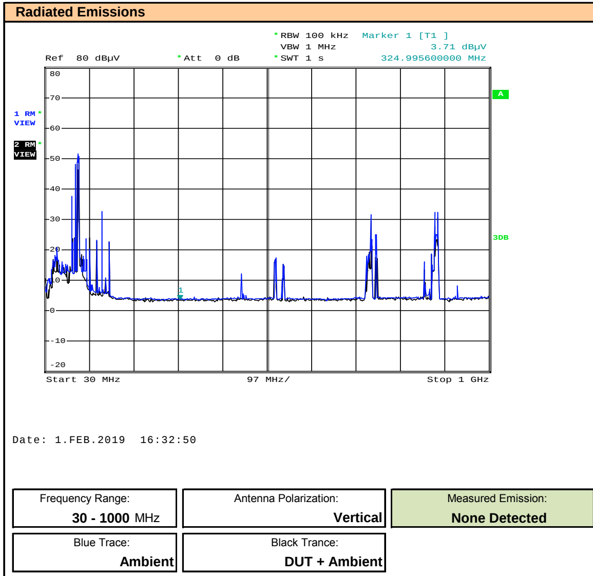
Plot 13.2 – Radiated Spurious Emissions OATS, 30MHz – 1000MHz, Vertical
