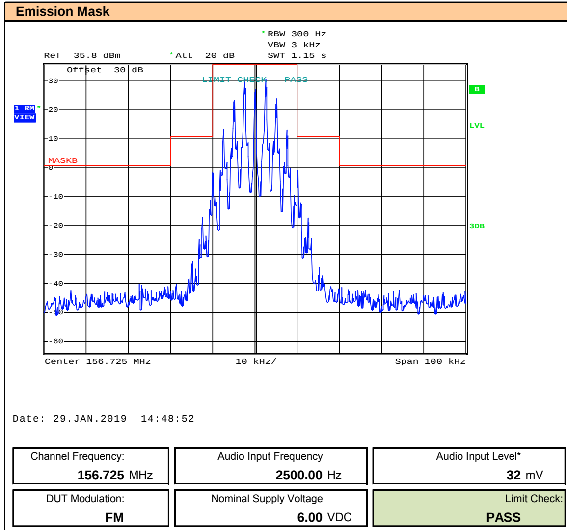
Plot 10.5 – Emission Mask Channel 74
