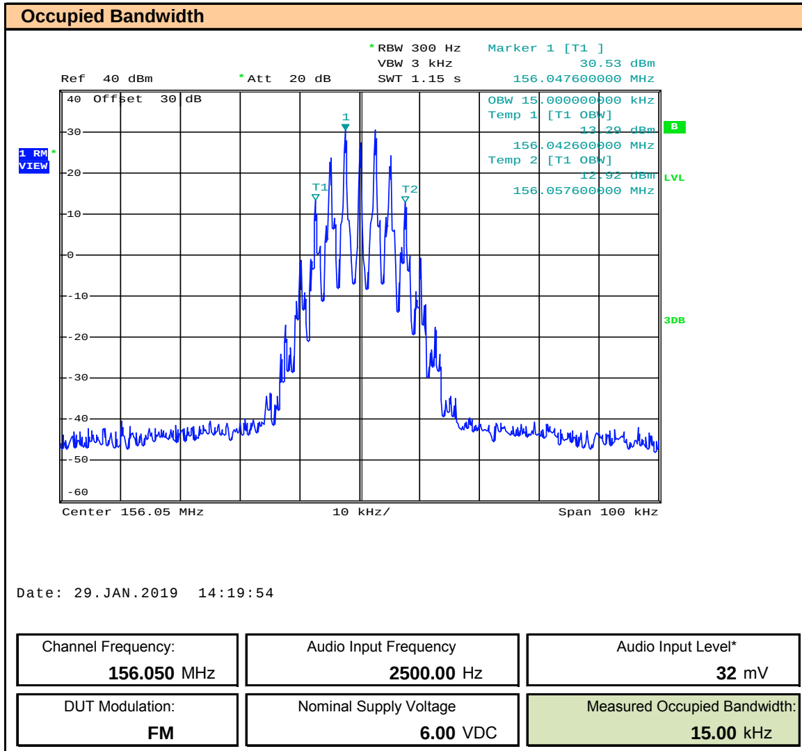
Plot 10.1 – Occupied Bandwidth Channel 1
