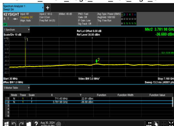
N12(5M)_DFT-s- OFDM_BPSK_Edge_1RB_Left_High_CH
