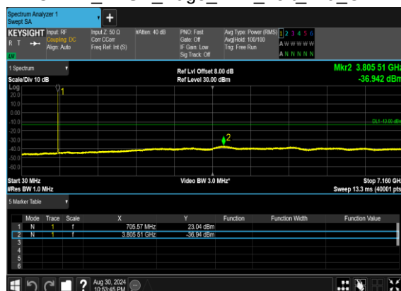
N12(5M)_DFT-s- OFDM_BPSK_Edge_1RB_Left_Mid_CH
