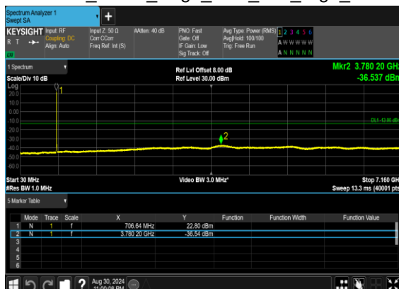
N12(10M)_DFT-s- OFDM_BPSK_Edge_1RB_Left_High_CH
