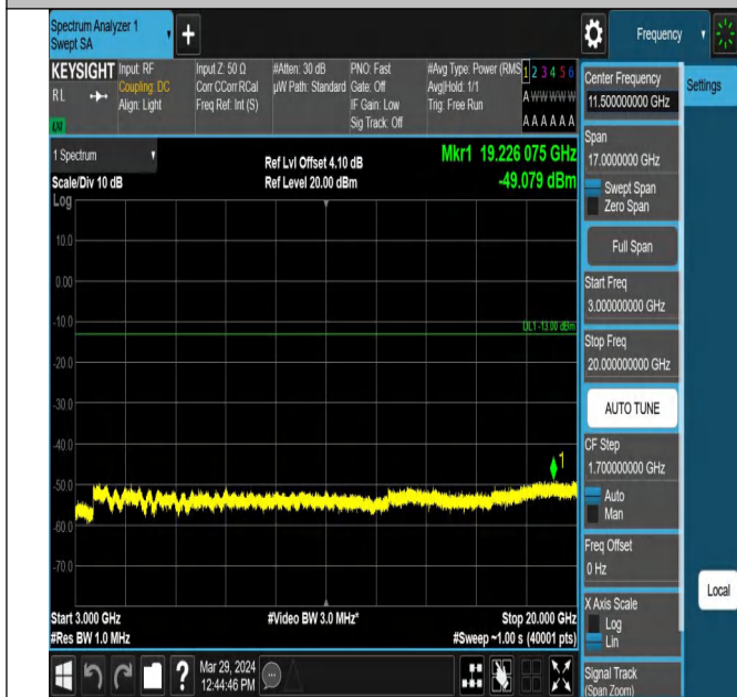
Band2_1.4MHz_QPSK_19193_1RB#0_3000~20000_3000~20000
