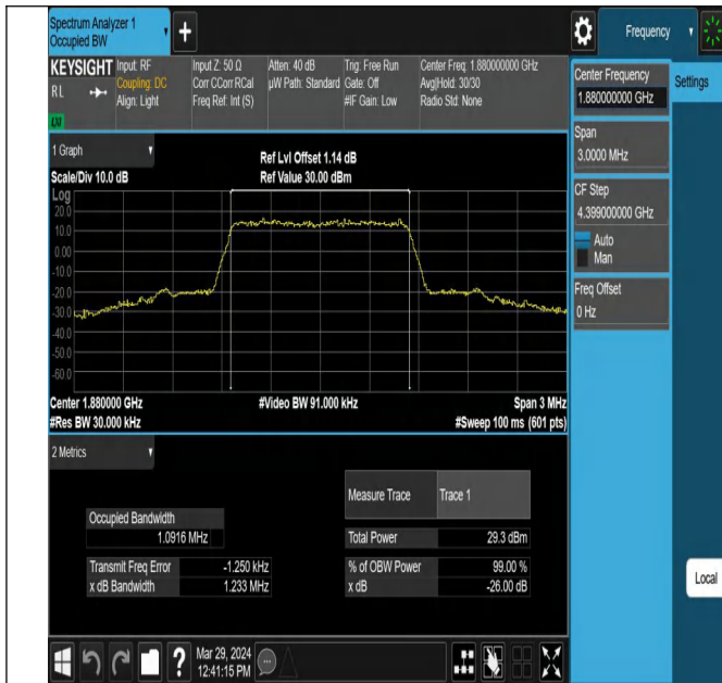
Band2-1.4MHz-QPSK-18900-6RB#0-PASS
