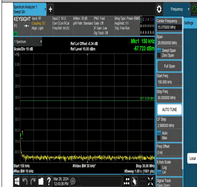
Band2_1.4MHz_QPSK_18900_1RB#0_0.15~30_0.15~30
