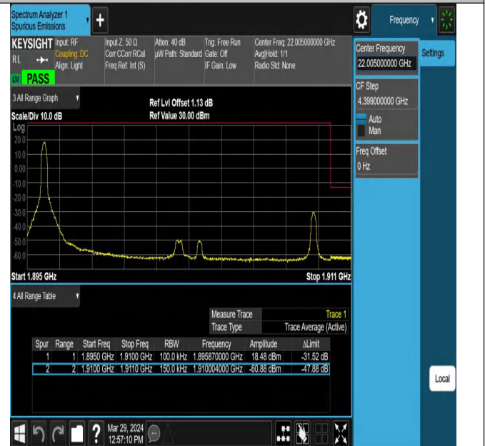
Band2_15MHz_QPSK_19125_1RB#0
