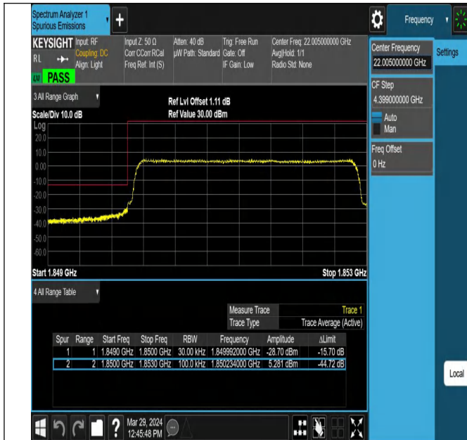
Band2_3MHz_QPSK_18615_15RB#0
