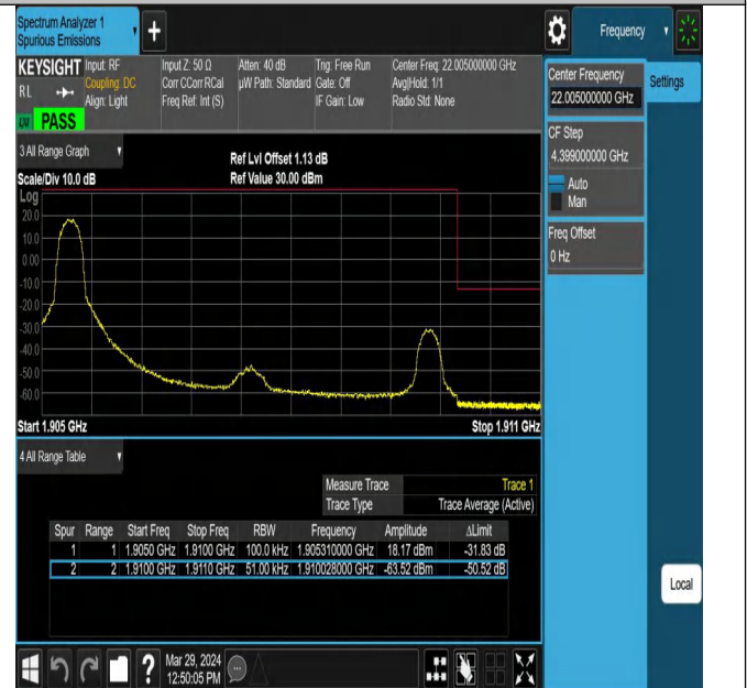
Band2_5MHz_QPSK_19175_1RB#0
