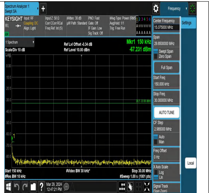
Band2_3MHz_QPSK_18900_1RB#0_0.15~30_0.15~30
