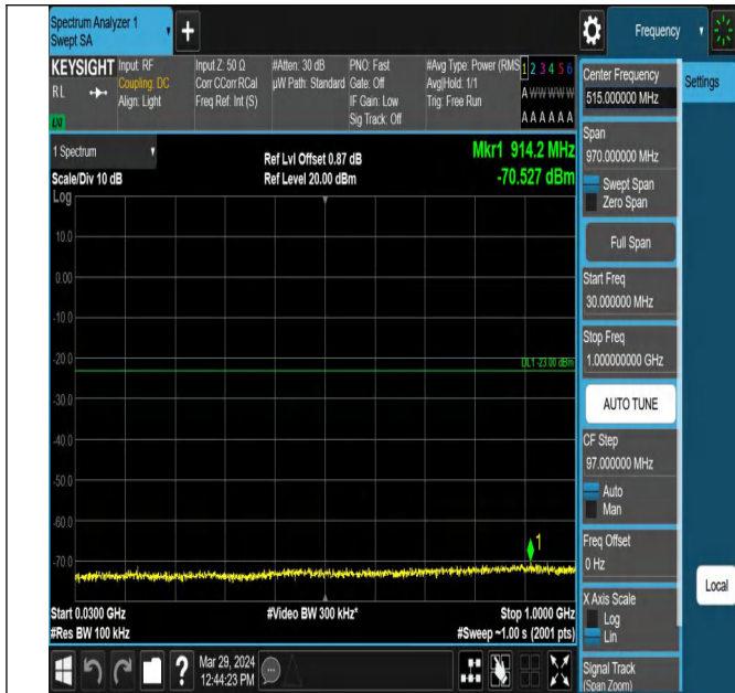
Band2_1.4MHz_QPSK_19193_1RB#0_30~1000_30~1000
