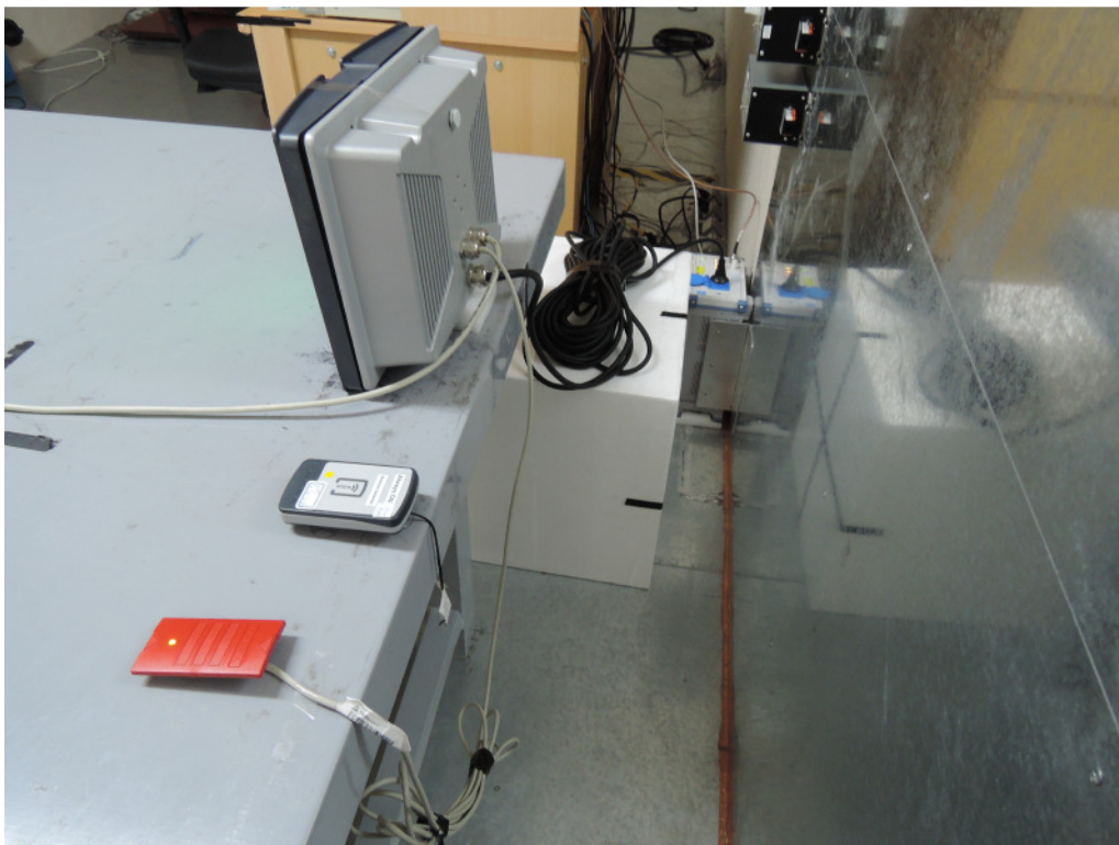
Photograph 5: Set-up for for Mains Conducted testing Front
