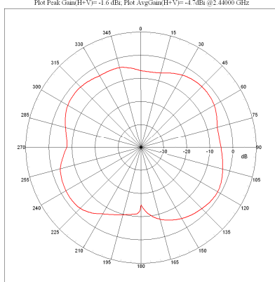
Far-field Power Distribution(H+V) on Y-Z Plane Plot Peak Gain(H+V)=-1.6 dB, Plot AvgGain(H+V)=-4.7dB @2.44000 GHz
