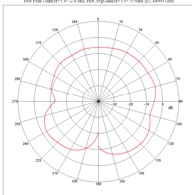
Far-field Power Distribution(H+V) on X-Z Plane Plot Peak Gain(H+V)=-2.8 dB, Plot AvgGain(H+V)=-5.9dB @2.44000 GHz
