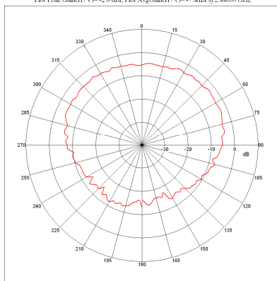
Far-field Power Distribution(H+V) on X-Y Plane Plot Peak Gain(H+V)=-2.6 dB, Plot AvgGain(H+V)=-7.4dB @2.44000 GHz
