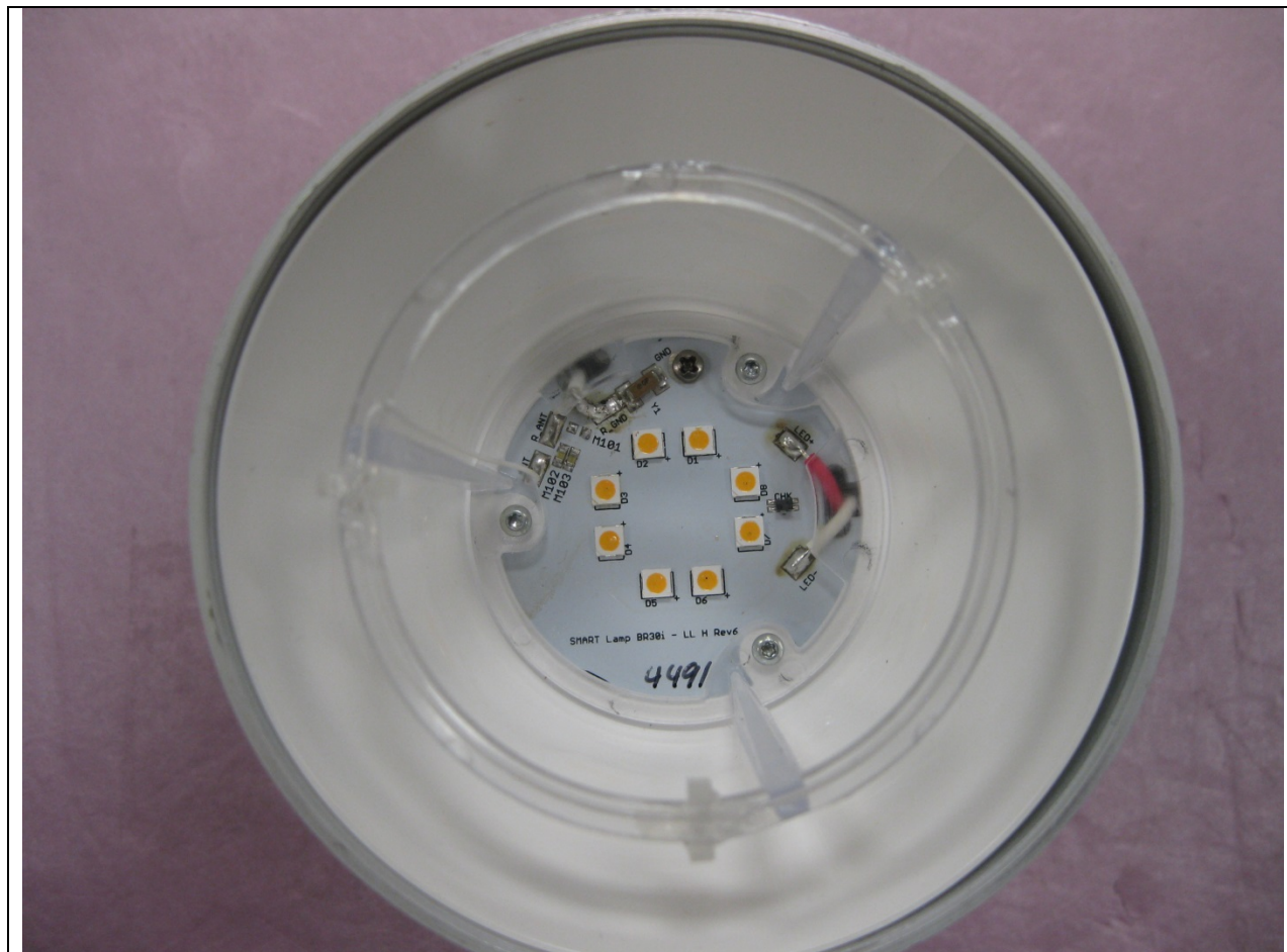
Top of Fixture with Bulb Dome Removed
