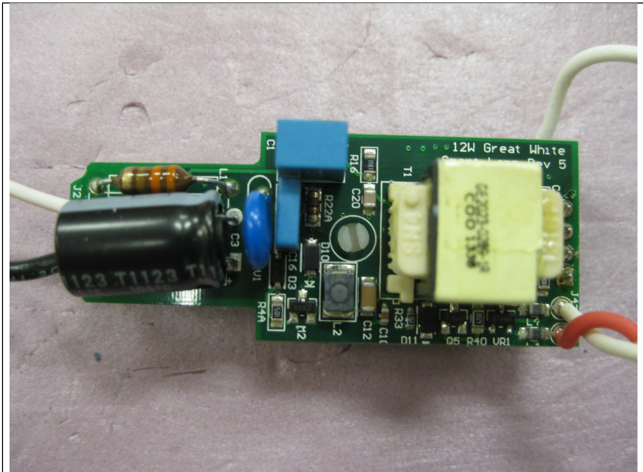
Power Supply Circuit Board - Top
