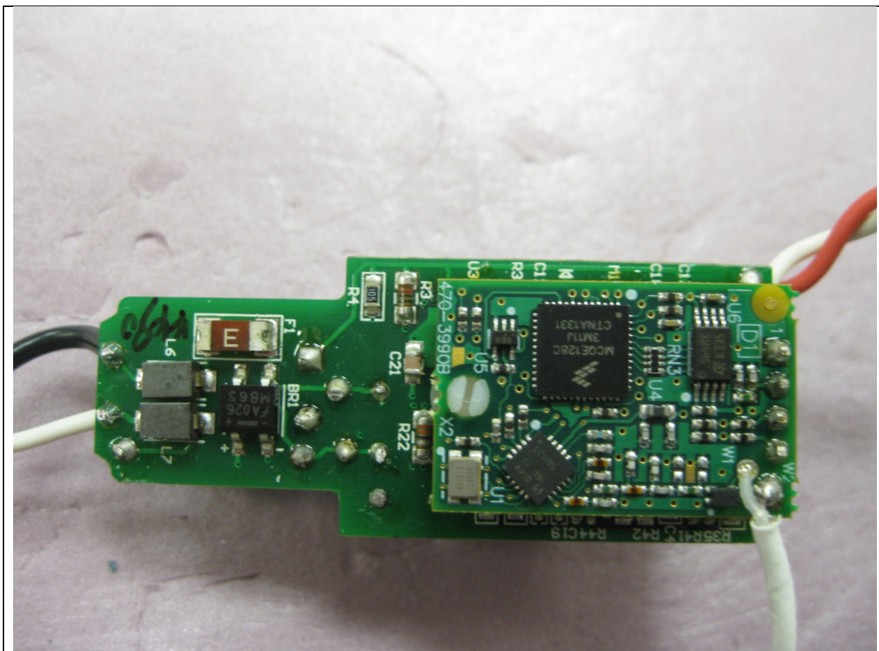
Power Supply Circuit Board – Bottom (Daughter card is Radio Board, installed)
