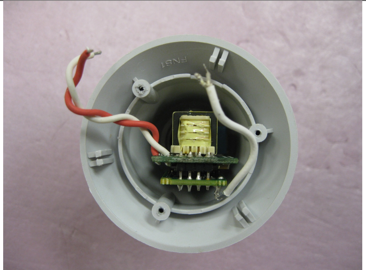
Upper Half Removed – Radio Circuit and Power Supply Circuit
